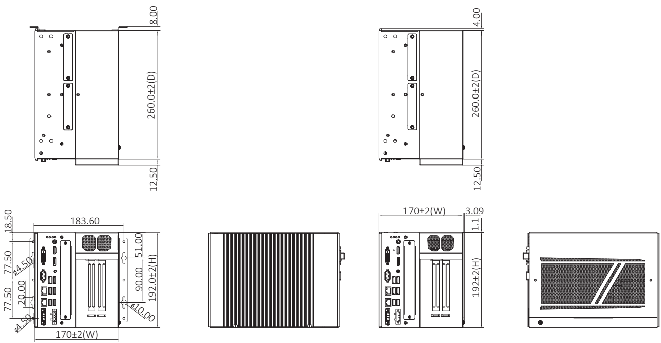
Wall mount (optional)
