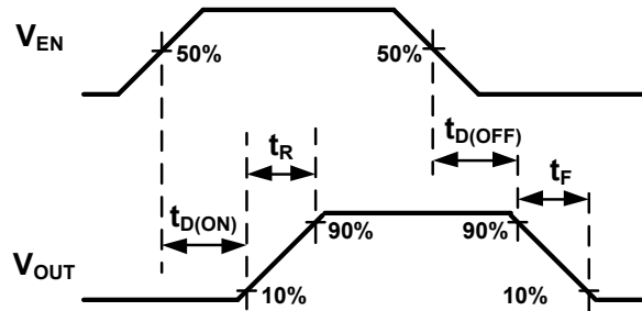
Figure 1. Voltage Waveform
