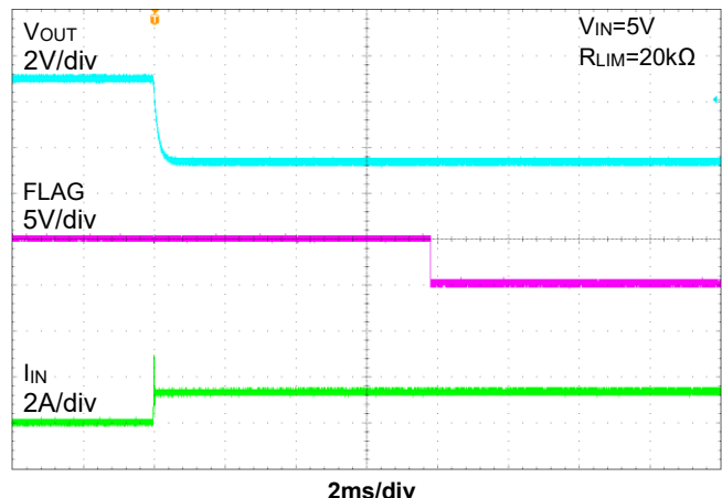
Figure 5. No Load to 1 \Omega Transient Response
