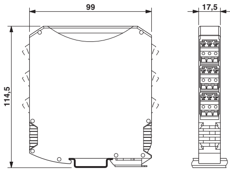
Figure 1 Dimensions
