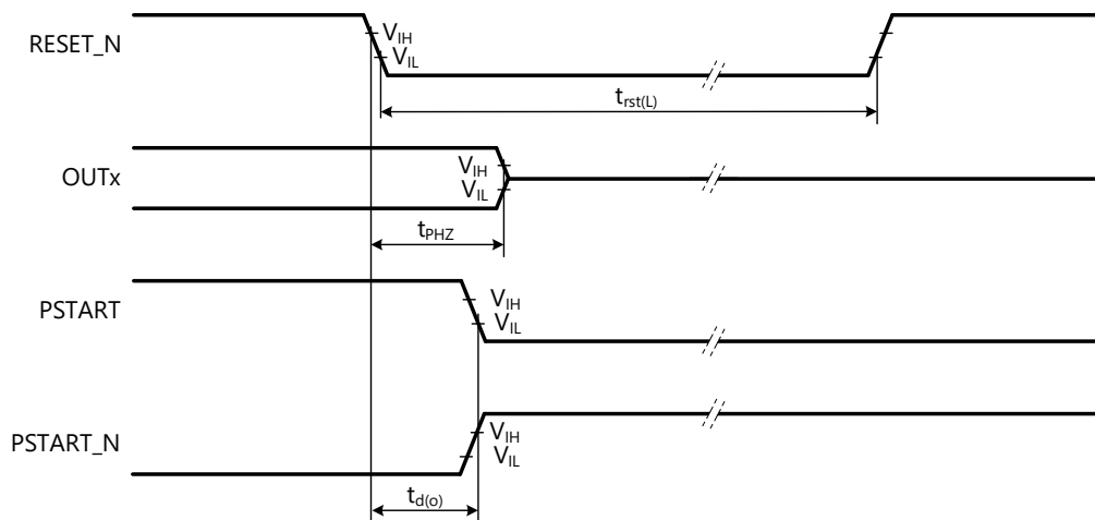
Figure 8. RESET_N Timing
