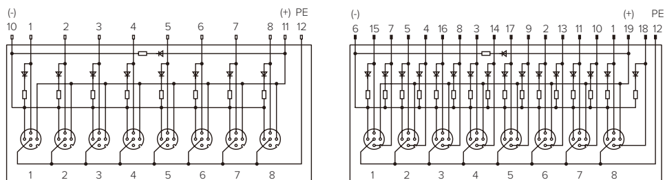
Wiring Diagram
