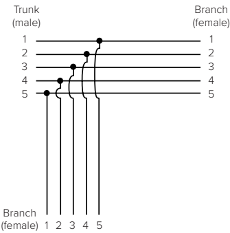
Example of 4-Pin Wiring
