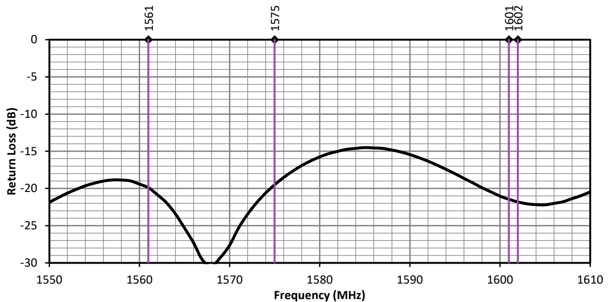
Figure 4. ANT-GNRM-L1A Series Antenna Return Loss, L1 Band
