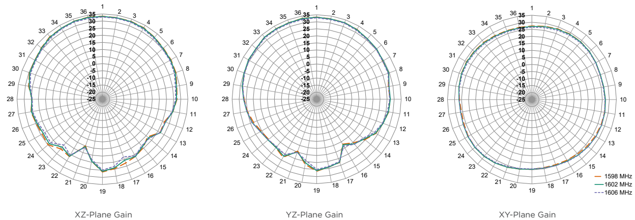
Figure 7. ANT-GNRM-L1A Radiation Patterns
