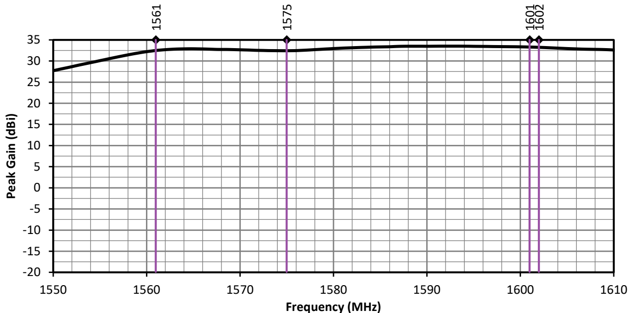
Figure 5. ANT-GNRM-L1A Series Antenna Peak Gain, L1 Band
