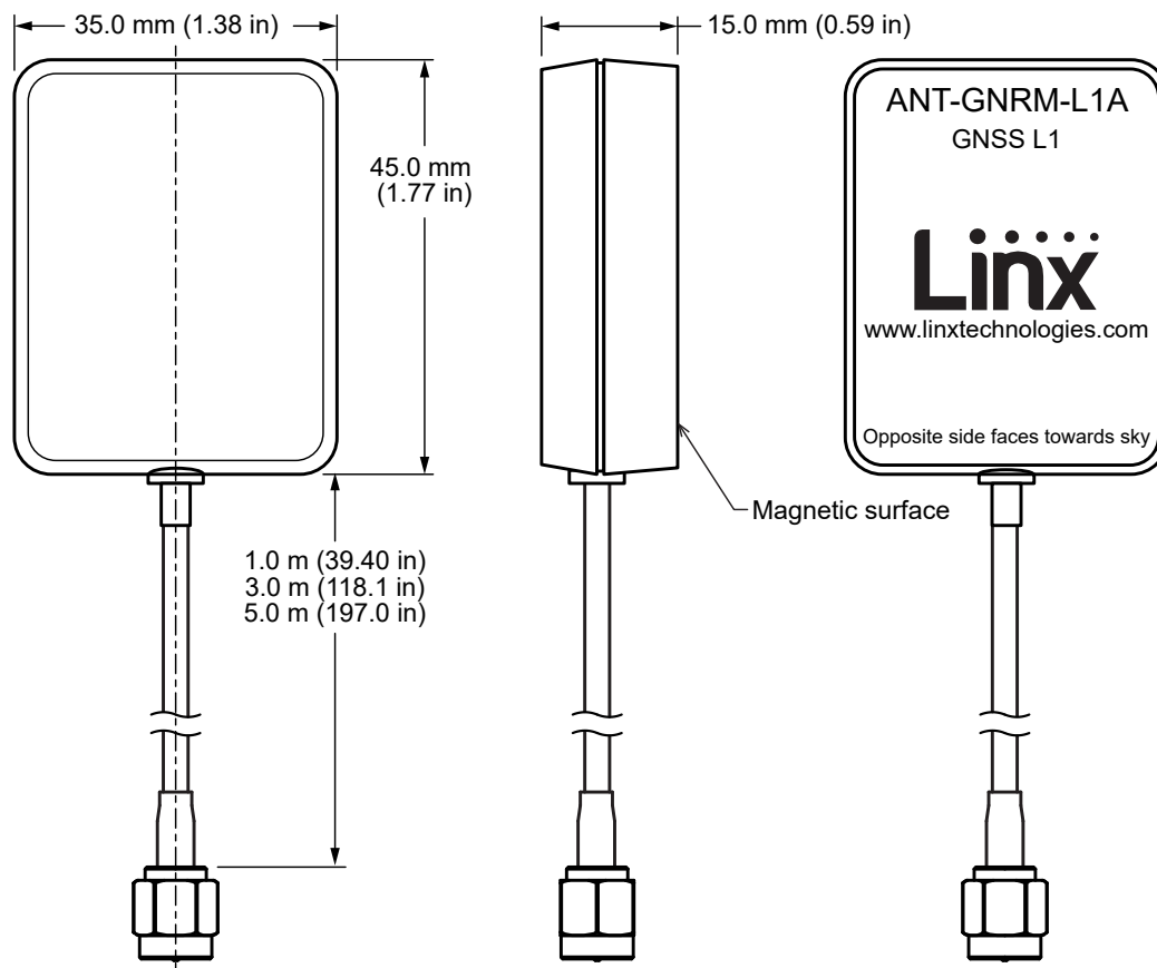
Figure 1. ANT-GNRM-L1A Series Antenna Dimensions
