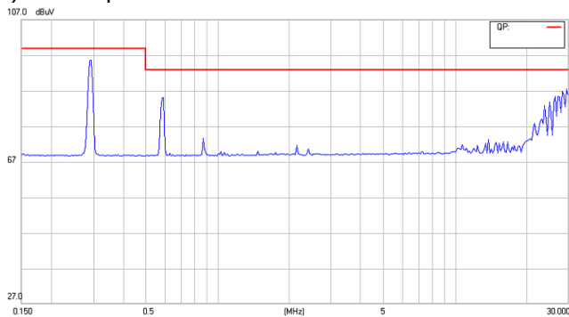
CQB150W-110S24 Positive
