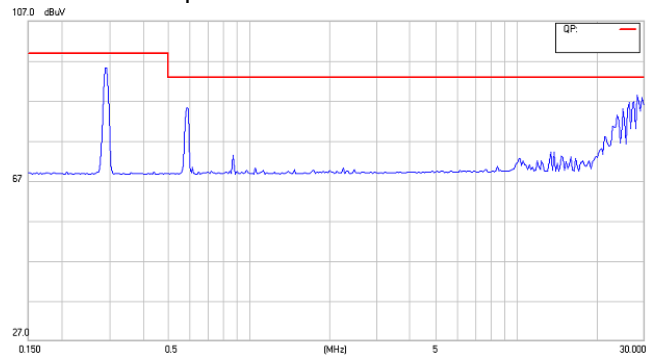
CQB150W-110S24 Negative
