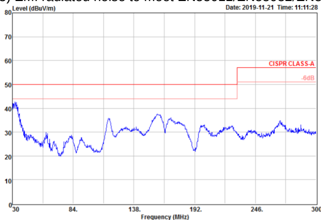
Radiated EN55032 Class A of CQB150W-110S24 Vertical
