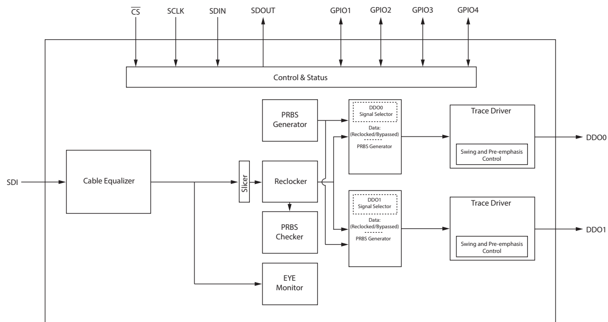
GS12341 Functional Block Diagram
