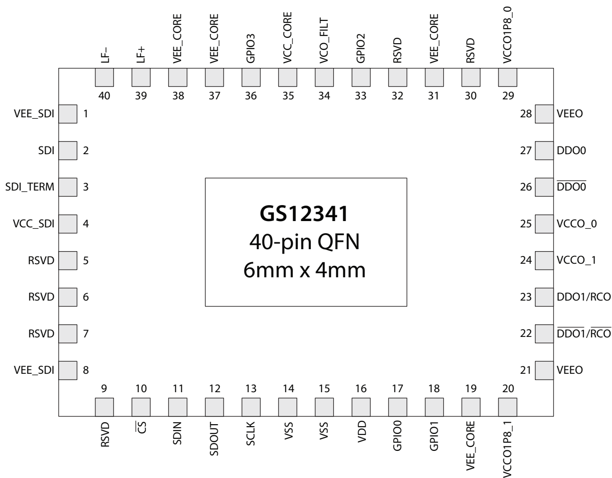
Figure 1-1: GS12341 Pin Assignment
