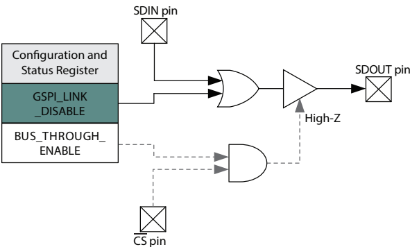
Figure 4-20: GSPI_LINK_DISABLE Operation
