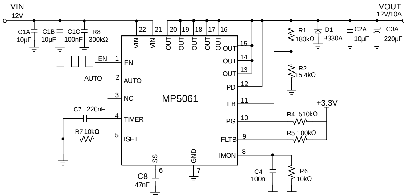
Figure 7: Typical Application Circuit with 10ms Soft-Start Time, 12A Current Limit
