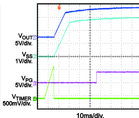
Start-Up Sequence
