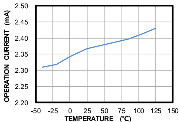
Operation Current vs. Temperature
