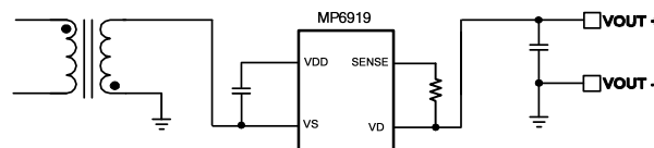
Figure 4: High-Side Rectification
