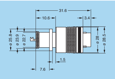
FM.LM.U2A.XPAT Straight plug, key (W) or key (R) with knurled grip and mold stop
