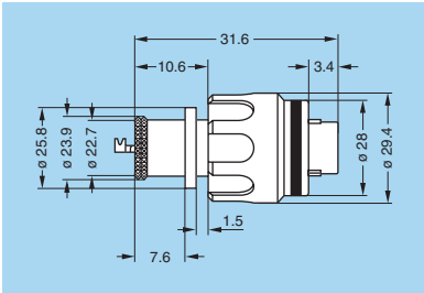
FG.LM.U2A.XPAT Straight plug, key (W) or key (R) with arctic grip and mold stop
