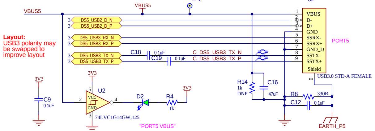
USB3.1(Type-A) Downstream Port 5
