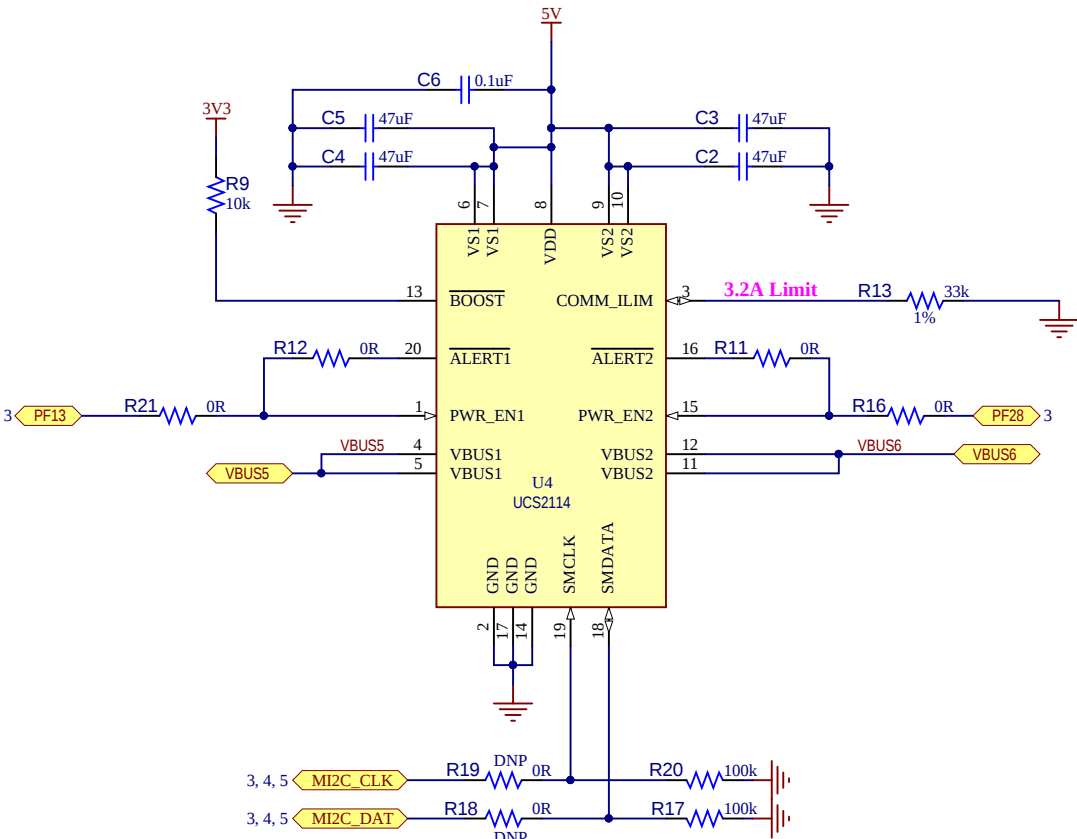
UCS2114 Power Switch For Port5 and Port6
