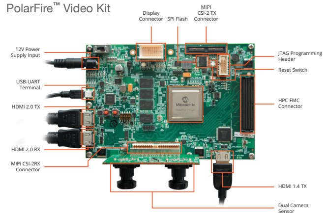
PolarFire™ Video Kit
