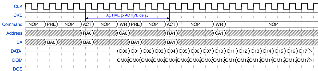
Figure 25-15. AXI Command - Pipelined SDRAM Write
