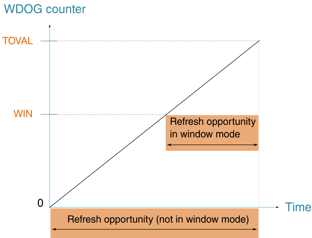
Figure 53-2. Refresh opportunity for the Watchdog counter
