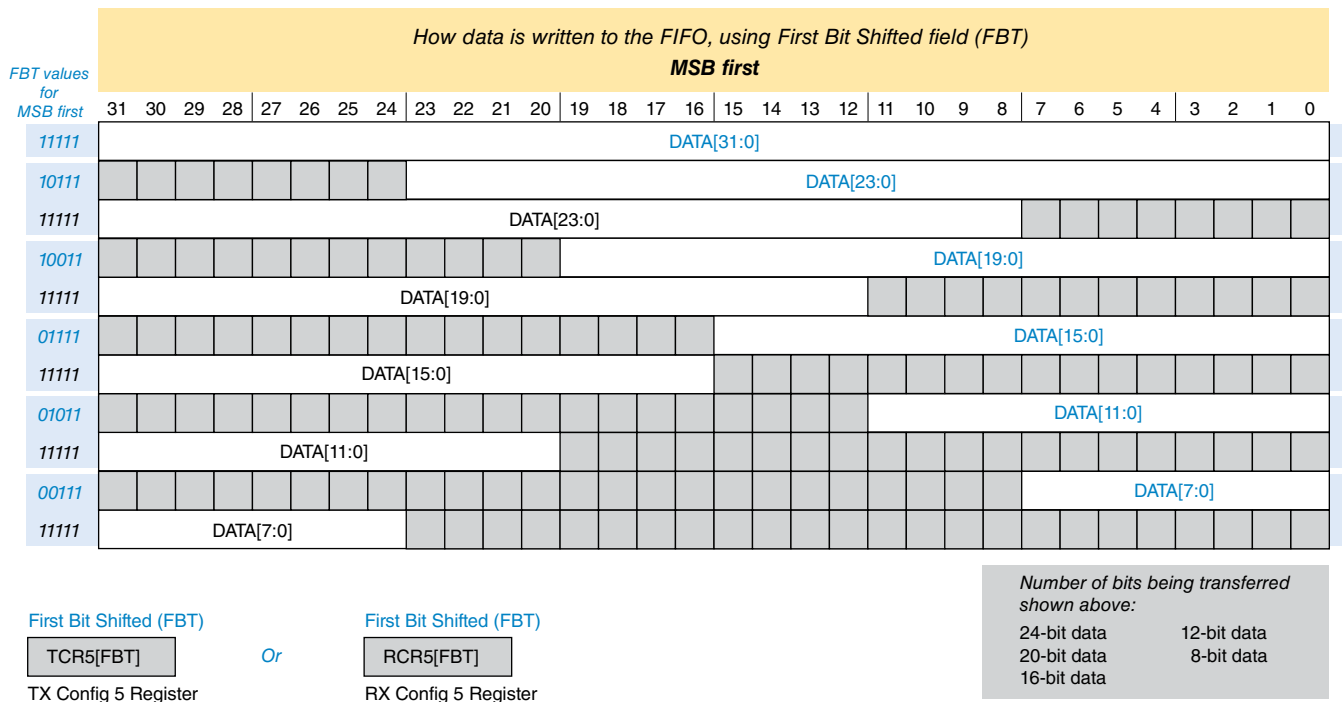
Figure 34-3. SAI first bit shifted, MSB first
