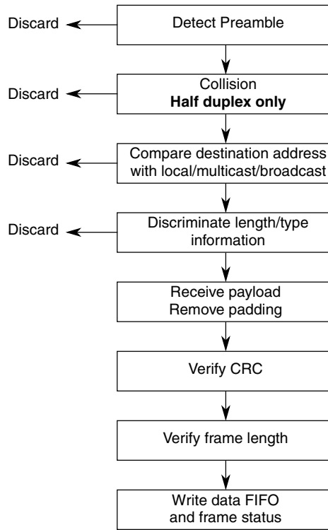
Figure 37-5. MAC receive flow
