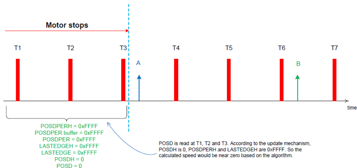
Figure 51-7. Speed measurement at time point T1~T3
