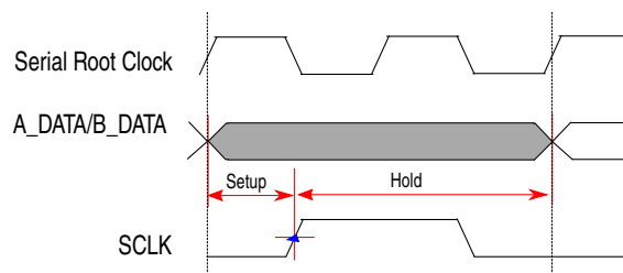
Figure 27-20. SDR instruction in DDR sequence
