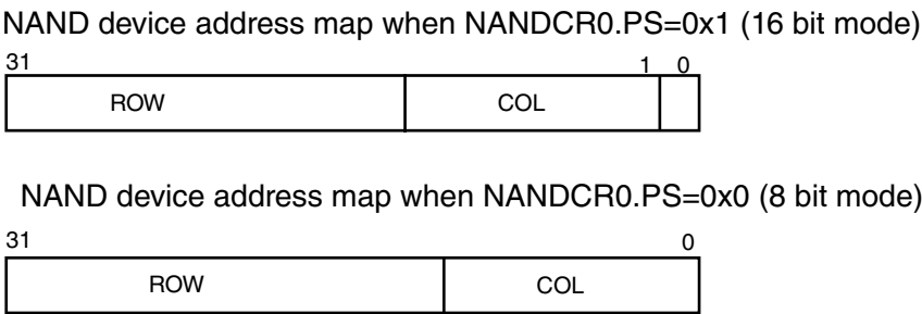
Figure 25-28. NAND Flash Address Multiplexing
