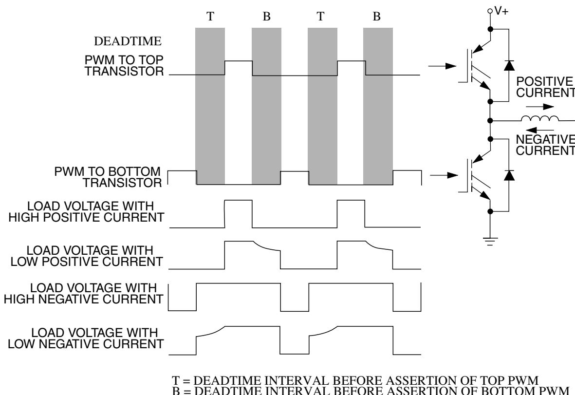
Figure 50-26. Output Voltage Waveforms
