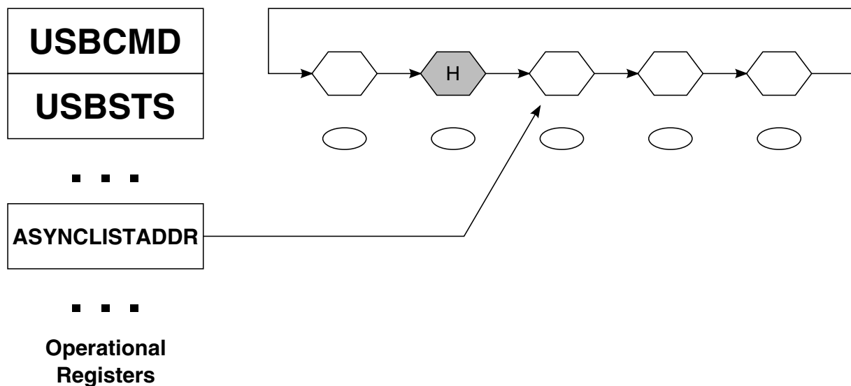
Figure 38-7. General Format of Asynchronous Schedule List
