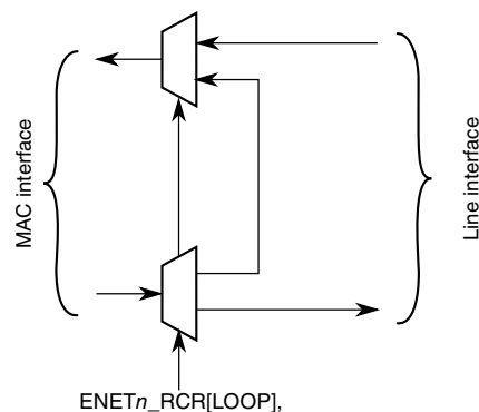
Figure 37-13. Loopback options
