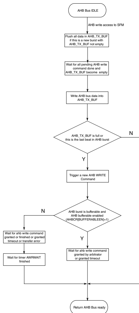
Figure 27-13. Hardware operation in response to AHB write access to Flash
