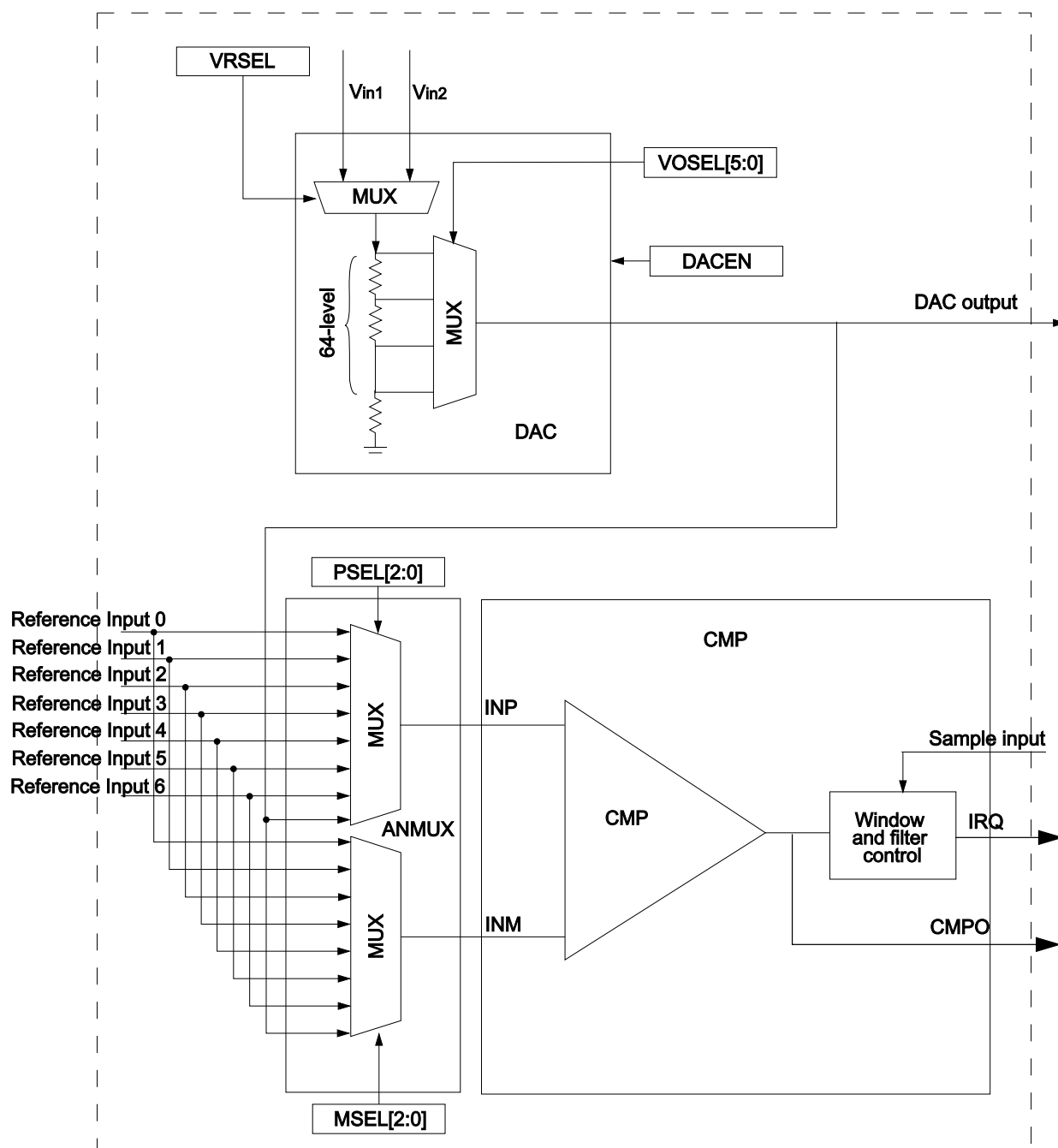
Figure 60-1. CMP, DAC and ANMUX block diagram
