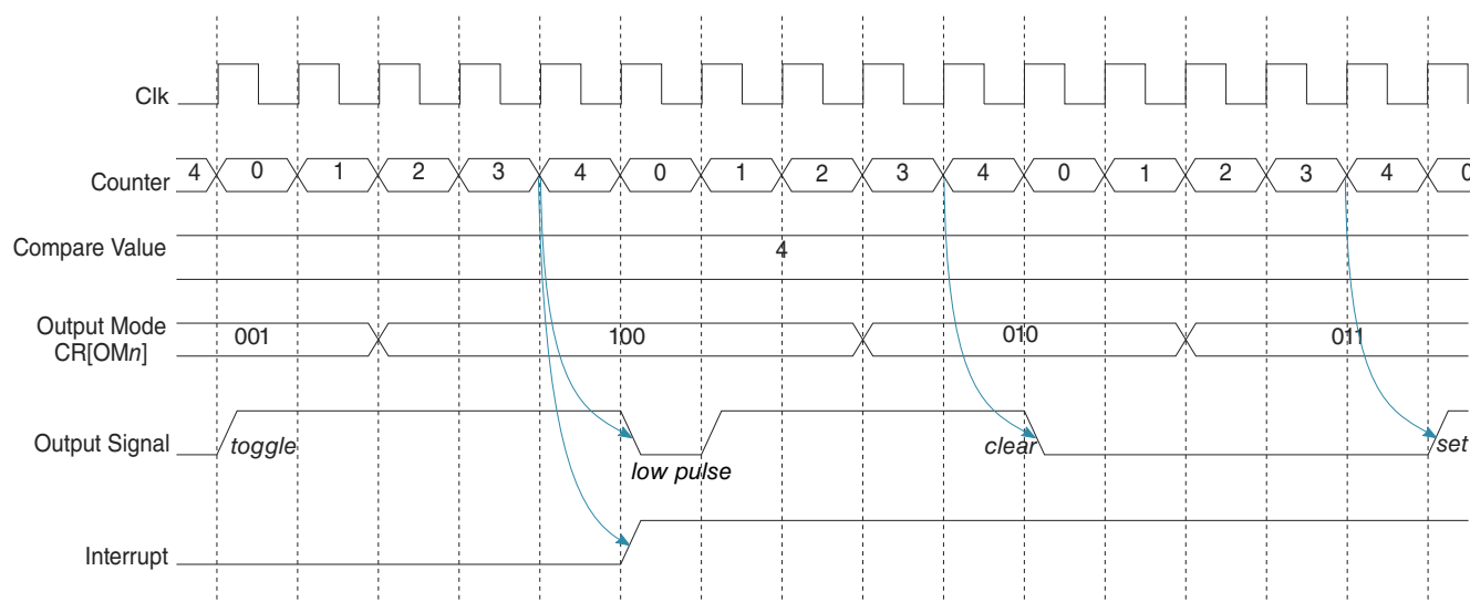
Figure 47-5. Output Compare and Interrupt Timing
