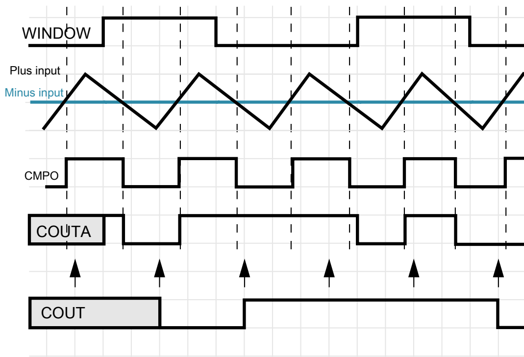
Figure 60-10. Windowed/resampled mode operation
