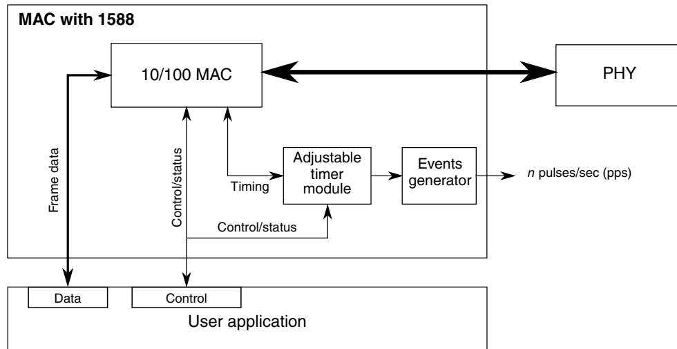
Figure 37-9. IEEE 1588 functions overview
