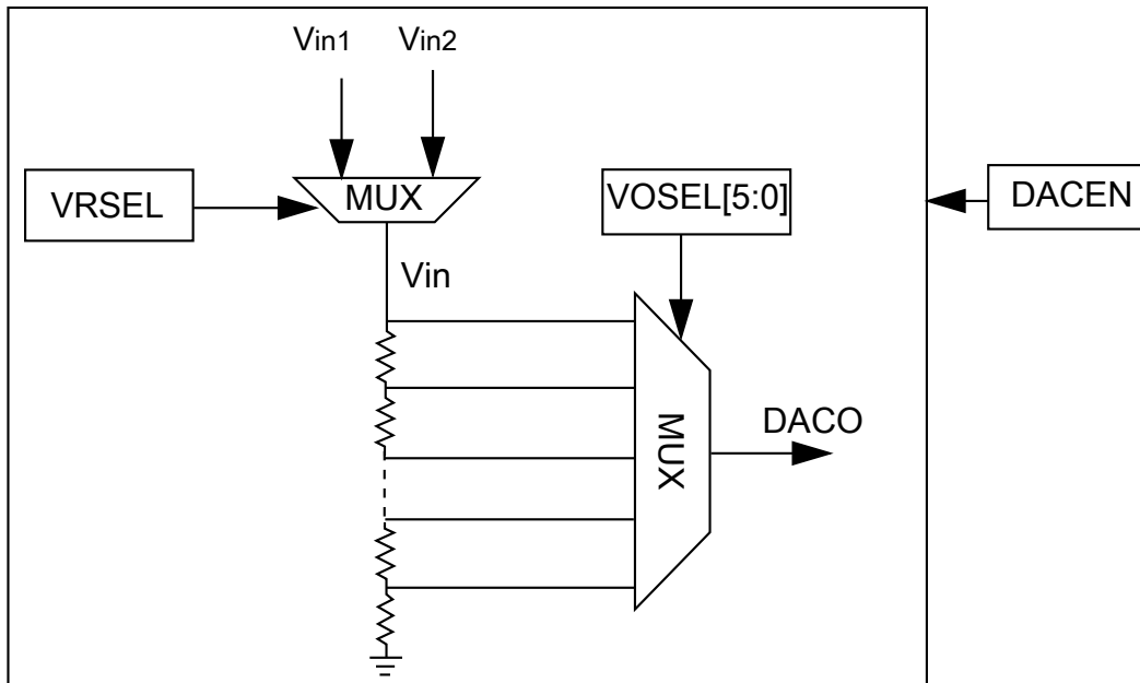
Figure 60-12. 6-bit DAC block diagram
