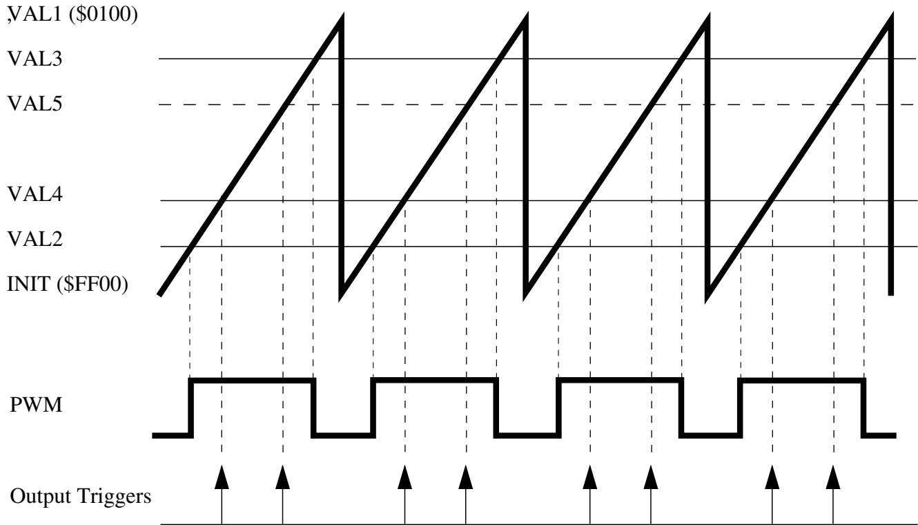
Figure 50-8. Multiple Output Trigger Generation in Hardware
