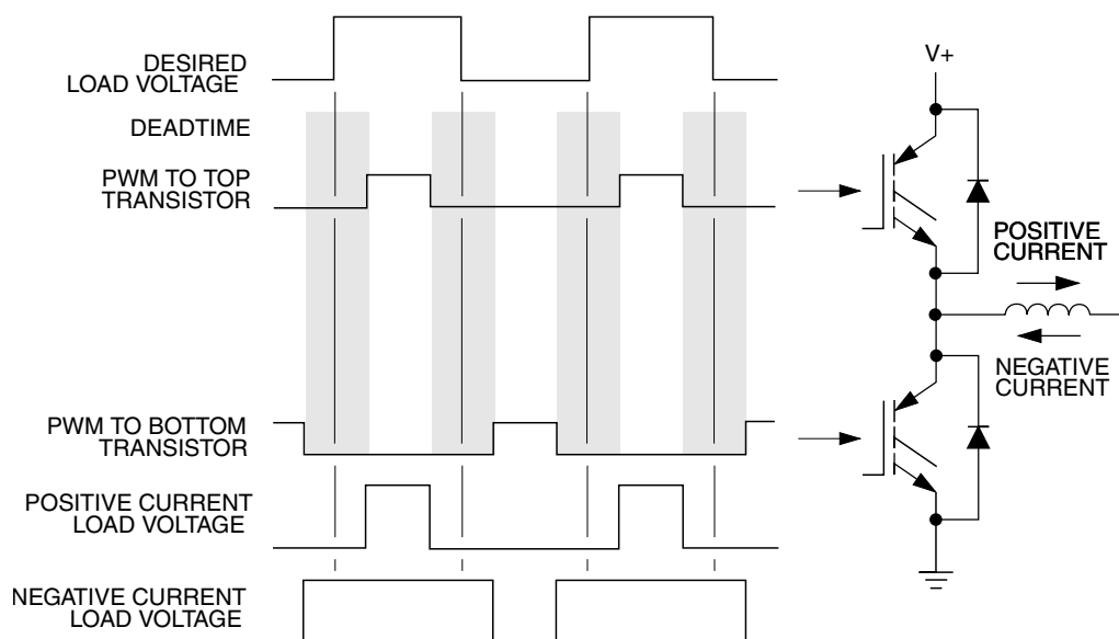
Figure 50-24. Deadtime Distortion
