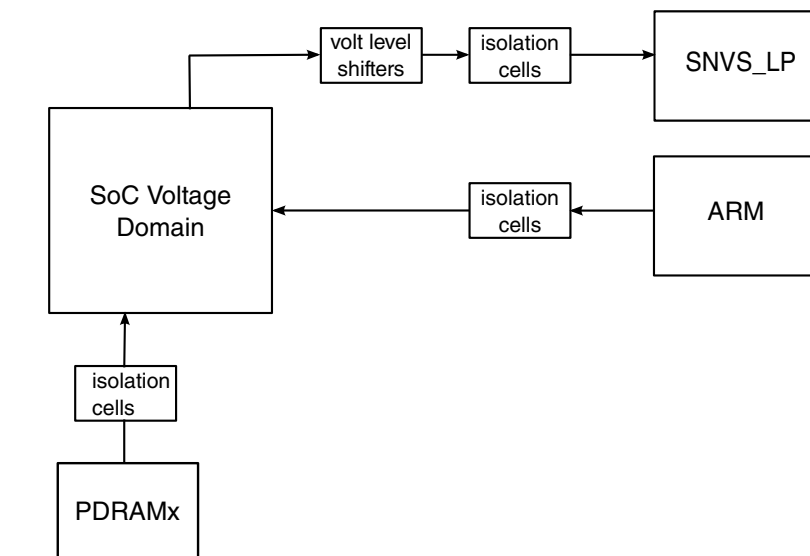
Figure 13-8. Isolation cells and Voltage level shifters placing
