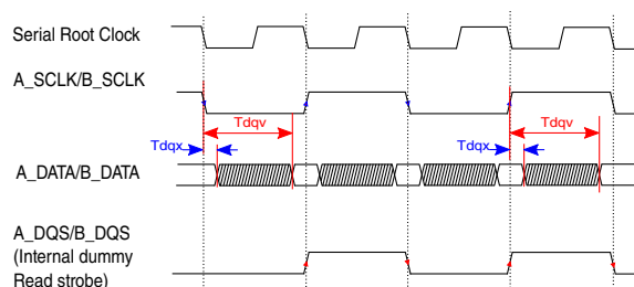
Figure 27-26. Input Timing for sampling with dummy read strobe in DDR mode
