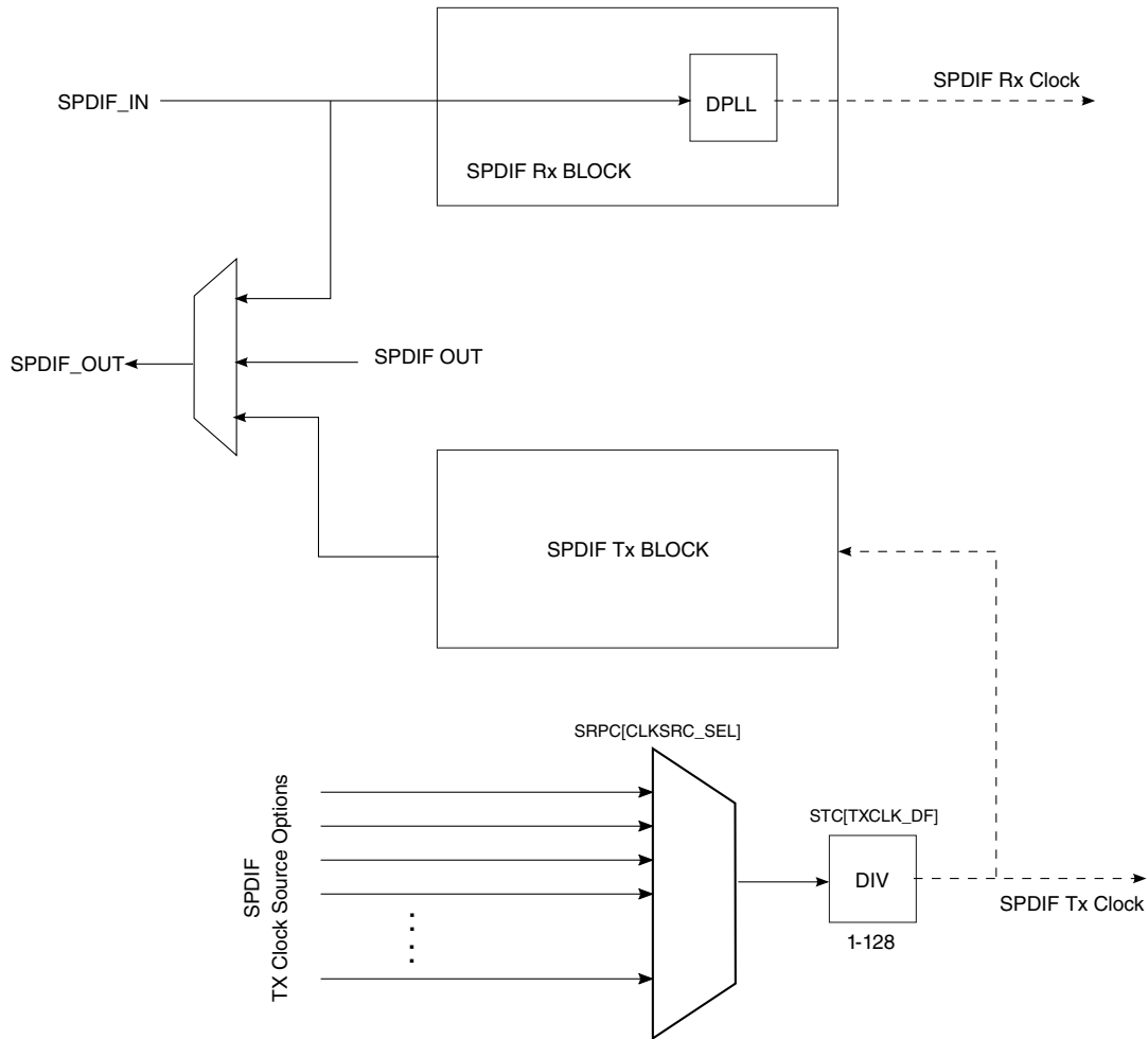
Figure 36-2. SPDIF Transceiver Clock Diagram
