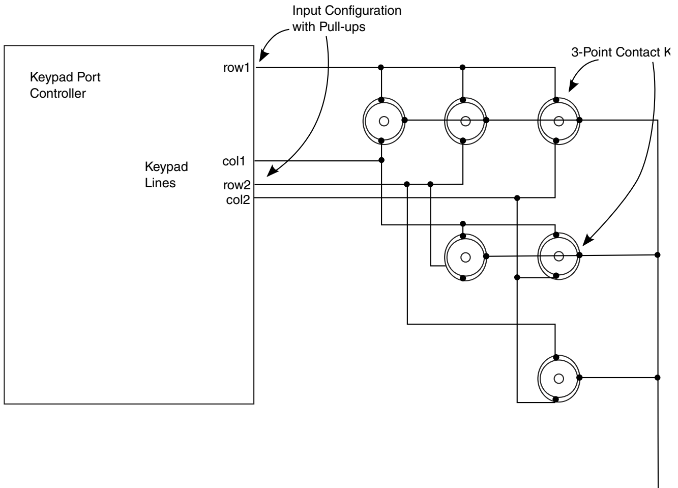
Figure 41-7. KPP Interface with 3-point Contact Key Matrix (Simplified View)
