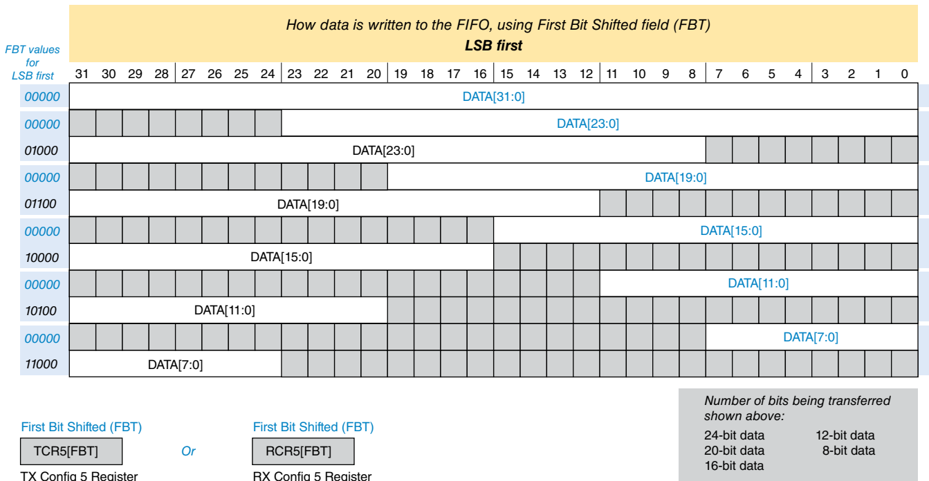
Figure 34-2. SAI first bit shifted, LSB first
