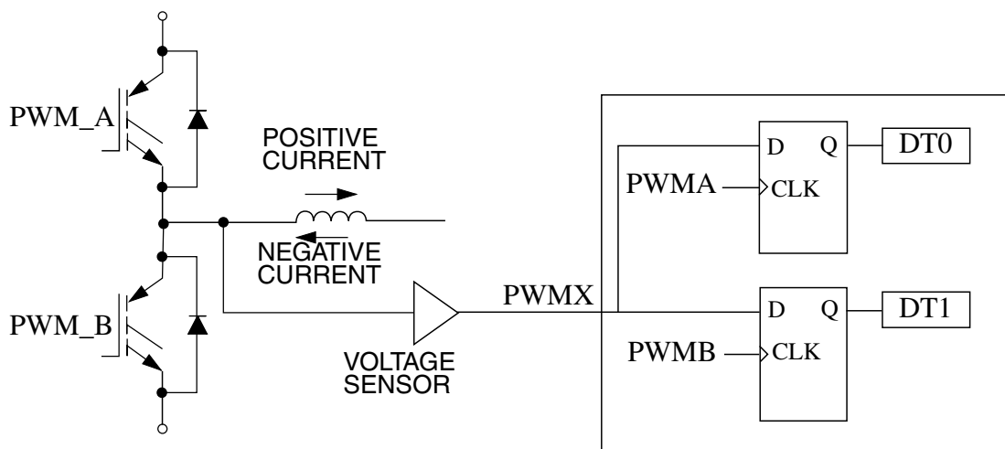
Figure 50-25. Current-status Sense Scheme for Deadtime Correction
