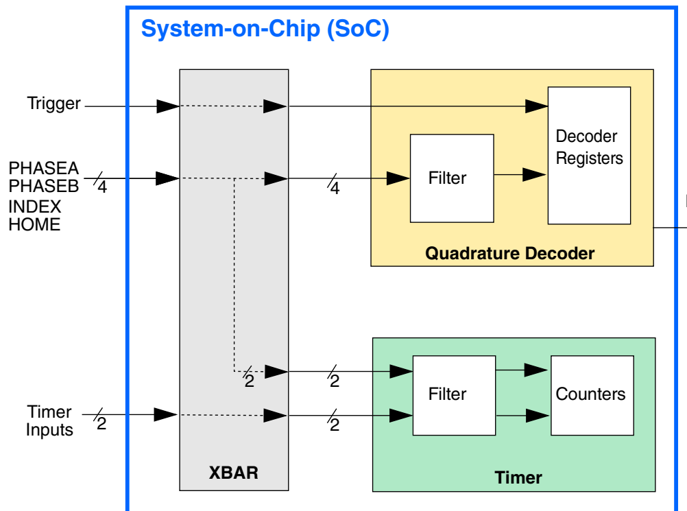
Figure 51-1. System Block Diagram
