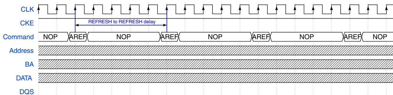
Figure 25-26. Refresh Command - SDRAM AUTO REFRESH
