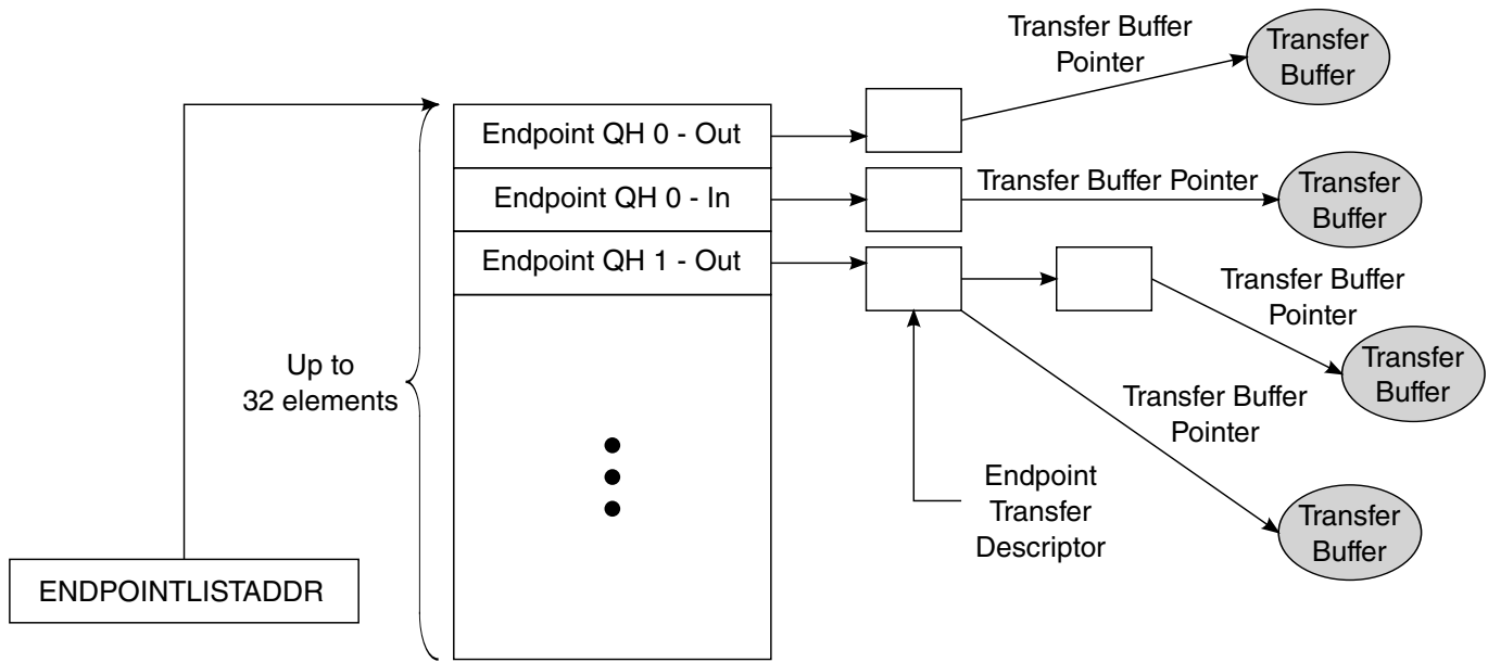
Figure 38-29. End Point Queue Head Diagram
