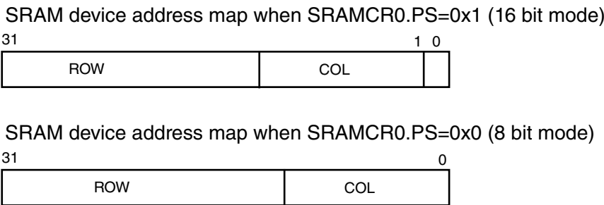
Figure 25-54. SRAM Address Multiplexing
