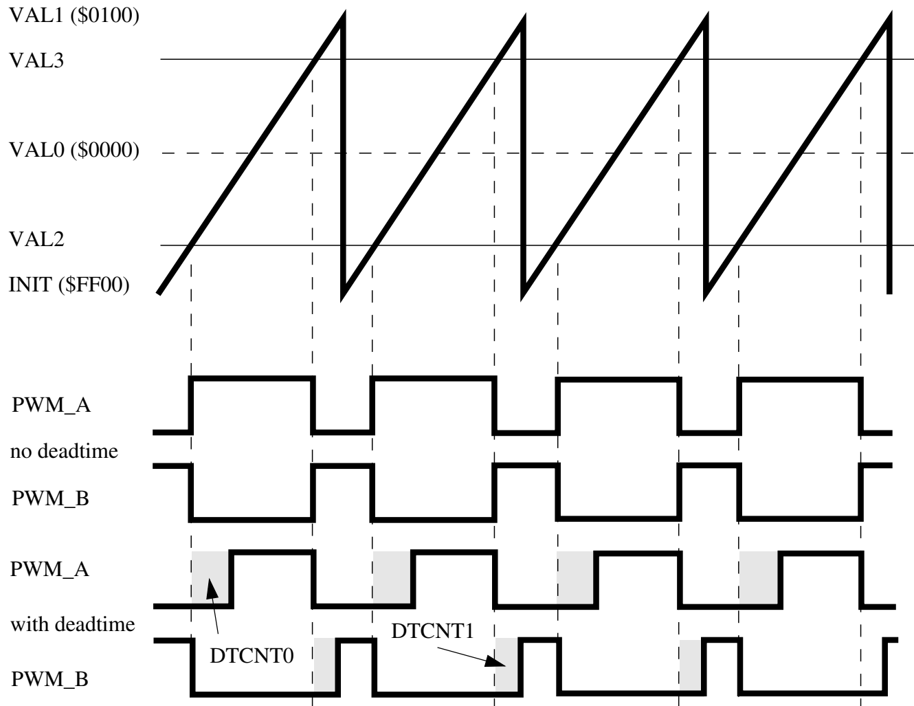
Figure 50-23. Deadtime Insertion
