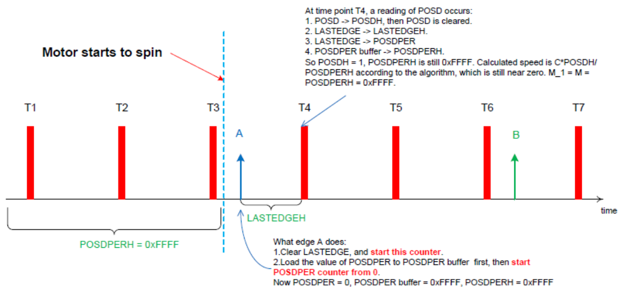
Figure 51-8. Speed measurement at time point T4
