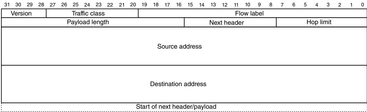
Figure 37-4. IPv6 header format
