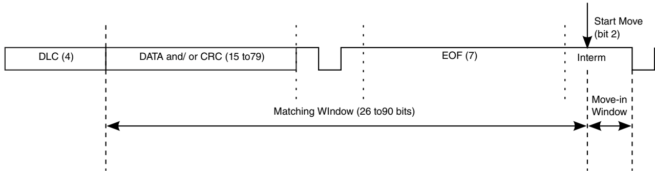
Figure 40-3. Matching and Move-In Time Windows
