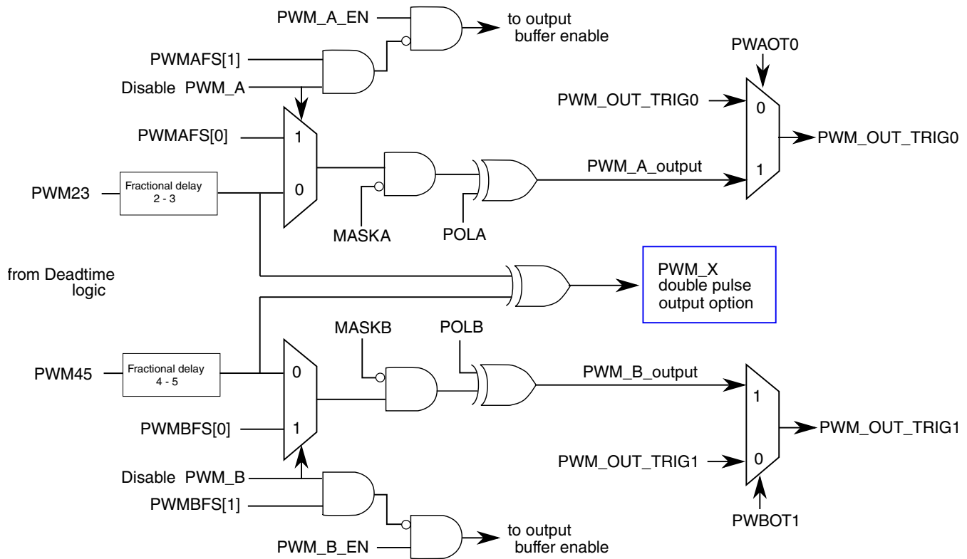
Figure 50-27. Output Logic
