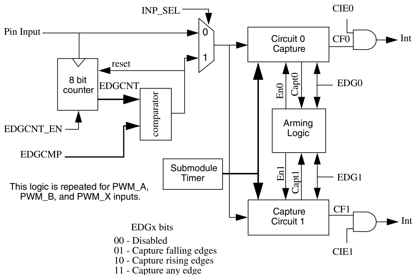
Figure 50-29. Enhanced Capture (E-Capture) Logic
