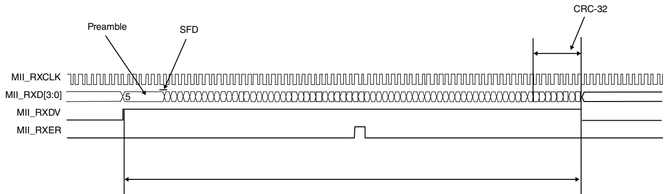
Figure 37-26. MII receive operation — errored frame
