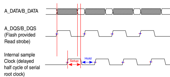
Figure 27-27. Input Timing 2 for Flash provided read strobe in SDR mode
