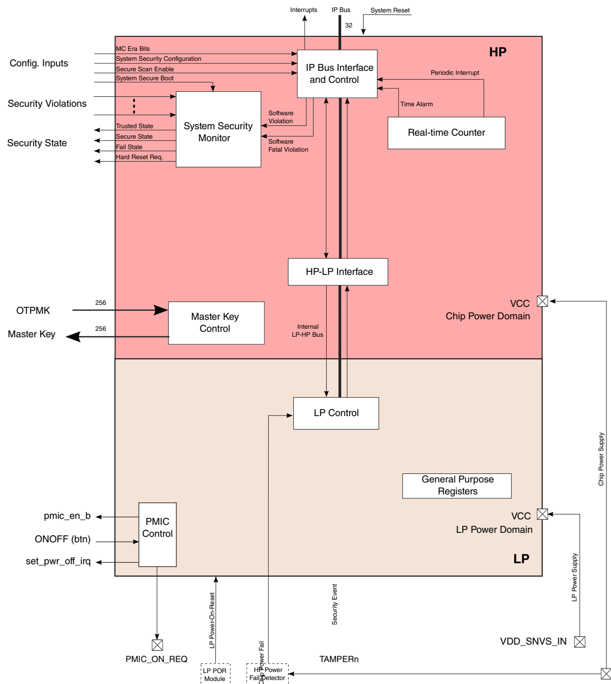
Figure 20-1. SNVS Block Diagram
