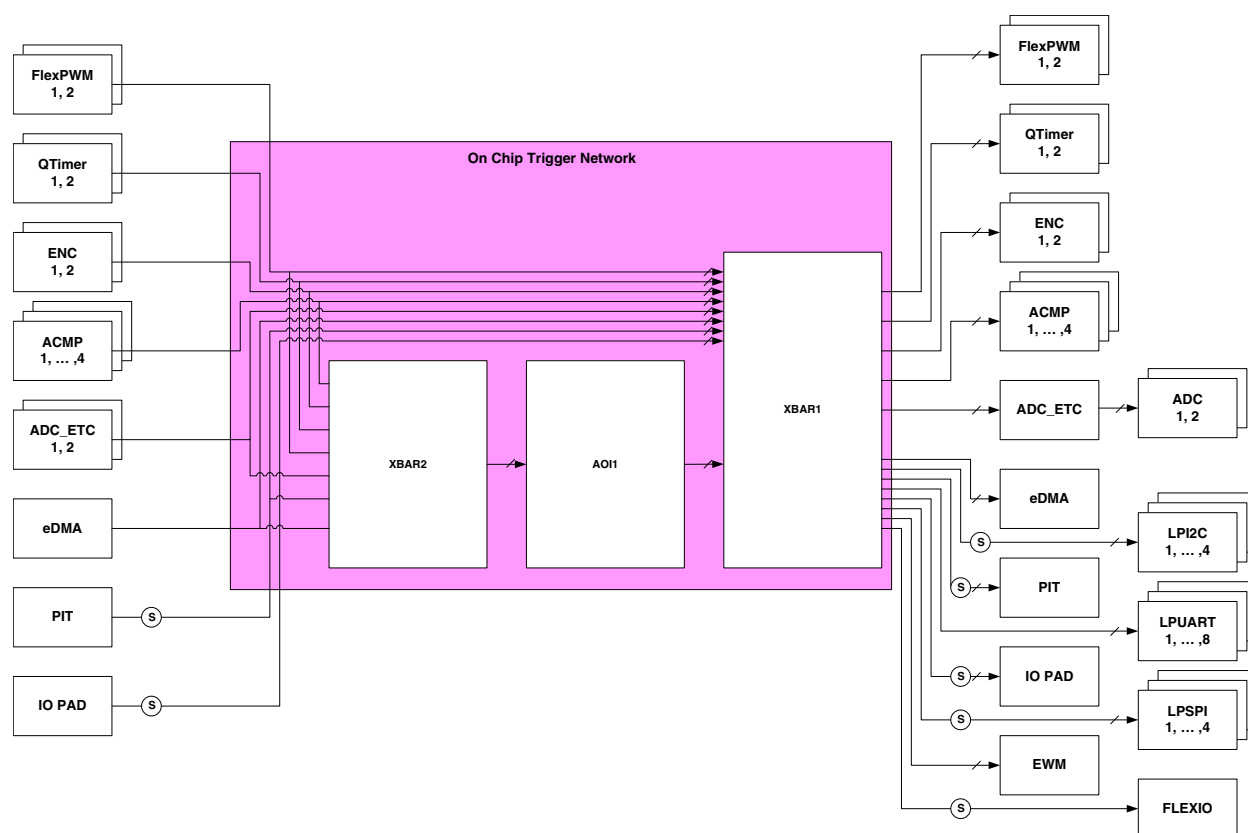
Figure 55-1. On-Chip Cross Trigger Network
