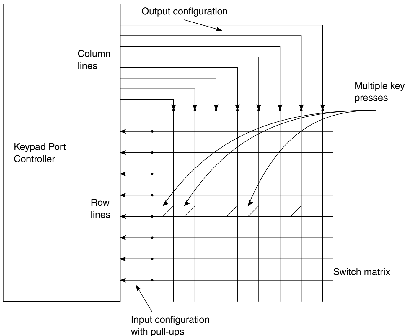
Figure 41-4. Multiple Key Presses on Same Row Line (Simplified View)
