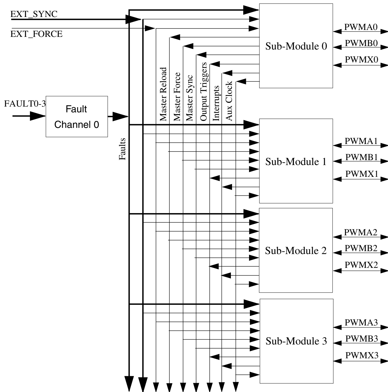
Figure 50-1. PWM Block Diagram
