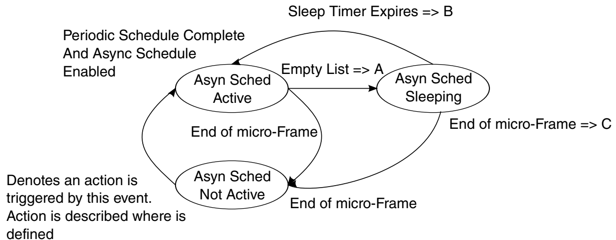
Figure 38-15. Example State Machine for Managing Asynchronous Schedule Traversal
