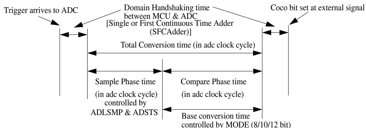
Figure 61-4. ADC conversion time details
