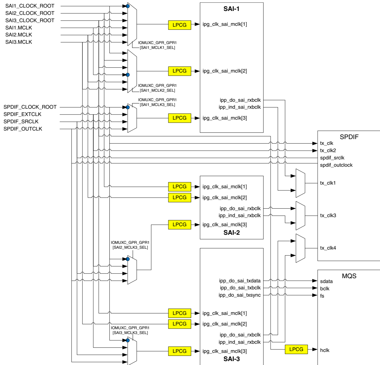
Figure 33-3. Audio subsystem clocking diagram
