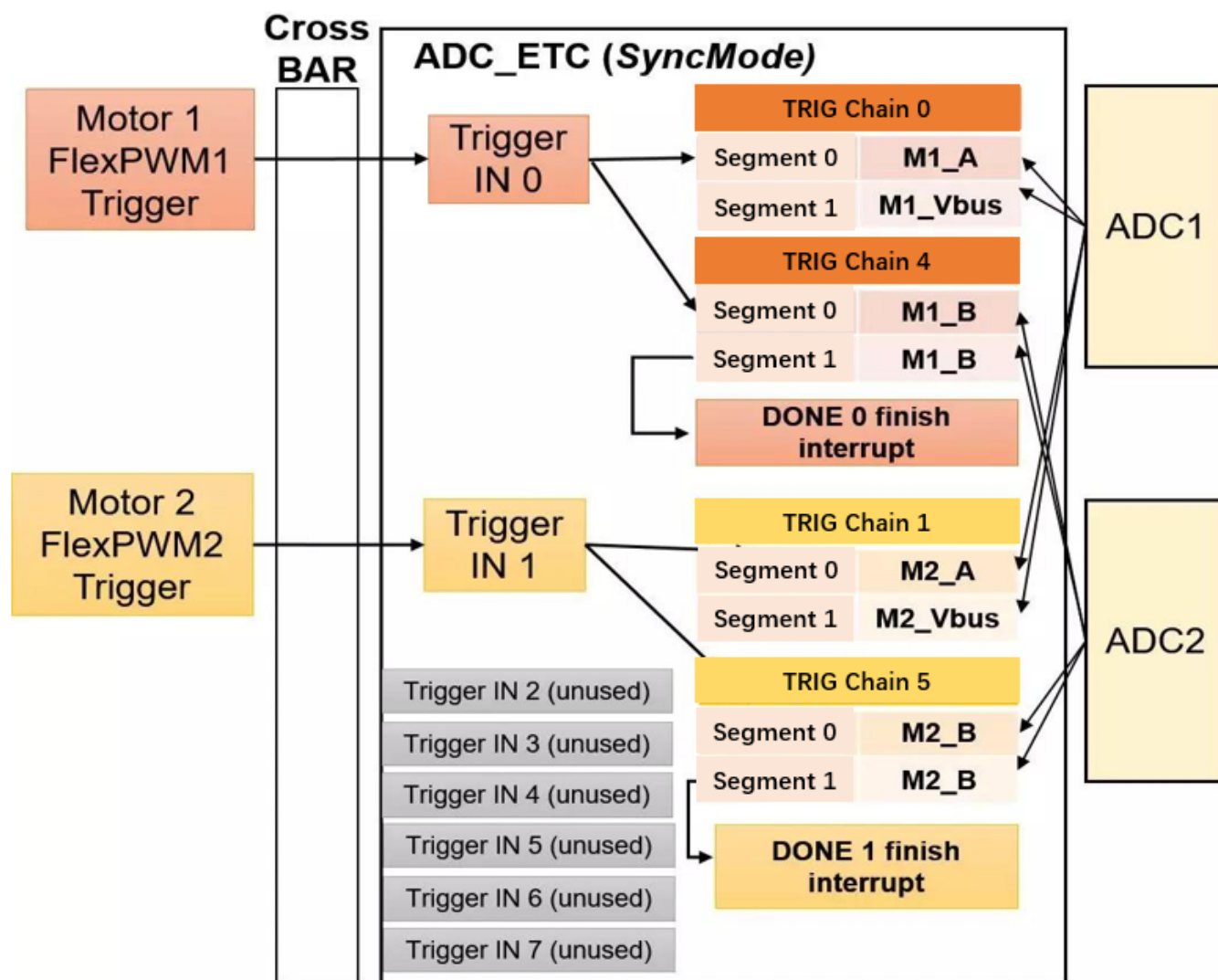
Figure 62-5. The configuration of ADC_ETC for dual motor control
