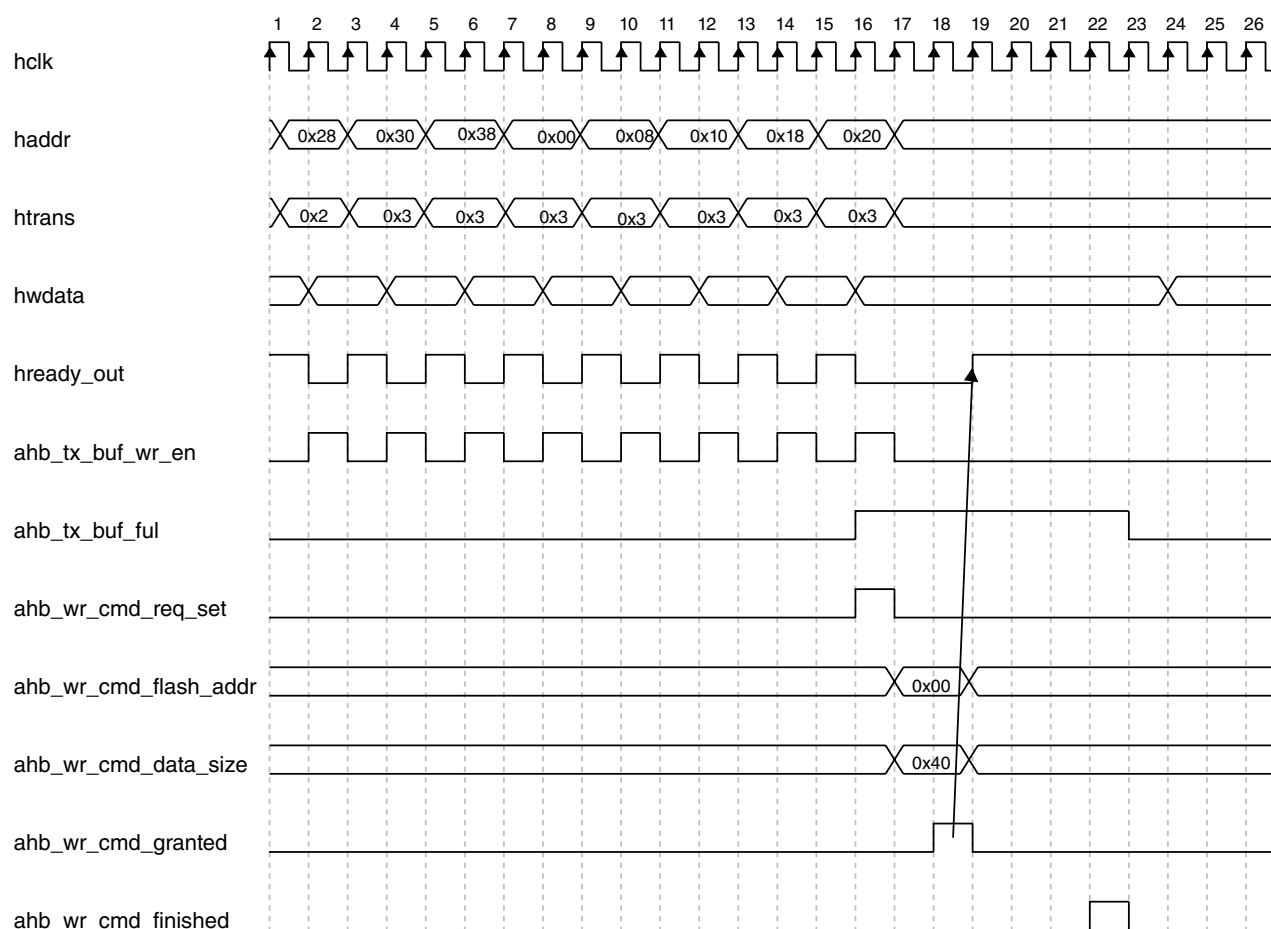
Figure 27-15. AHB write access (WRAP8/64bit/Bufferable)
