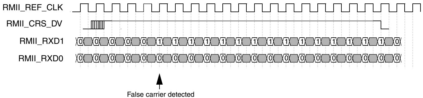
Figure 37-20. RMII receive operation with false carrier
