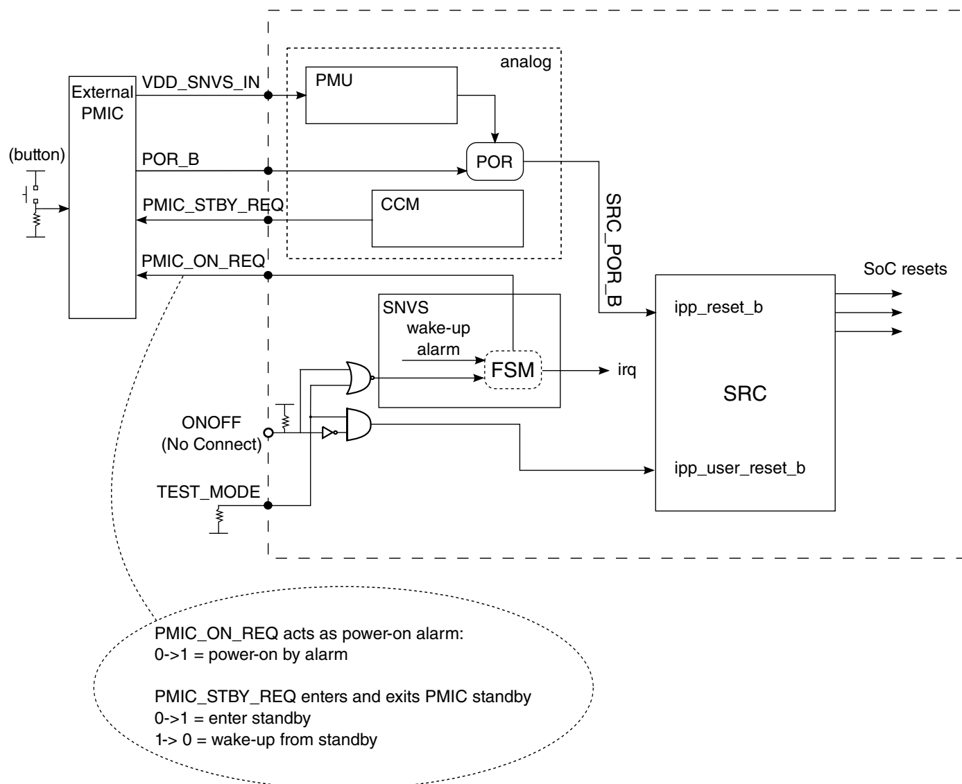
Figure 21-2. Chip reset scheme under external PMIC control
