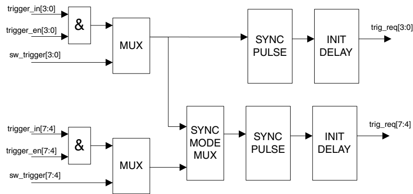
Figure 62-2. Trigger process diagram
