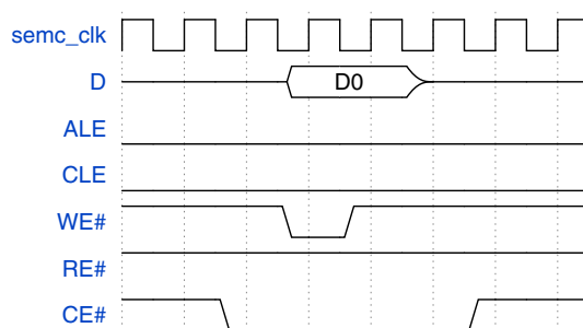
Figure 25-44. NAND Flash Access Command type - Write Phase
