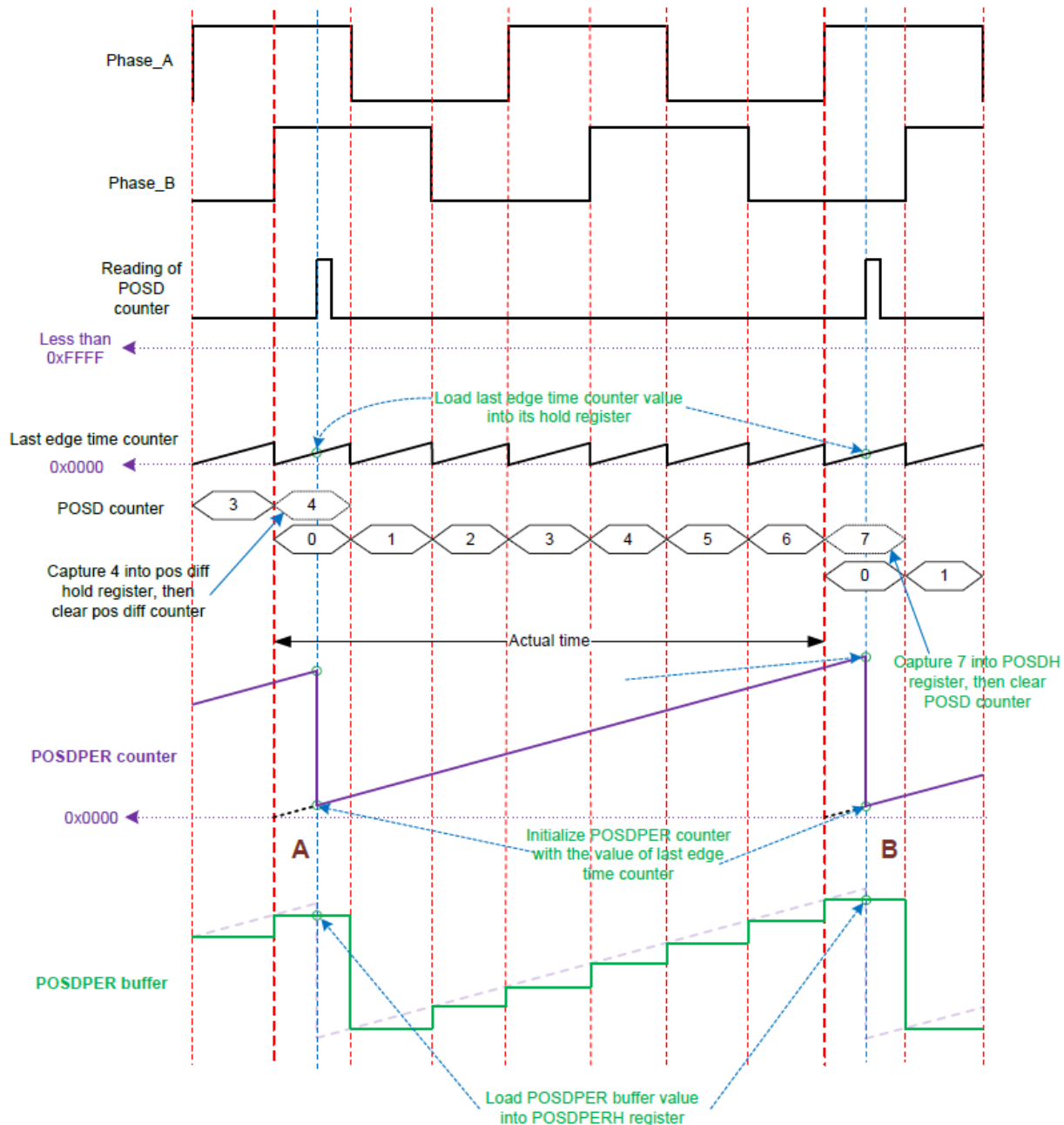
Figure 51-4. Counters behavior and updating mechanism
