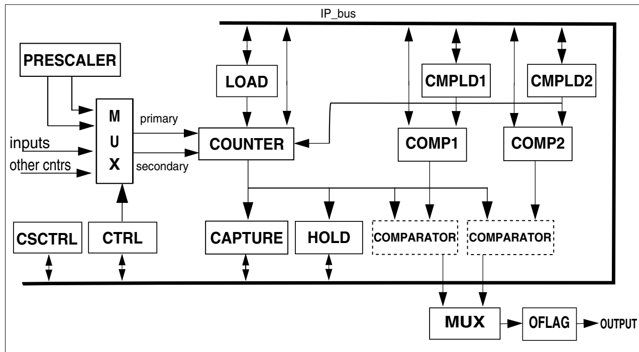
Figure 49-1. Quad Timer Block Diagram
