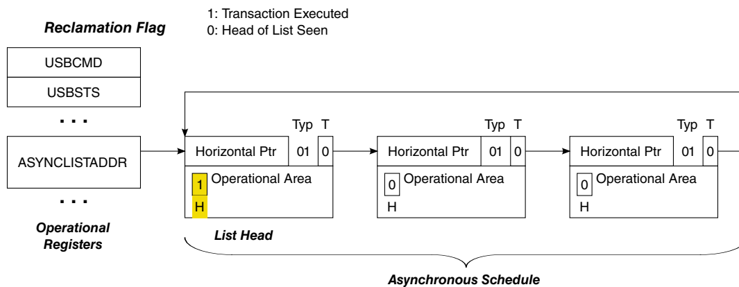
Figure 38-14. Asynchronous Schedule List w/Annotation to Mark Head of List
