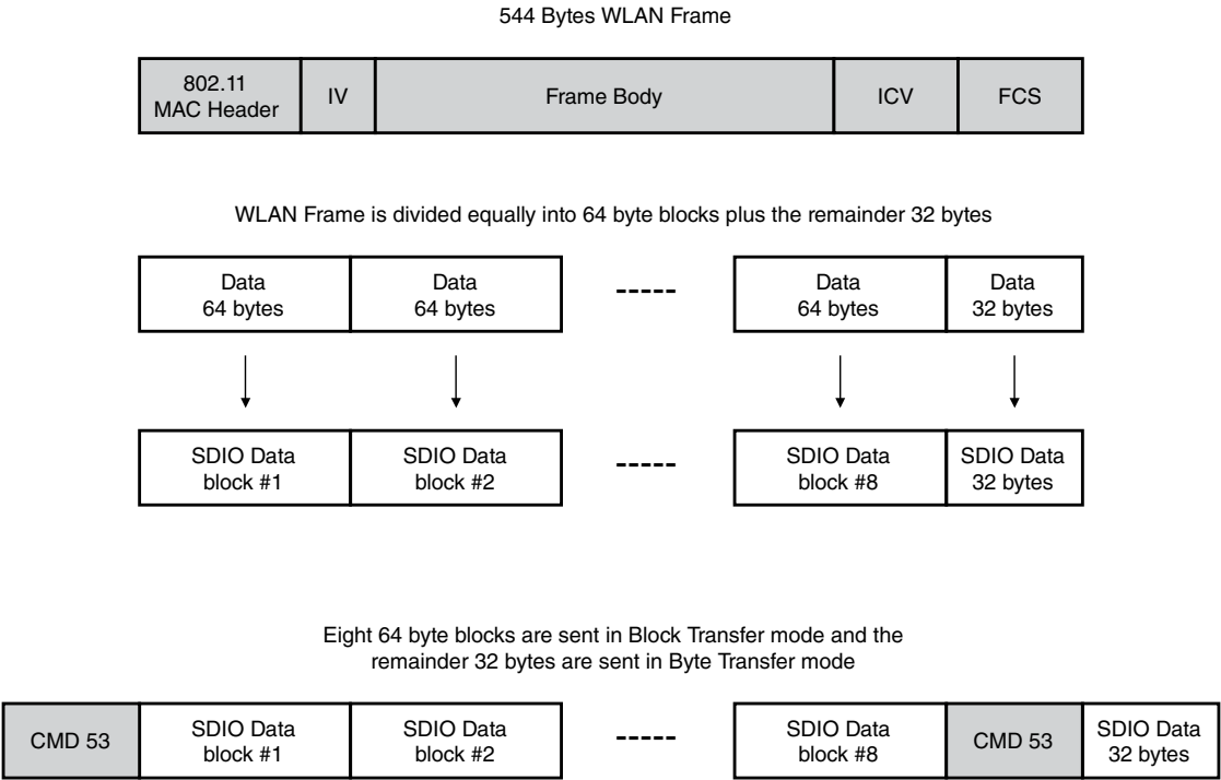
Figure 26-6. Example for dividing large data transfers
