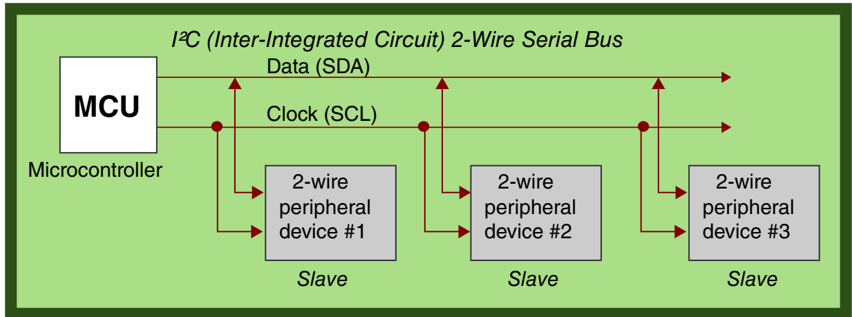
Figure 42-2. I²C 2-wire serial bus
