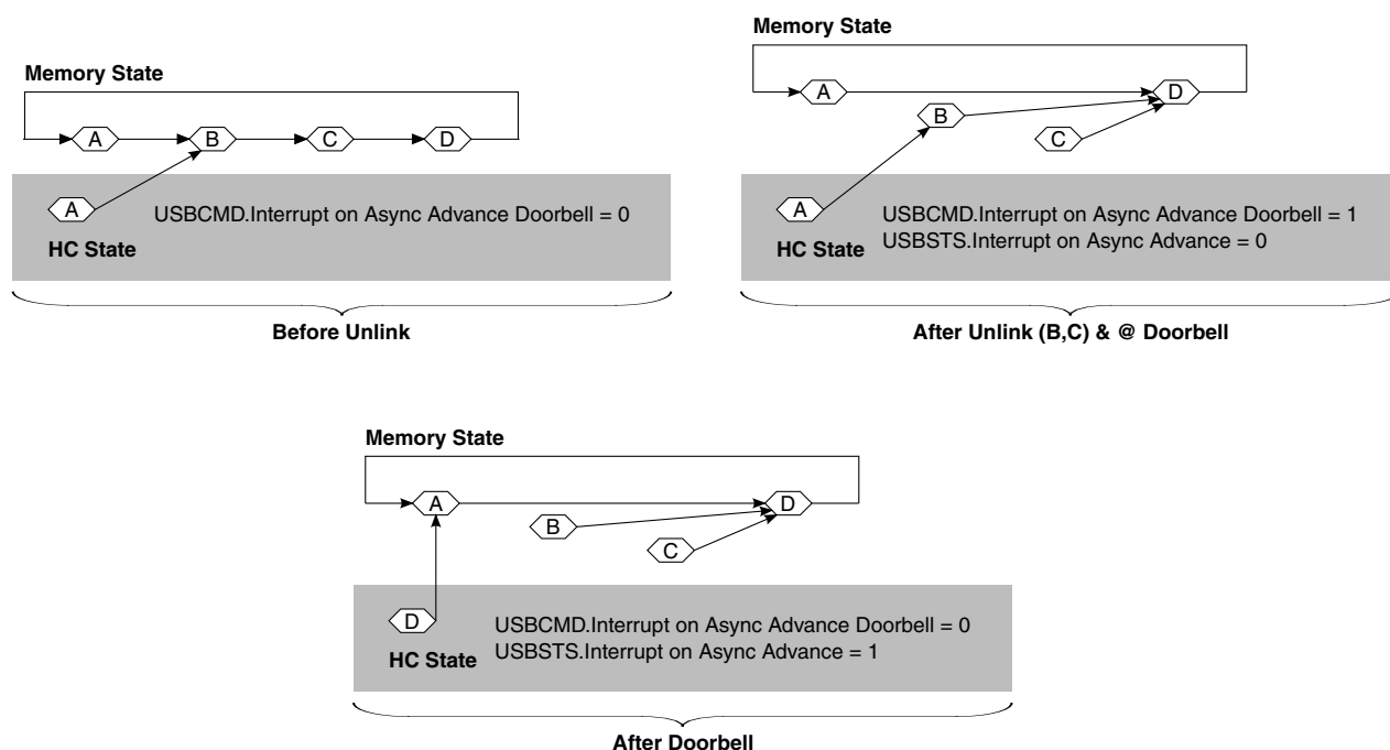
Figure 38-13. Generic Queue Head Unlink Scenario
