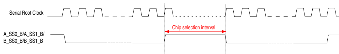
Figure 27-24. Chip Selection Valid interval
