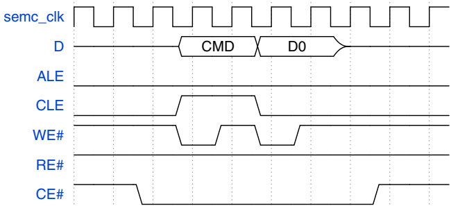
Figure 25-42. NAND Flash Access Command Type - Command + Write Phase
