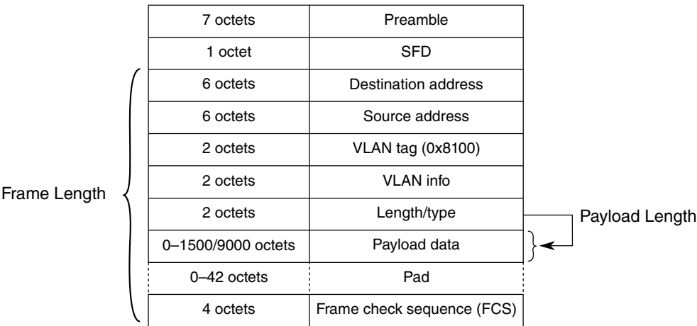
Figure 37-3. VLAN-tagged MAC frame format overview
