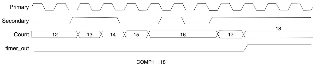
Figure 49-4. Triggered Count Mode 1 (CTRL[LENGTH]=0)
