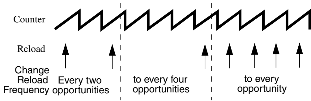
Figure 50-35. Half Cycle Reload Frequency Change
