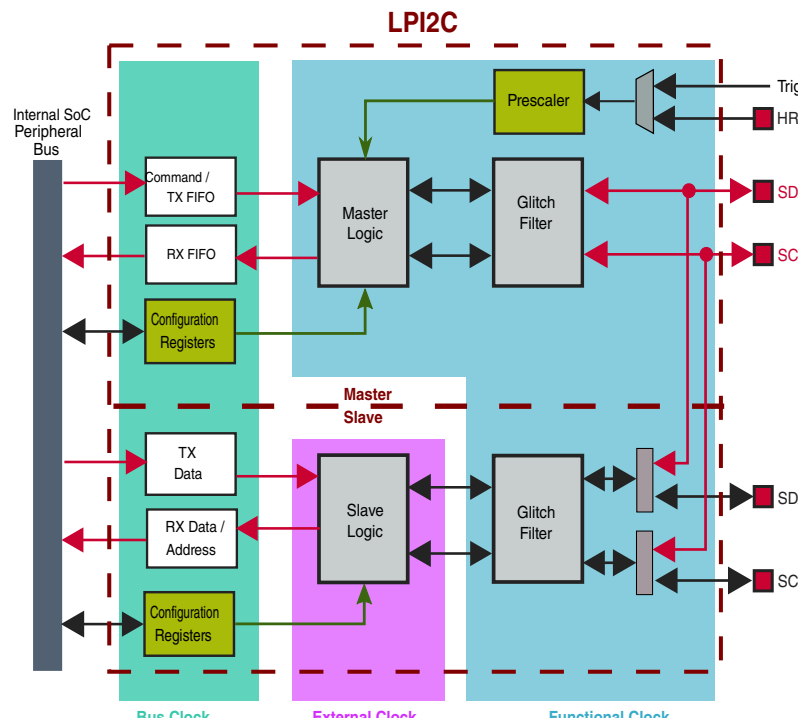
Figure 42-1. LPI2C block diagram
