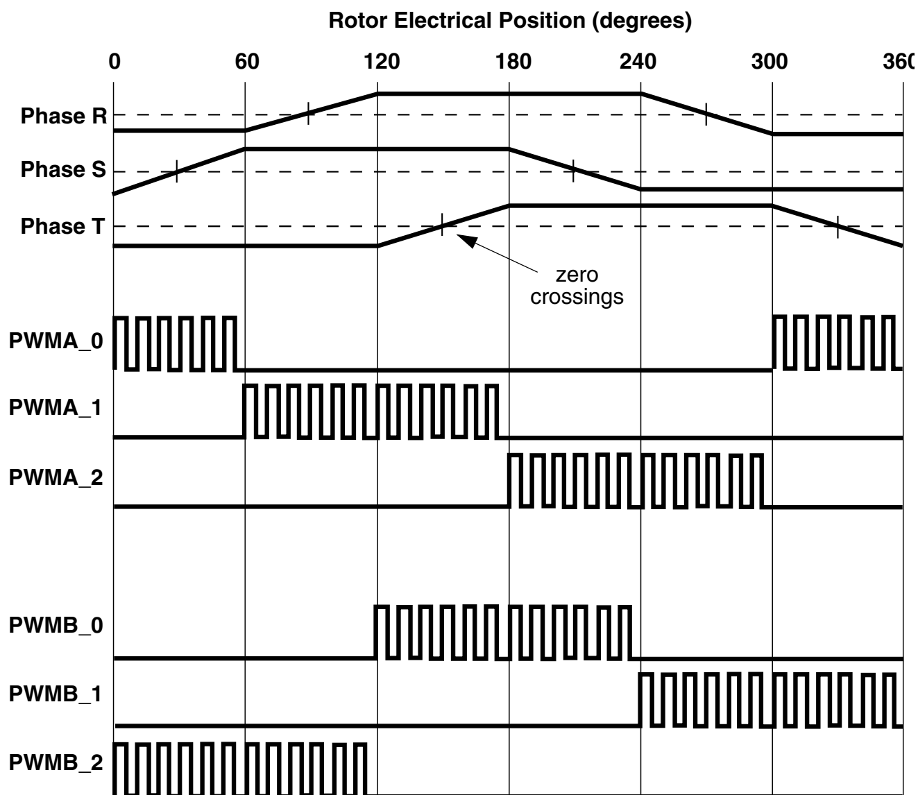
Figure 50-12. Sensorless BLDC Commutation Using the Force Out Function
