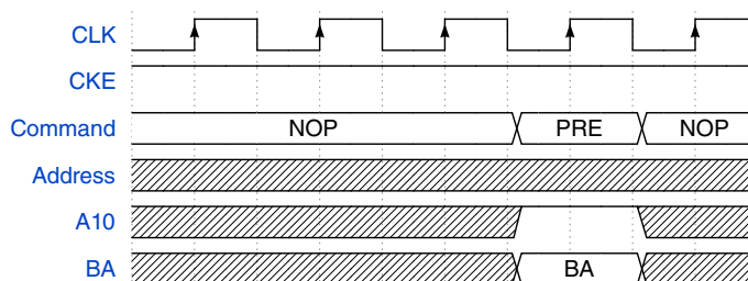
Figure 25-10. IP Command - SDRAM PRECHARGE ALL
