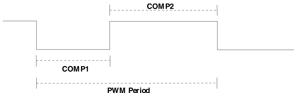
Figure 49-2. Variable PWM Waveform
