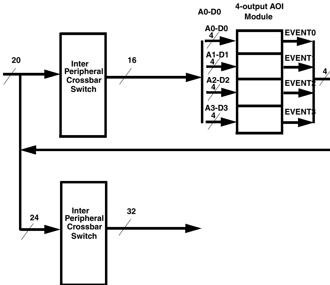
Figure 58-2. Integration Example of AOI with two Inter-Peripheral Crossbar Switches
