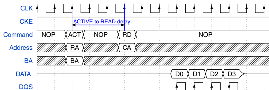
Figure 25-3. IP Command - SDRAM READ
