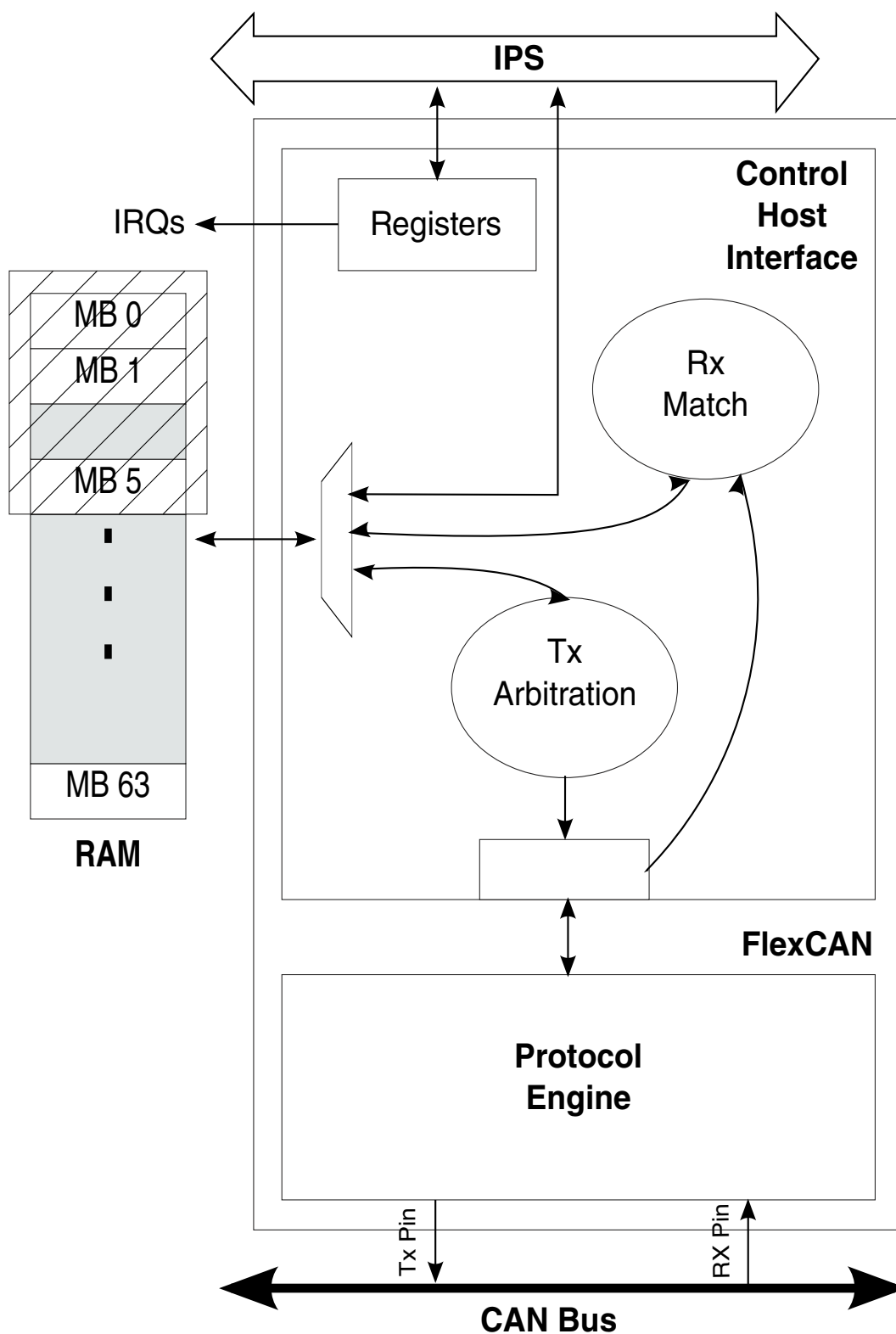
Figure 40-1. FLEXCAN Block Diagram
