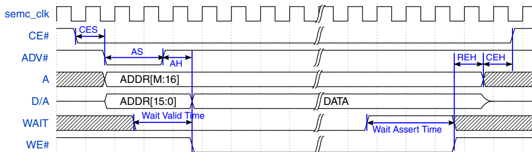
Figure 25-61. SRAM Write in ASYNC Mode (ADMUX) with Wait Pin
