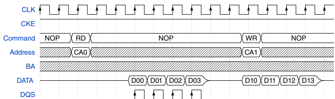
Figure 25-21. SDRAM Read-to-Write Access (CL=3)
