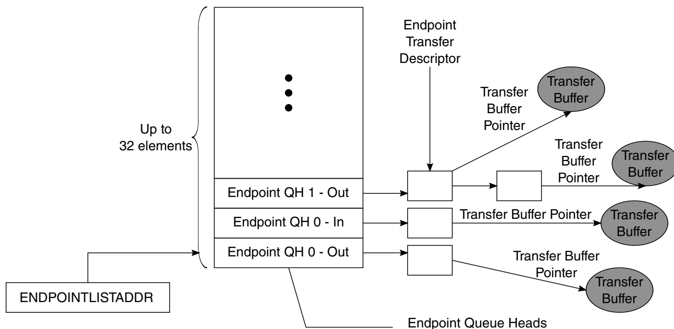
Figure 38-27. EndPoint Queue Head Organization
