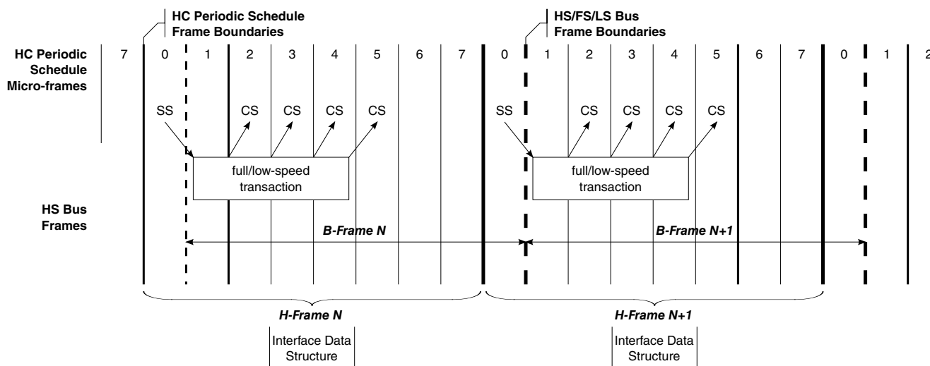
Figure 38-10. Relationship of Periodic Schedule Frame Boundaries to Bus Frame Boundaries
