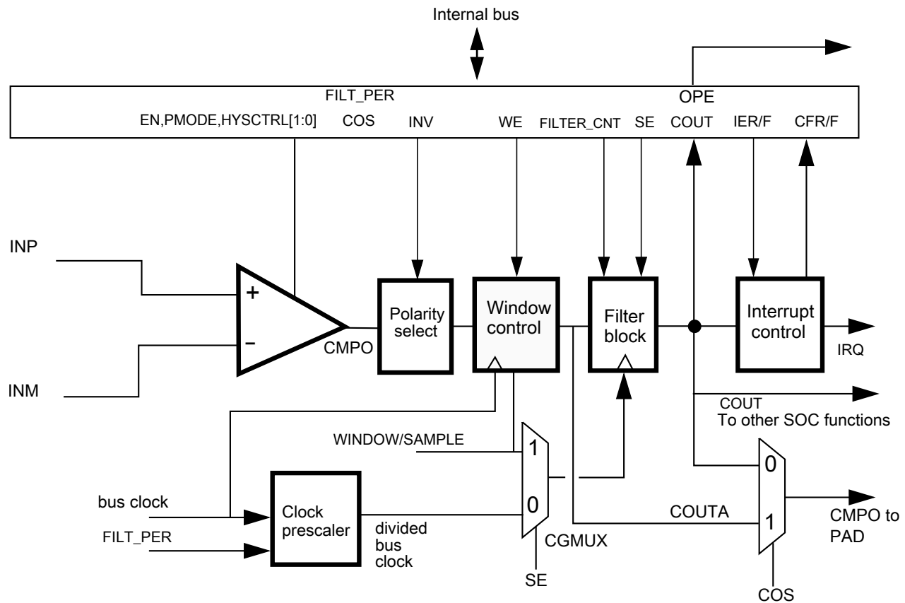
Figure 60-2. Comparator module block diagram
