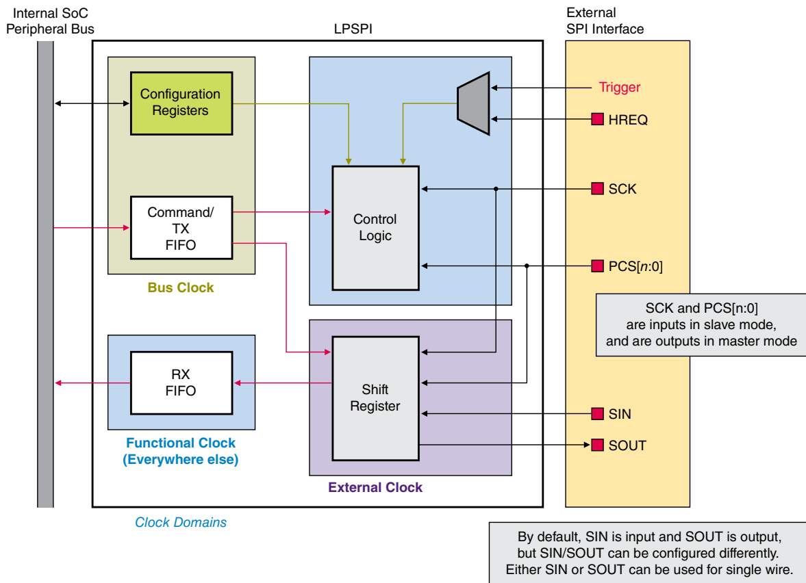
Figure 43-1. Block diagram
