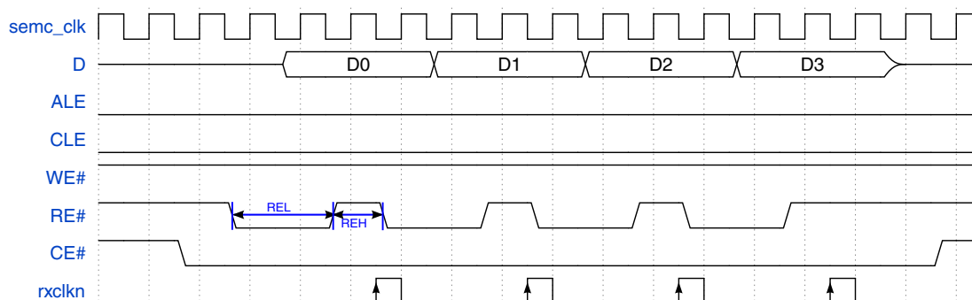
Figure 25-47. NAND Flash Read Access in EDO mode
