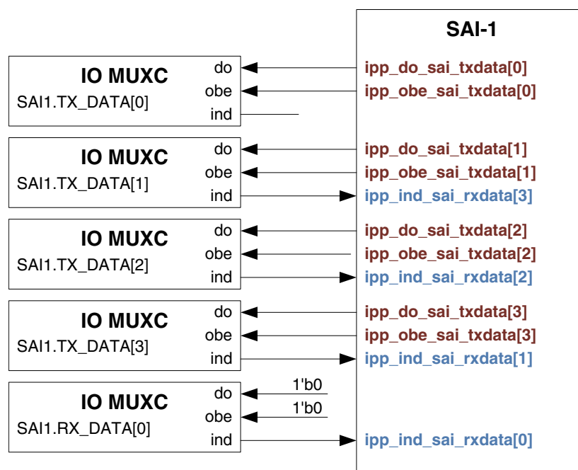
Figure 33-2. SAI-1 TX/RX Data Multiplexing
