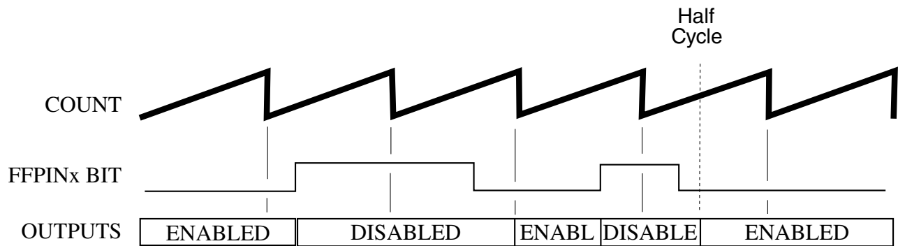
Figure 50-31. Automatic Fault Clearing
