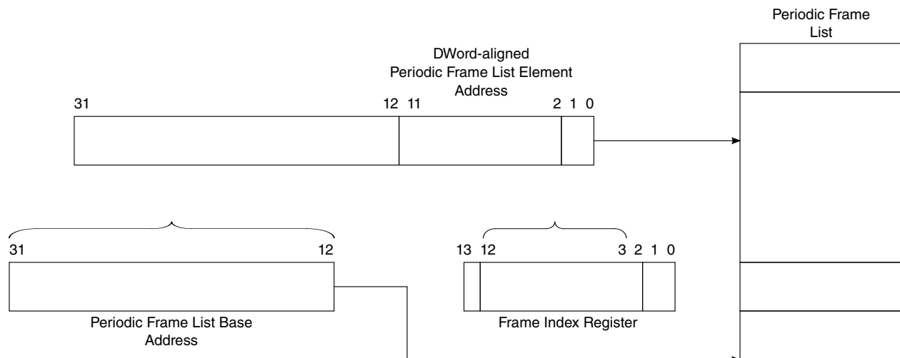
Figure 38-6. Derivation of Pointer into Frame List Array
