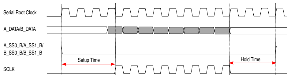
Figure 27-22. Chip selection output timing for SDR sequence
