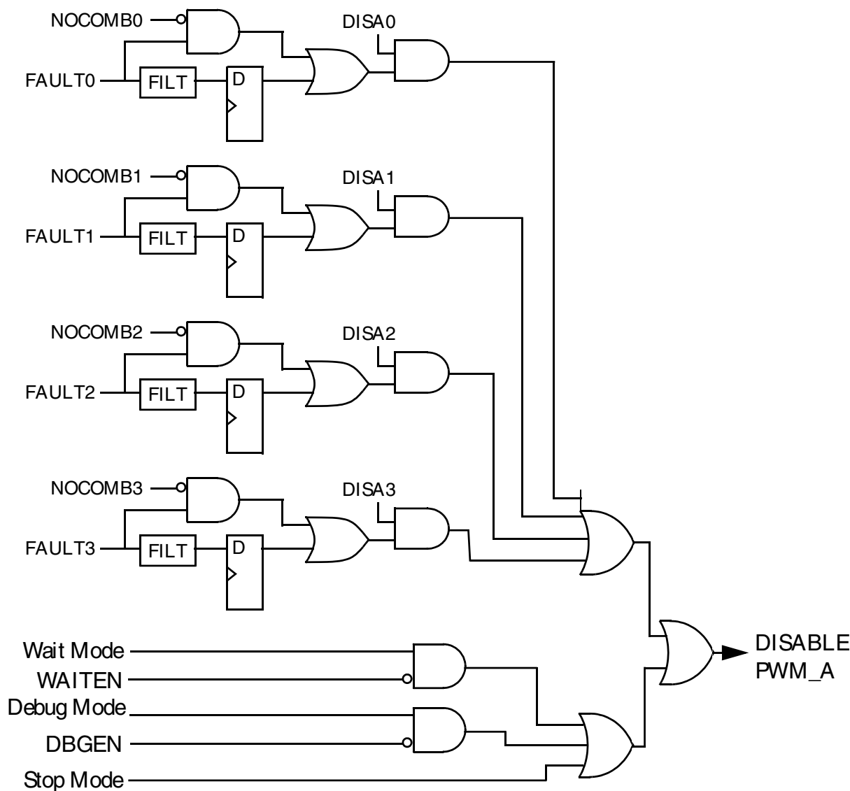
Figure 50-30. Fault Decoder for PWM_A
