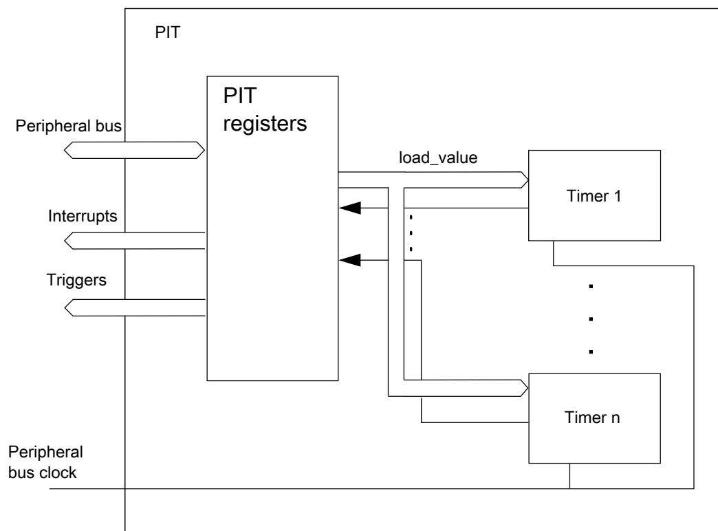
Figure 48-1. Block diagram of PIT
