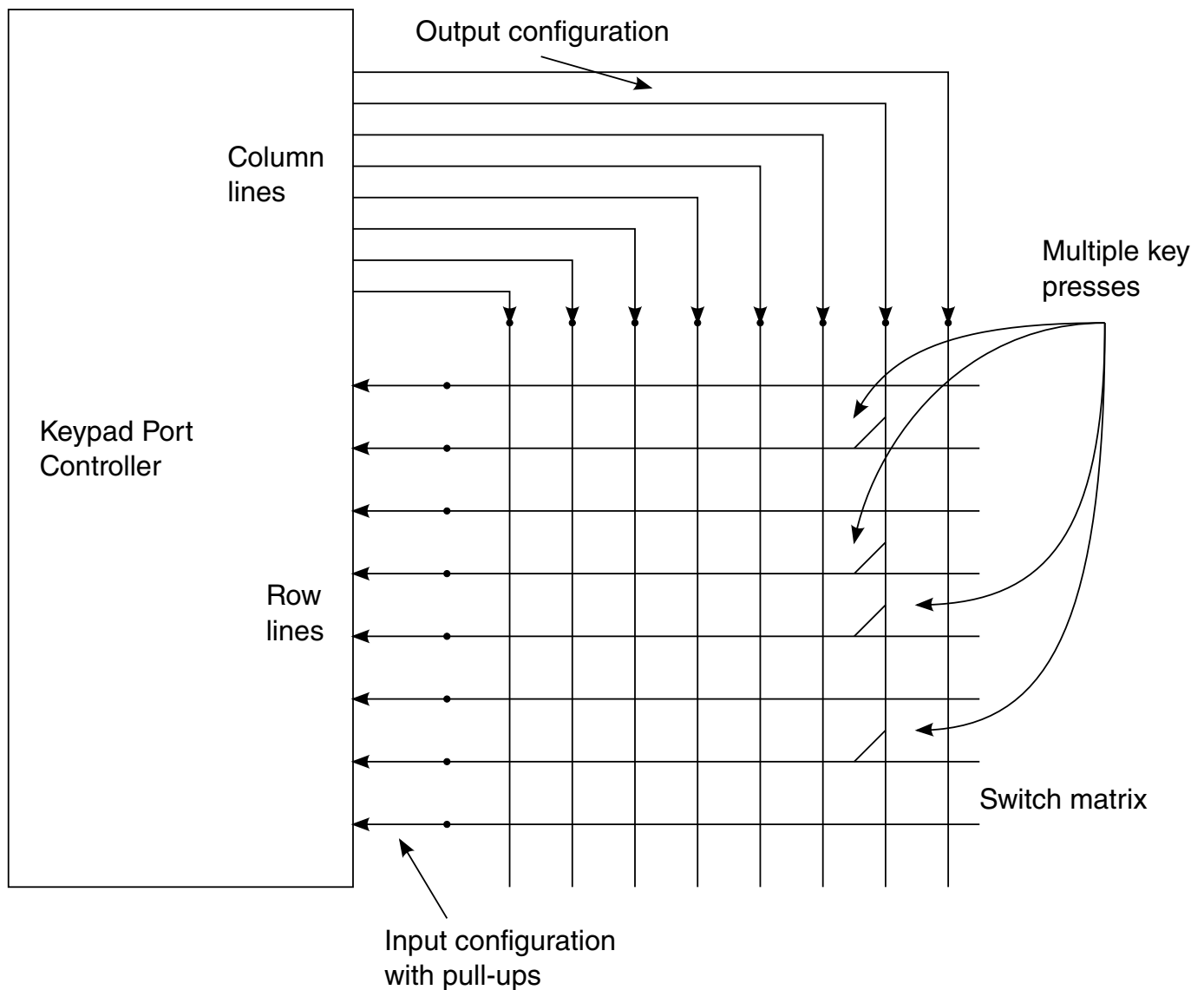
Figure 41-3. Multiple Key Presses on Same Column Line (Simplified View)
