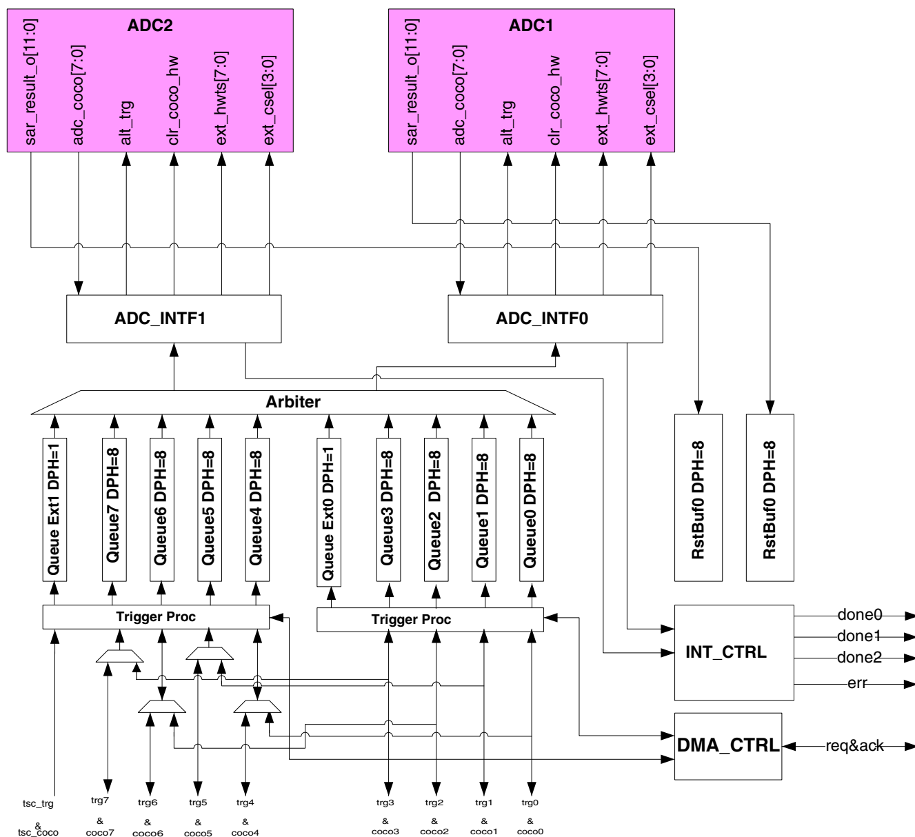
Figure 62-1. ADC_ETC block diagram
