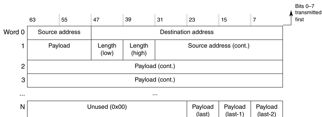
Figure 37-14. Normal Ethernet frame 64-bit mapping example
