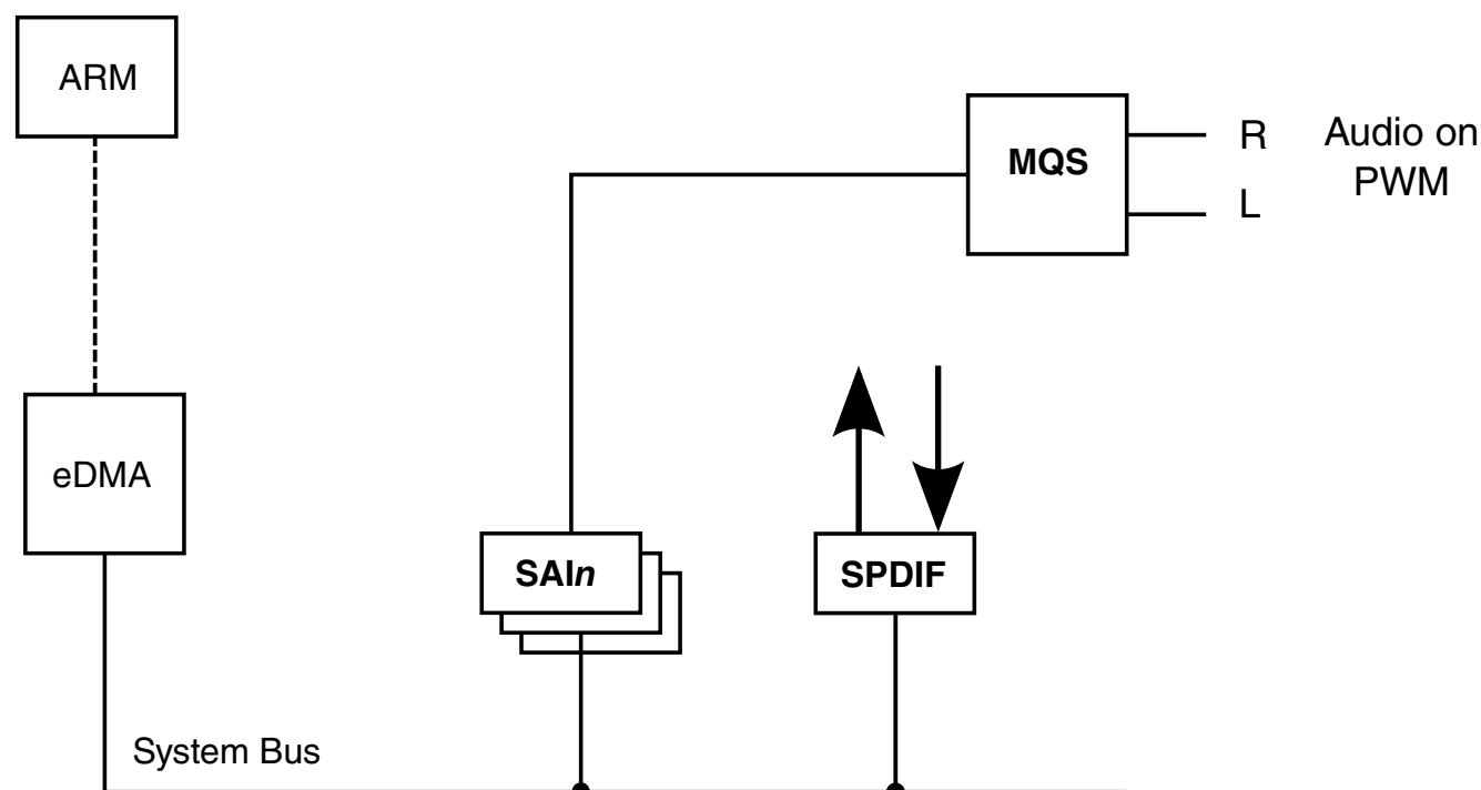
Figure 33-1. Audio peripherals block diagram
