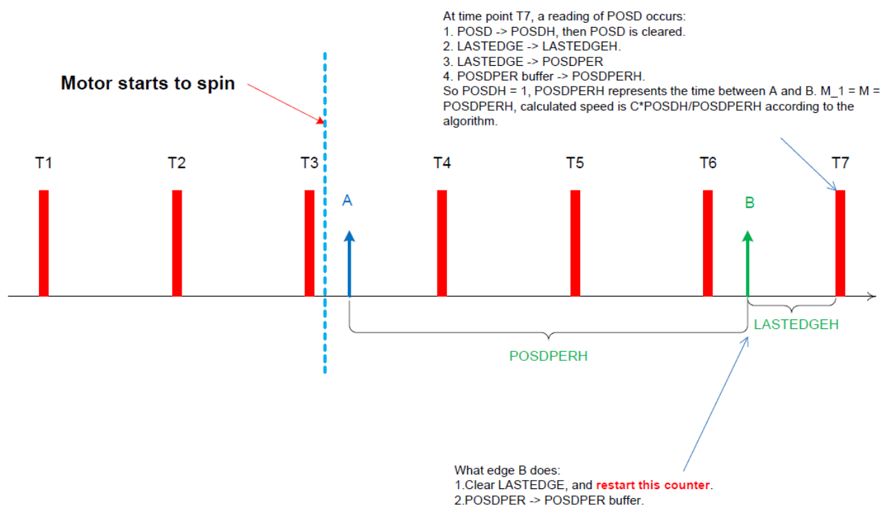
Figure 51-10. Speed measurement at time point T7
