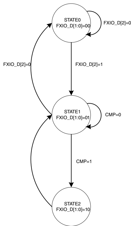
Figure 45-5. State Diagram
