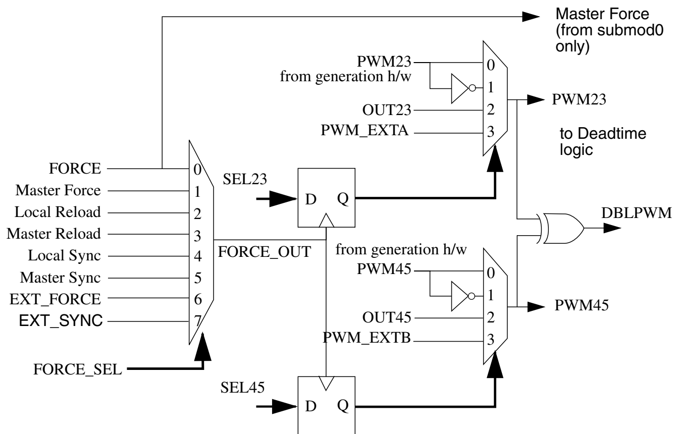
Figure 50-19. Force Out Logic
