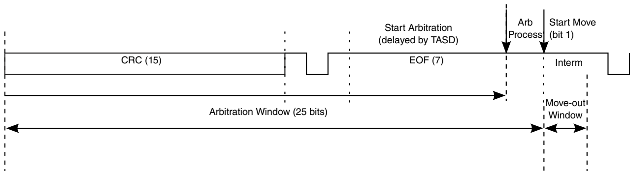
Figure 40-4. Arbitration and Move-Out Time Windows
