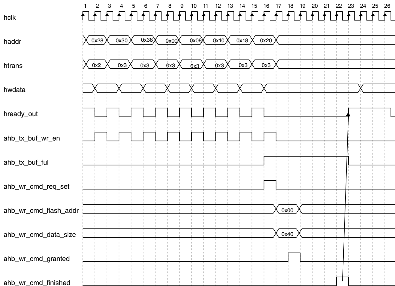
Figure 27-16. AHB write access (WRAP8/64bit/Non-Bufferable)
