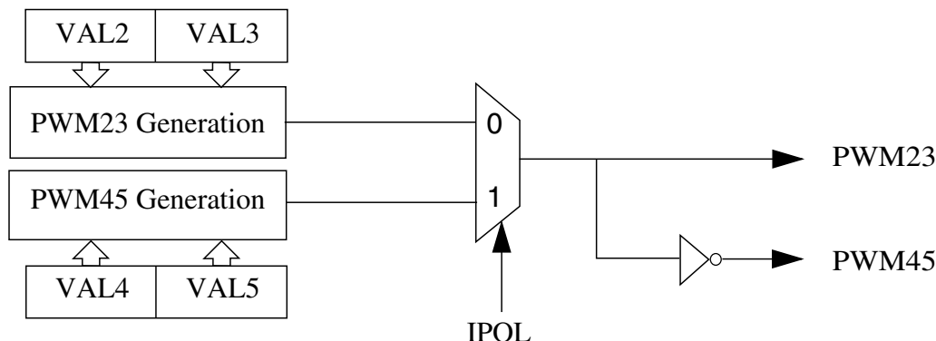
Figure 50-20. Complementary Channel Pair
