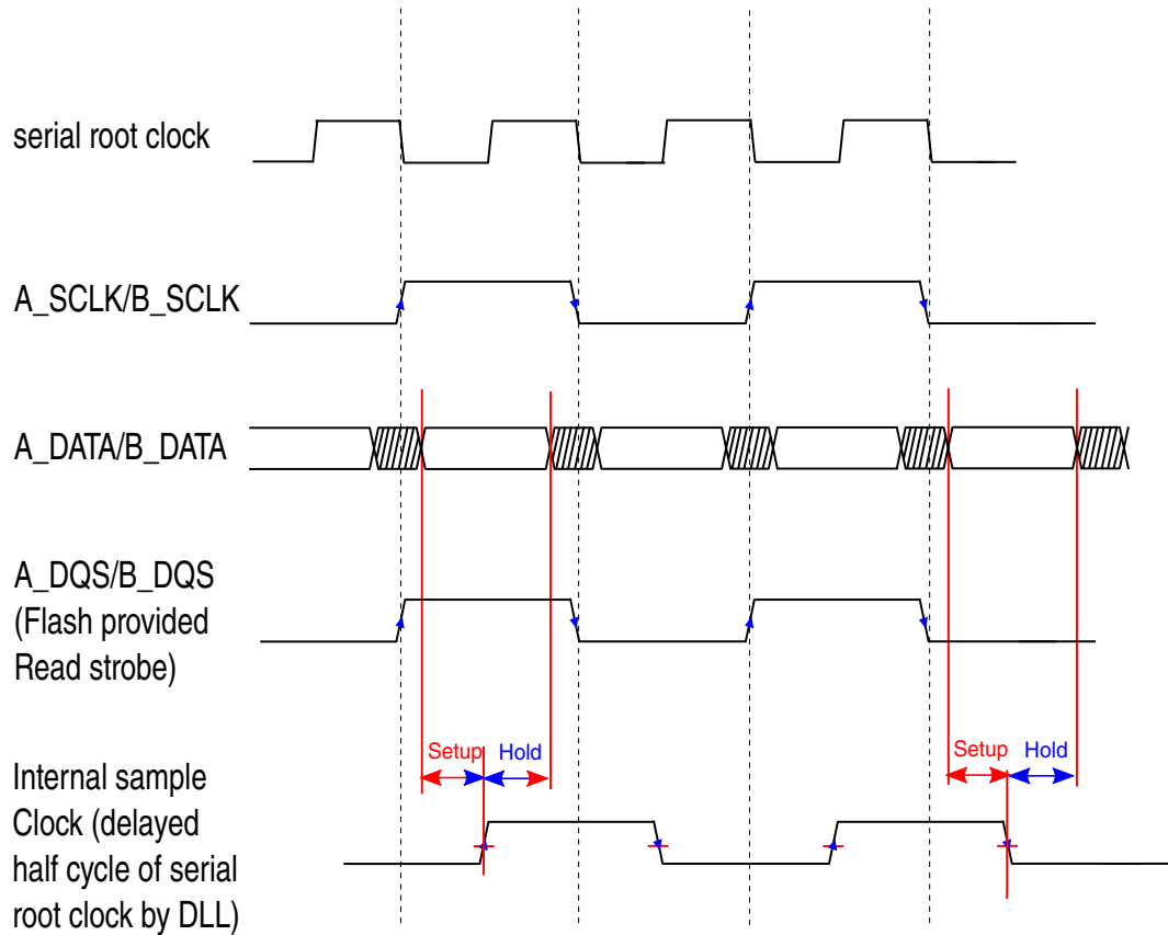
Figure 27-28. Input Timing 2 for Flash provided read strobe in DDR mode
