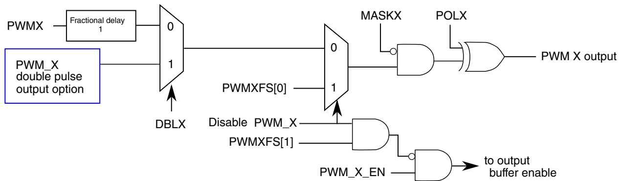
Figure 50-28. Output Logic continued
