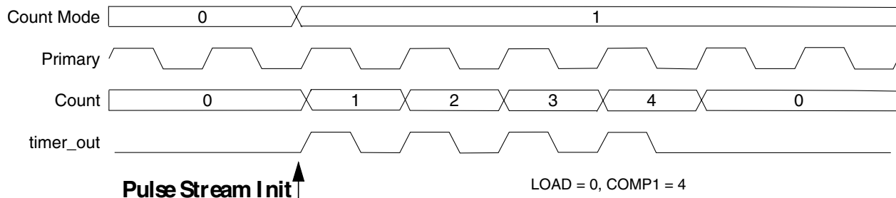
Figure 49-7. Pulse Output Mode
