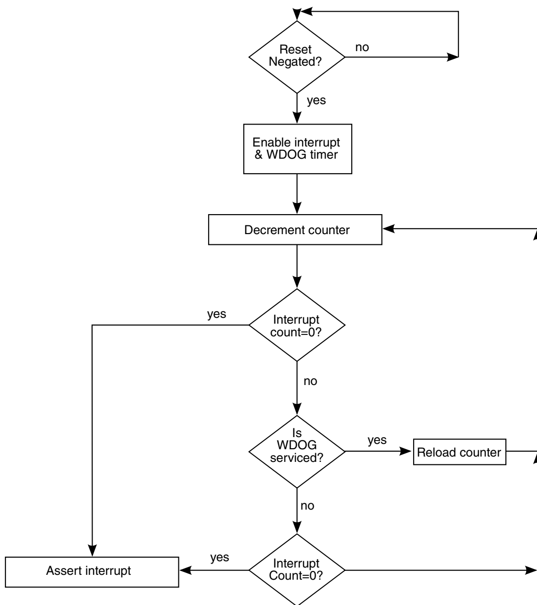
Figure 52-6. Interrupt Generation Flow Diagram
