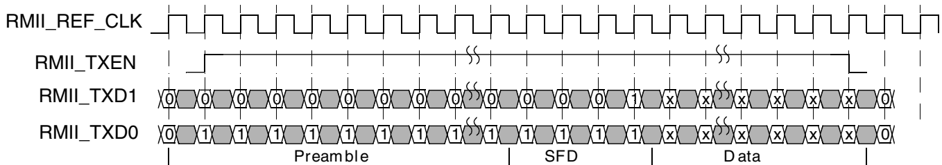
Figure 37-21. RMII transmit operation
