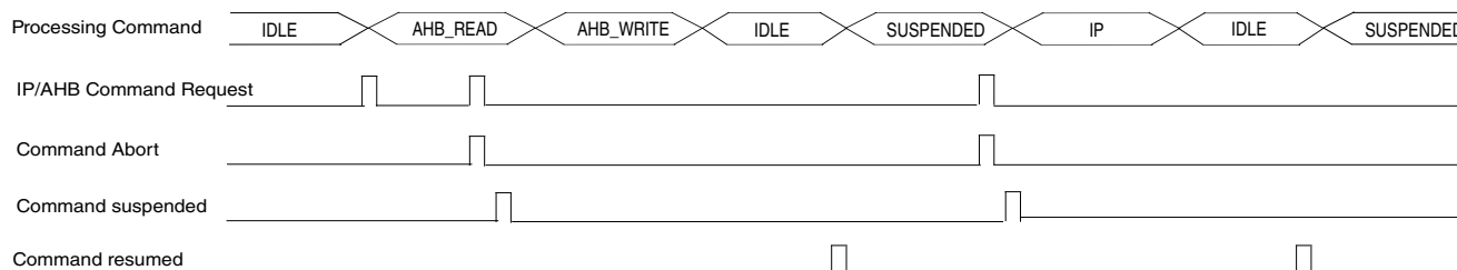
Figure 27-18. Command Instructions Execution on FlexSPI interface
