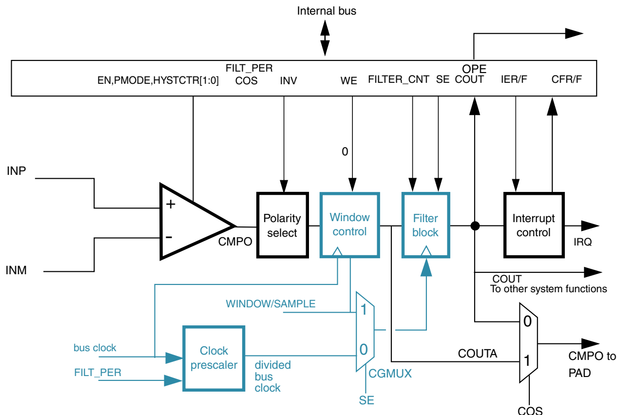
Figure 60-3. Comparator operation in Continuous mode
