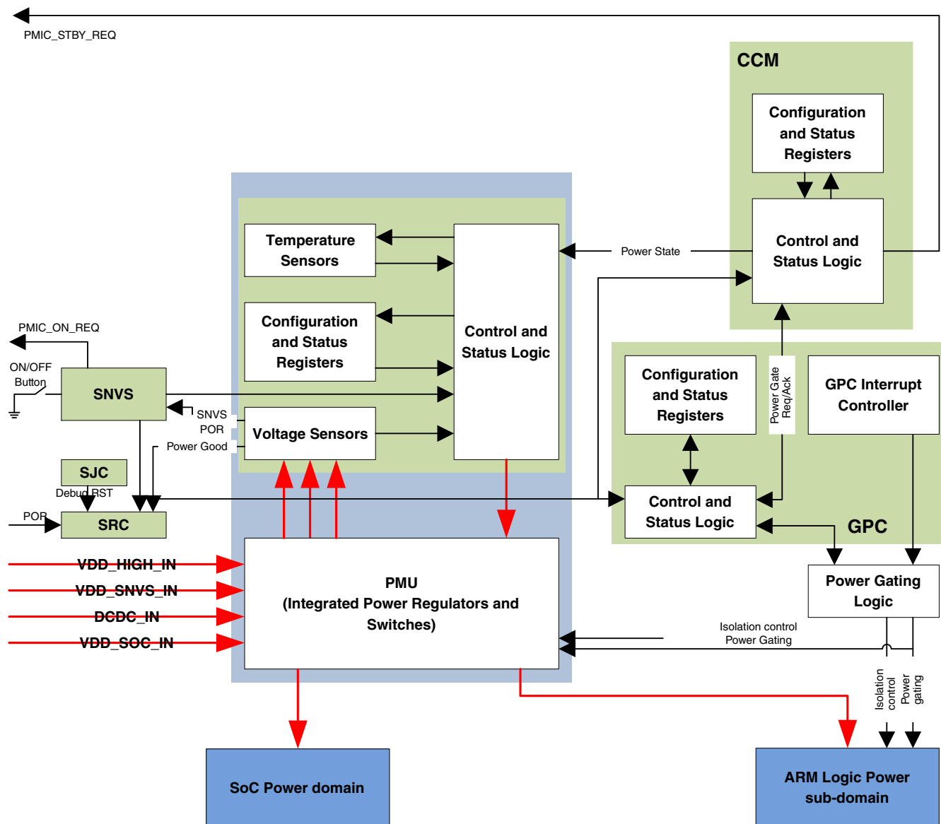
Figure 13-3. Power Management System
