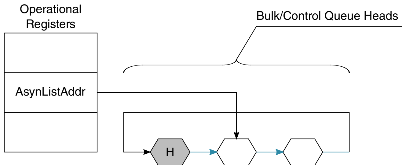
Figure 38-3. Asynchronous Schedule Organization
