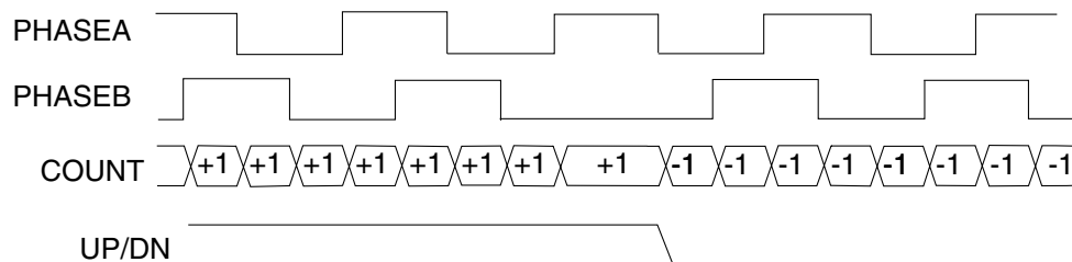
Figure 49-3. Quadrature Incremental Position Encoder
