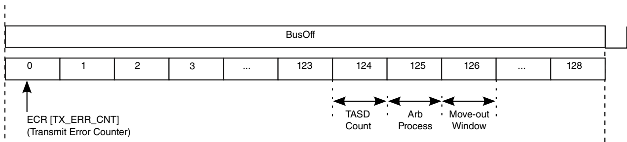
Figure 40-5. Arbitration at the end of Bus Off and Move-Out Time Windows
