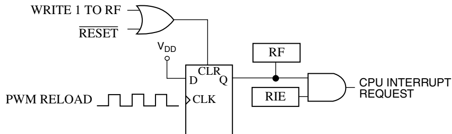
Figure 50-37. PWMF Reload Interrupt Request
