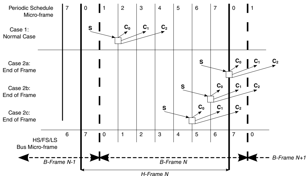
Figure 38-20. Split Transaction, Interrupt Scheduling Boundary Conditions
