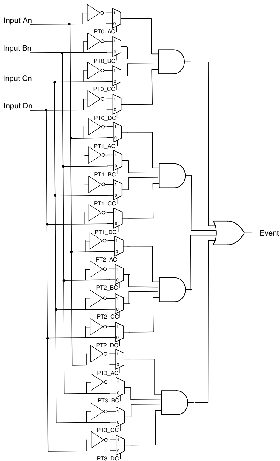
Figure 58-1. Simplified AOI Block Diagram
