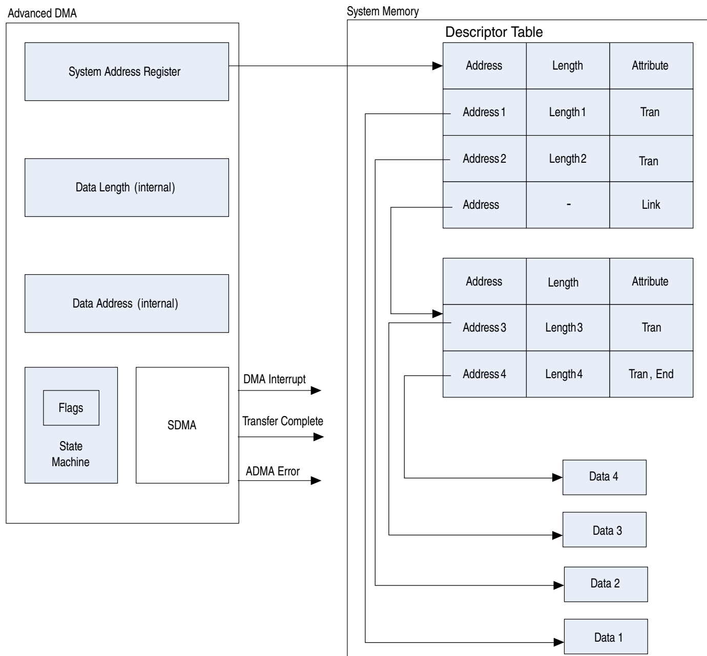
Figure 26-11. Concept and access method of the ADMA2 descriptor table
