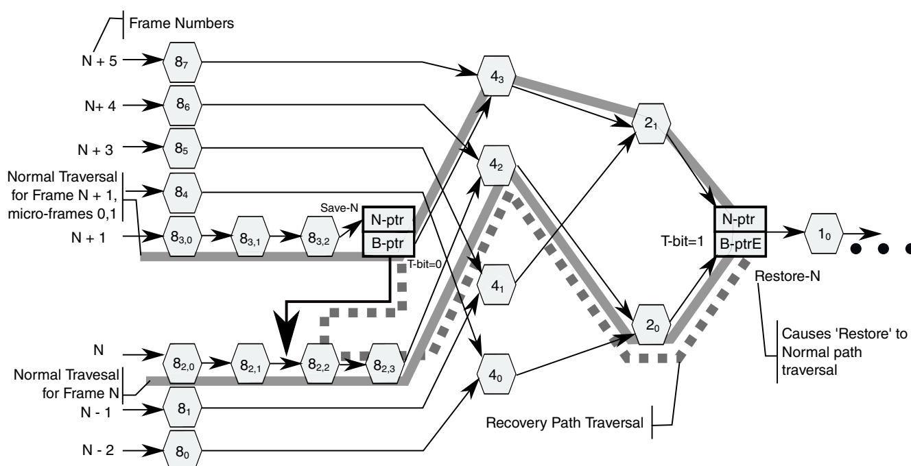
Figure 38-22. Example Host Controller Traversal of Recovery Path via FSTNs
