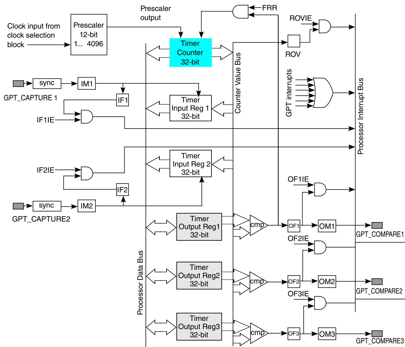
Figure 47-1. GPT Block Diagram
