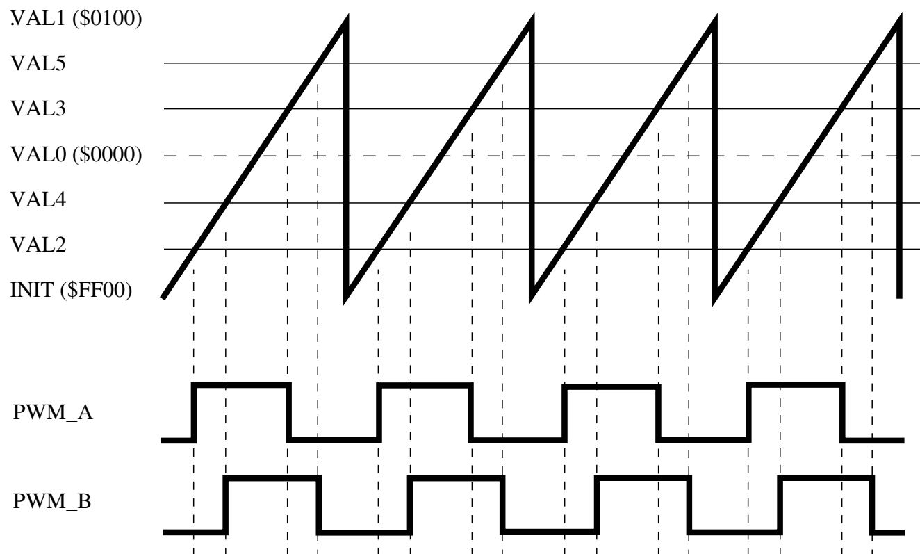
Figure 50-5. Phase Shifted Outputs Example
