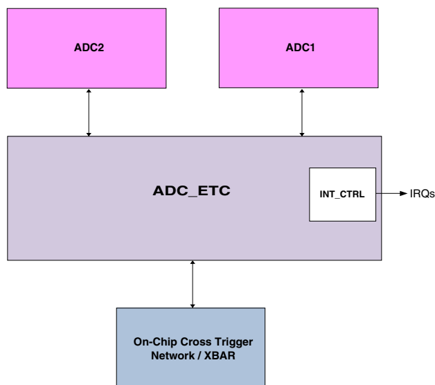
Figure 59-1. Block Diagram (Simplified)
