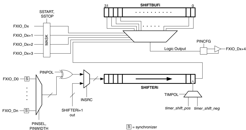
Figure 45-4. Logic Microarchitecture
