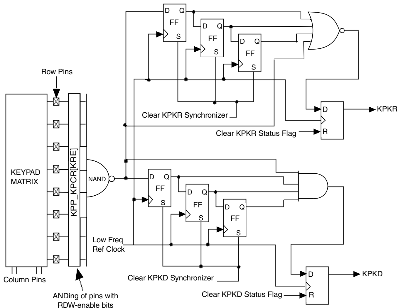
Figure 41-2. Keypad Synchronizer Functional Diagram
