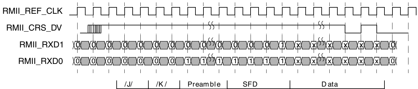
Figure 37-19. RMII receive operation
