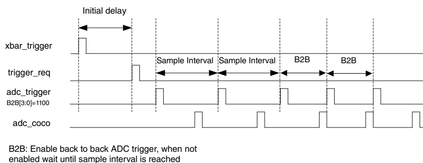
Figure 62-3. ETC-ADC interface timing
