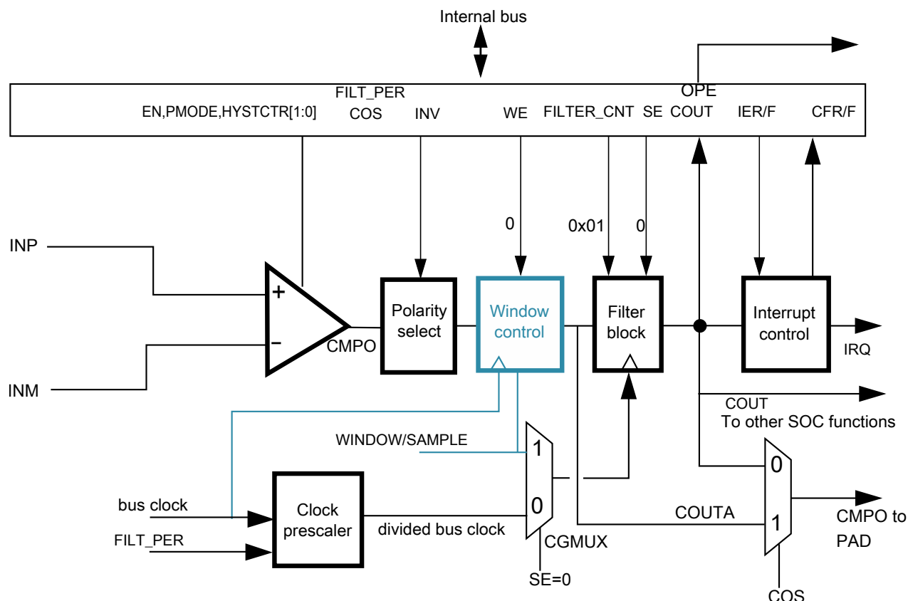
Figure 60-5. Sampled, Non-Filtered (# 3B): sampling interval internally derived
