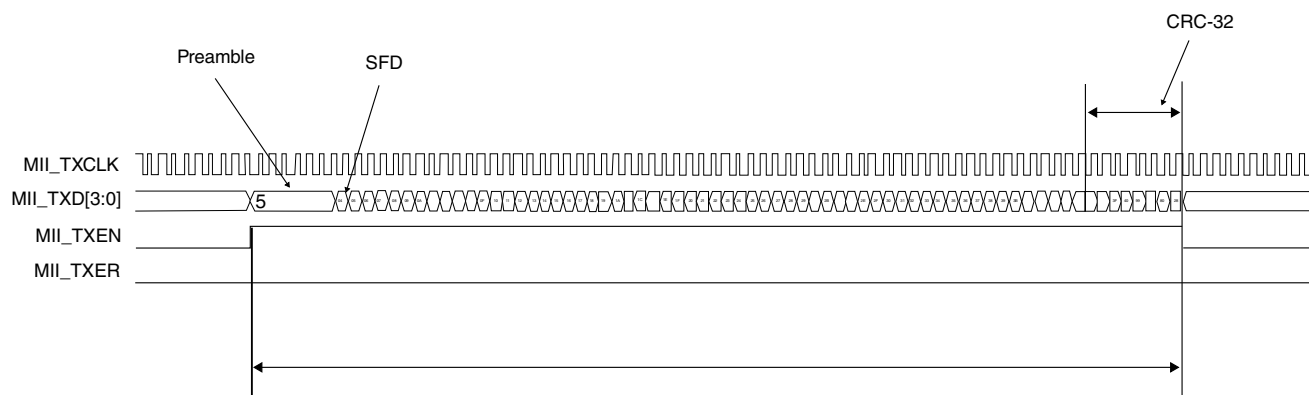
Figure 37-22. MII transmit operation
