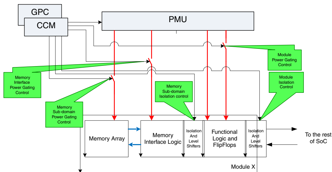
Figure 13-5. Power domain interface
