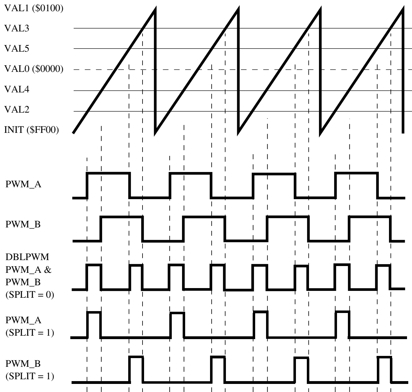
Figure 50-7. Double Switching Output Example
