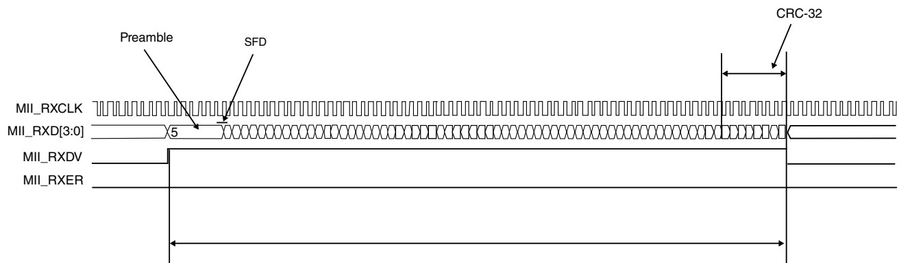
Figure 37-25. MII receive operation
