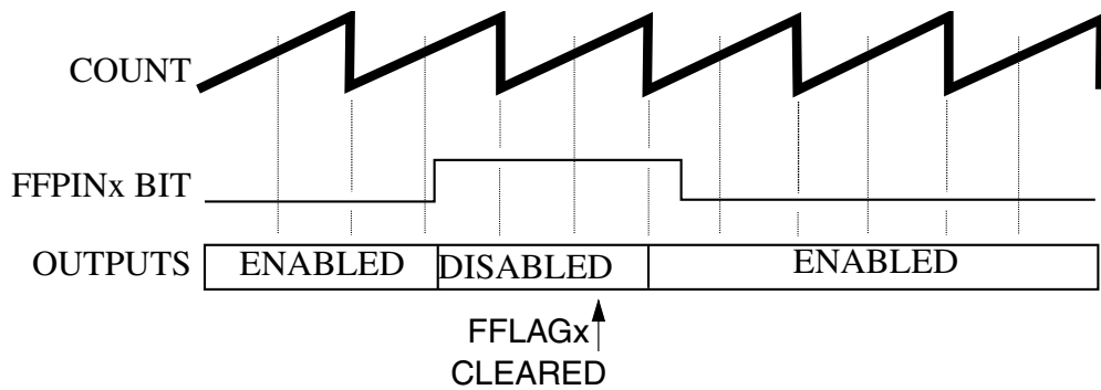
Figure 50-32. Manual Fault Clearing (FCTRL[FSAFE]=0)
