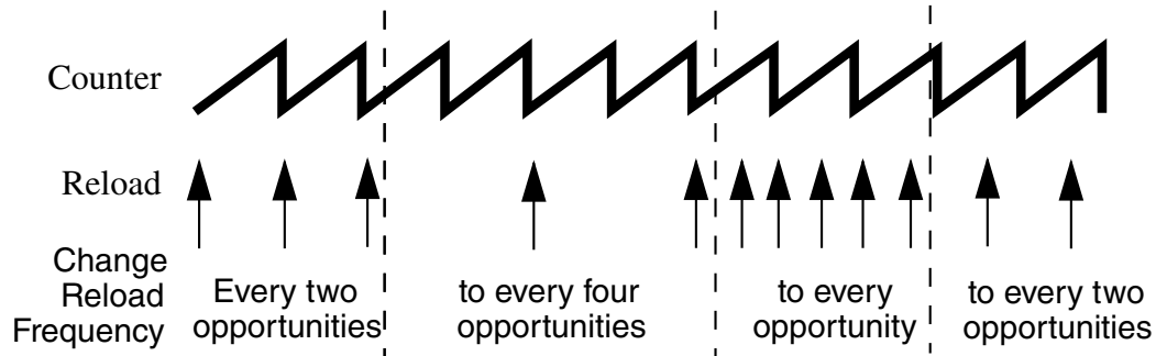
Figure 50-36. Full and Half Cycle Reload Frequency Change
