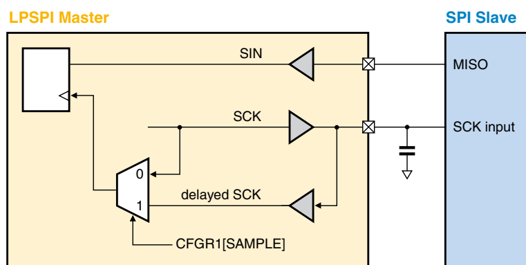
Figure 43-3. Clock loopback
