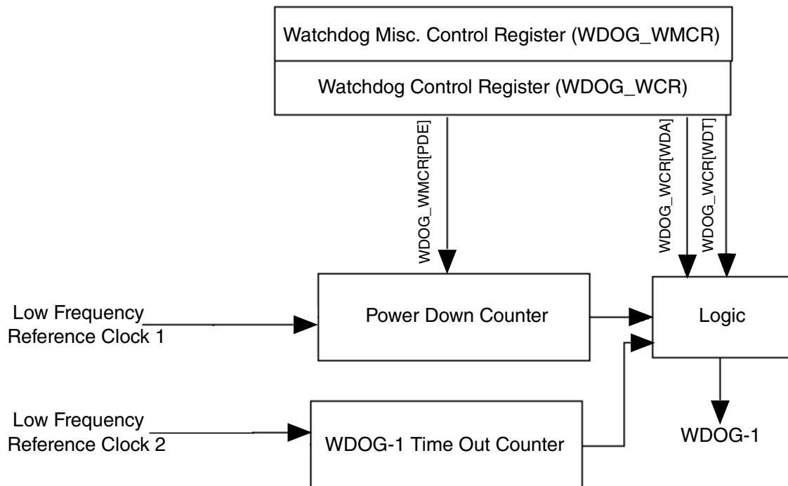
Figure 52-2. WDOG_B (ipp_wdog) generation
