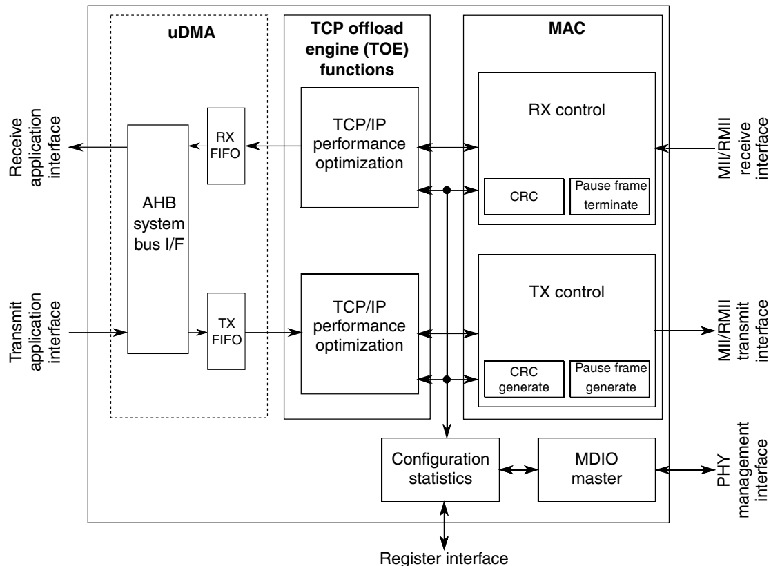
Figure 37-1. Ethernet MAC-NET core block diagram
