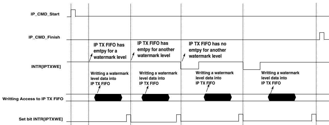
Figure 27-11. Filling IP TX FIFO by processor
