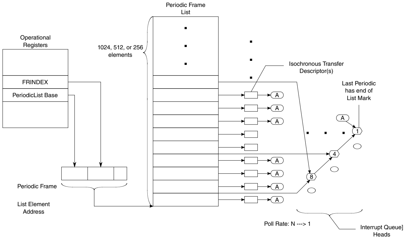
Figure 38-2. Periodic Schedule Organization
