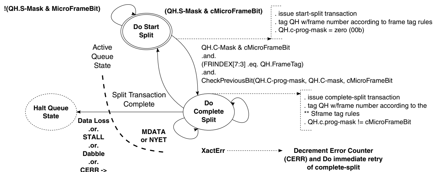
Figure 38-23. Split Transaction State Machine for Interrupt
