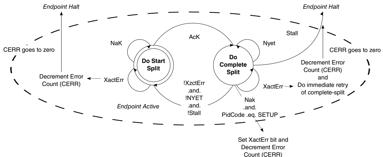
Figure 38-19. Host Controller Asynchronous Schedule Split-Transaction State Machine
