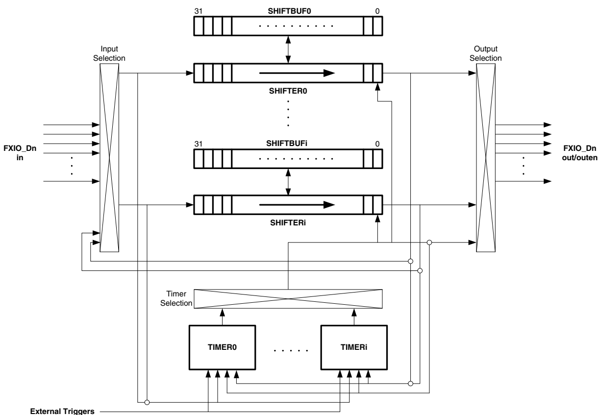
Figure 45-1. FlexIO block diagram
