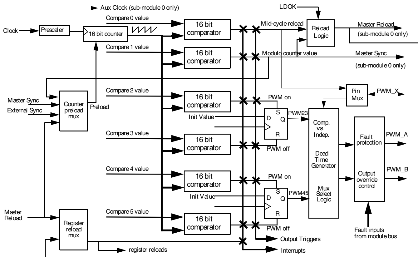
Figure 50-2. PWM Submodule Block Diagram
