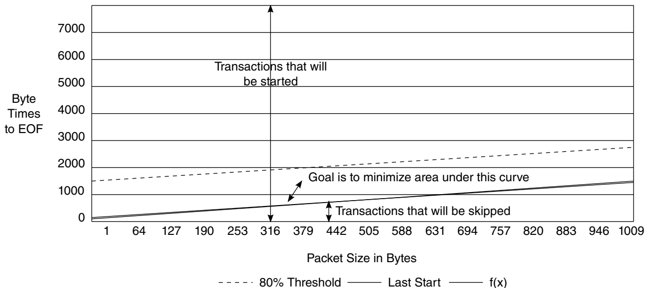
Figure 38-8. Best Fit Approximation
