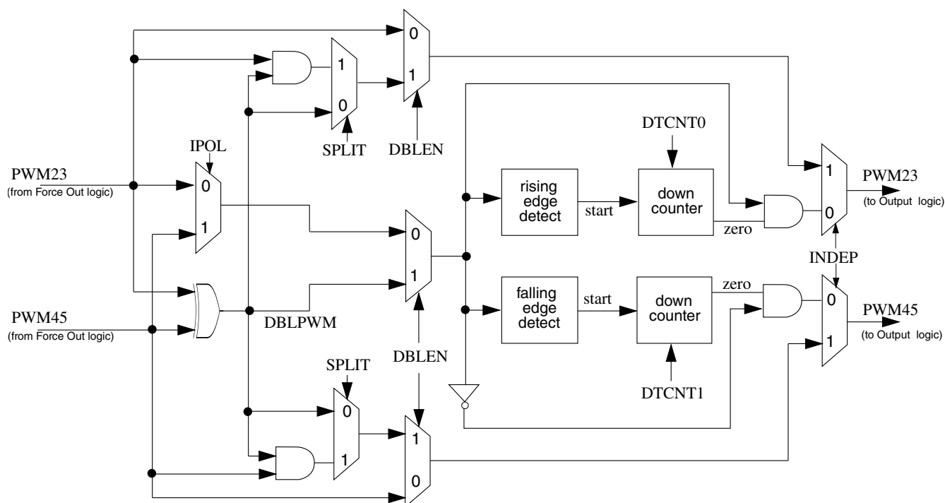
Figure 50-22. Deadtime Insertion Logic
