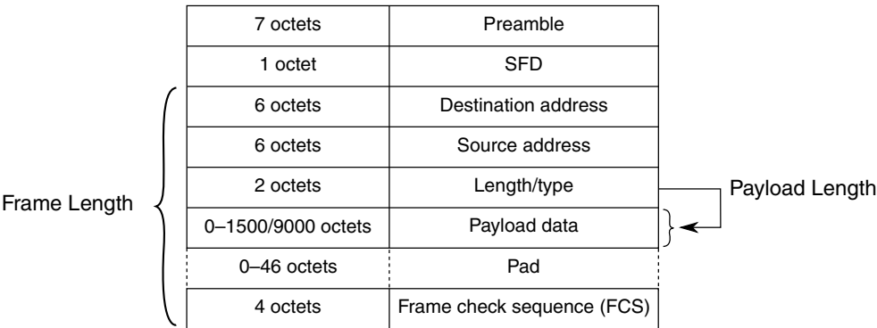
Figure 37-2. MAC frame format overview
