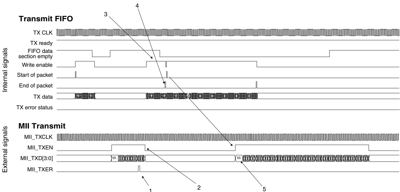
Figure 37-16. Transmit FIFO underflow protection
