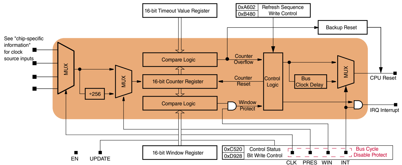
Figure 53-1. WDOG block diagram
