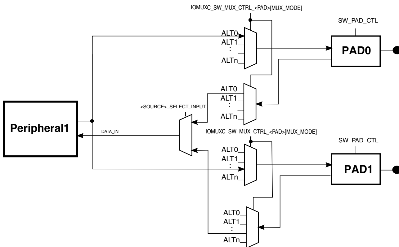
Figure 11-2. IOMUX Cell Block Diagram
