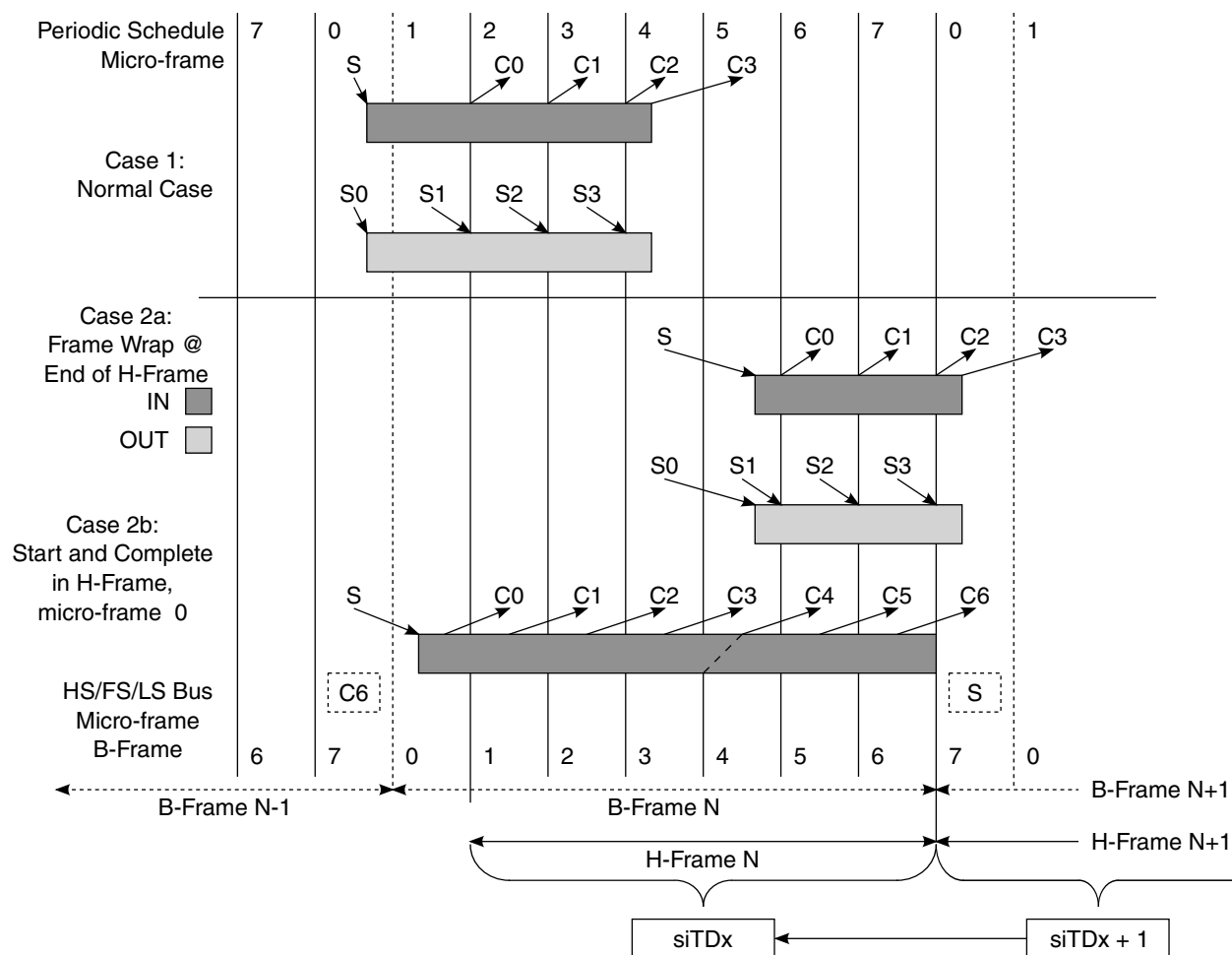
Figure 38-24. Split Transaction, Isochronous Scheduling Boundary Conditions
