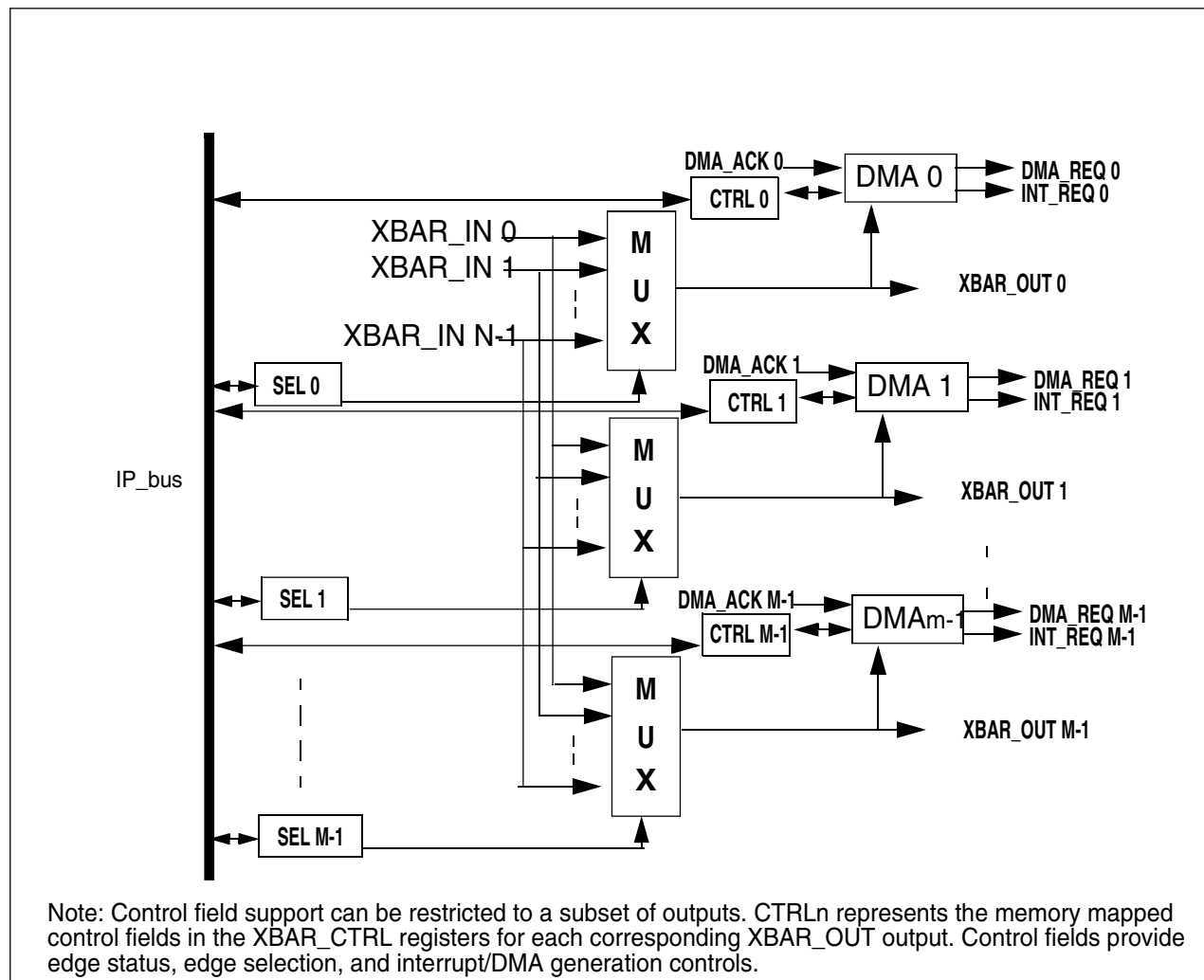
Figure 56-1. XBAR Block Diagram
