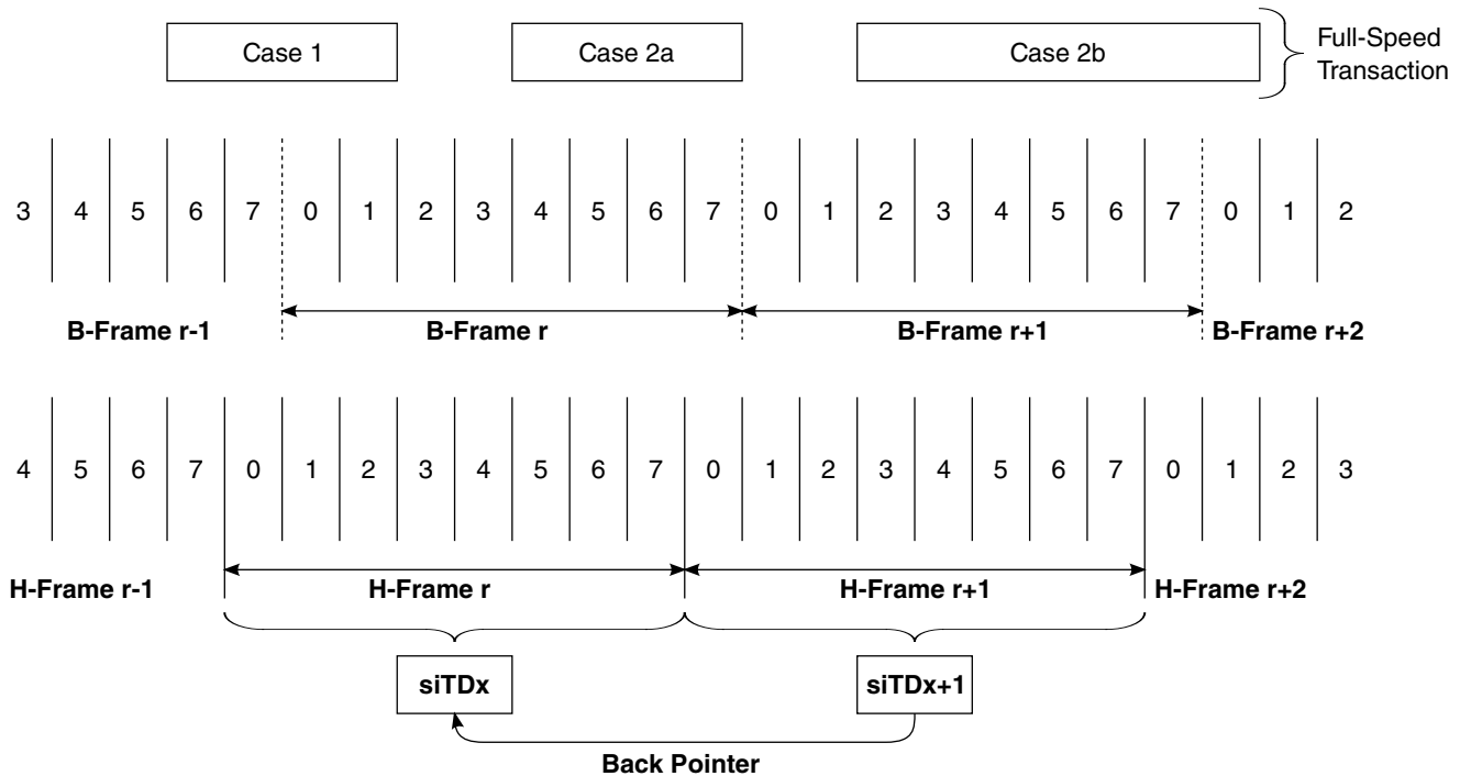
Figure 38-25. siTD Scheduling Boundary Examples
