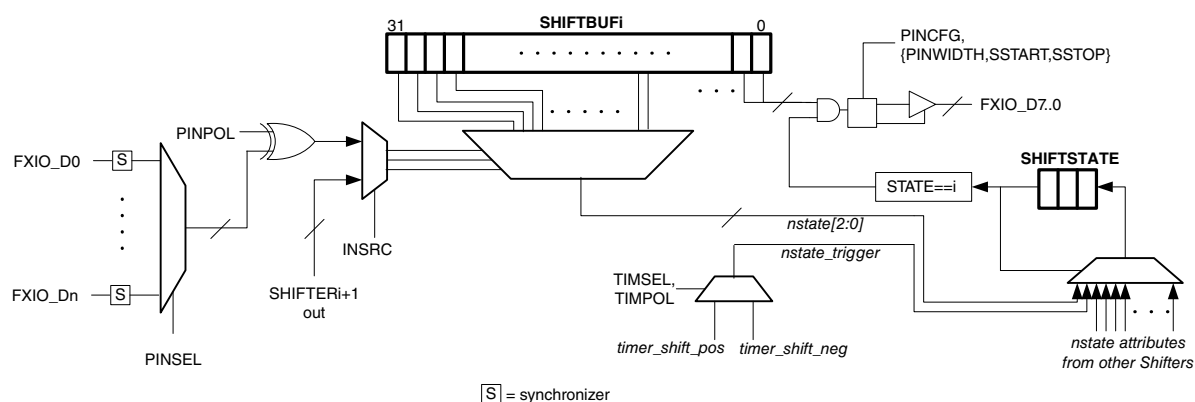
Figure 45-3. State Microarchitecture
