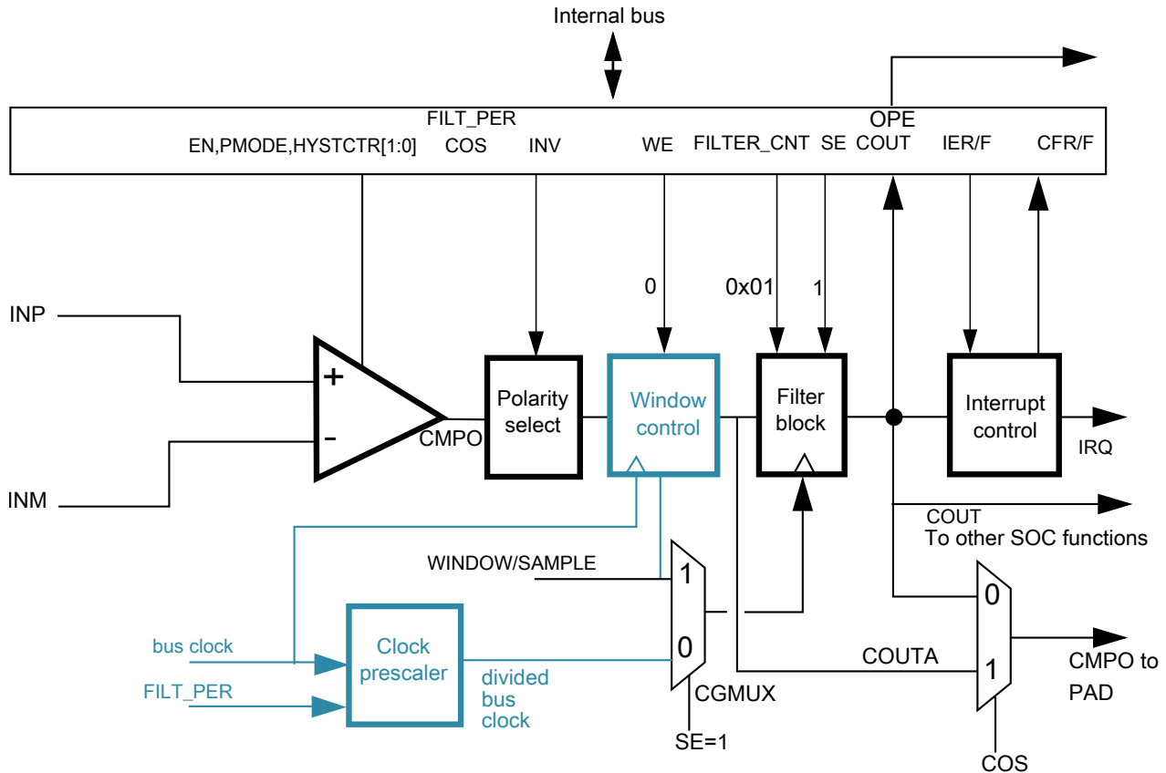
Figure 60-4. Sampled, Non-Filtered (# 3A): sampling point externally driven
