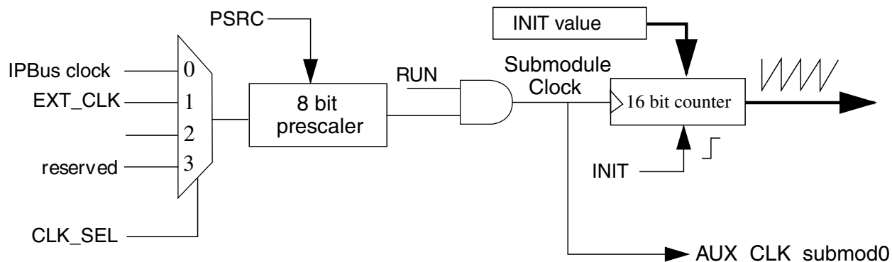
Figure 50-14. Clocking Block Diagram for PWM Submodule 0
