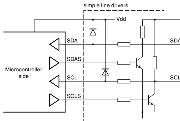
Figure 42-3. I²C 4-wire serial bus
