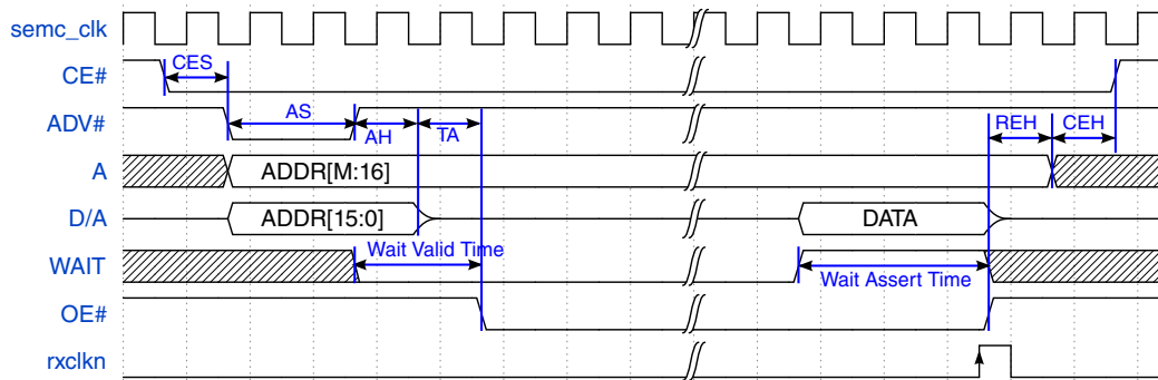
Figure 25-60. SRAM Read in ASYNC Mode (ADMUX) with Wait Pin
