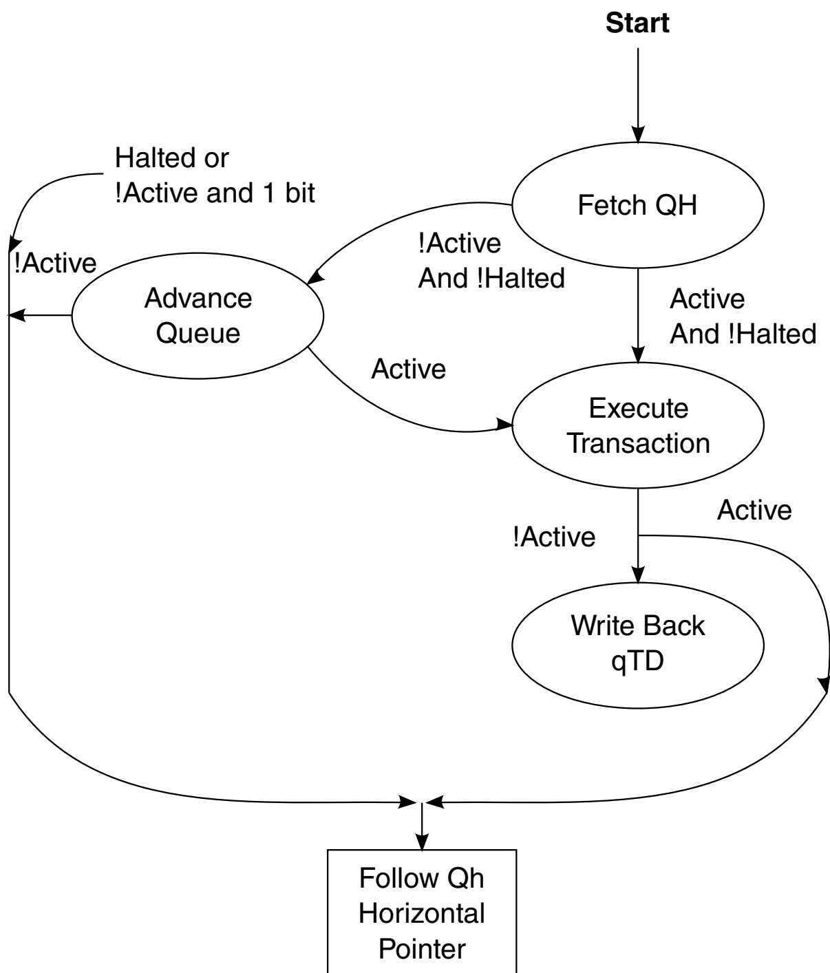
Figure 38-17. Host Controller Queue Head Traversal State Machine
