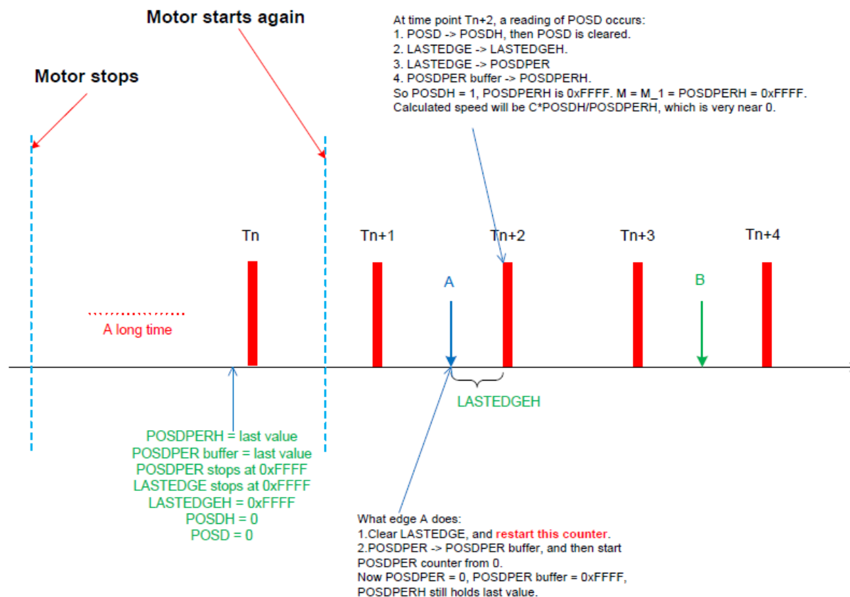
Figure 51-13. Speed measurement at time point T_{n+2}
