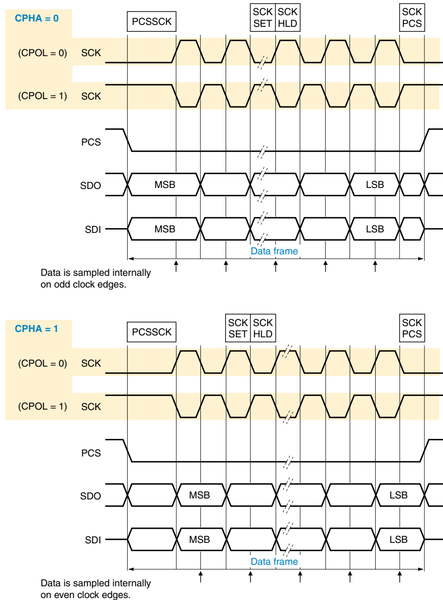
Figure 43-2. Clock Phase (TCR[CPHA]) timing diagram example
