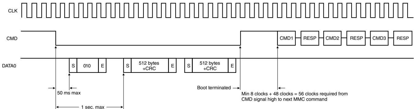
Figure 26-14. MultiMediaCard state diagram (normal boot mode)
