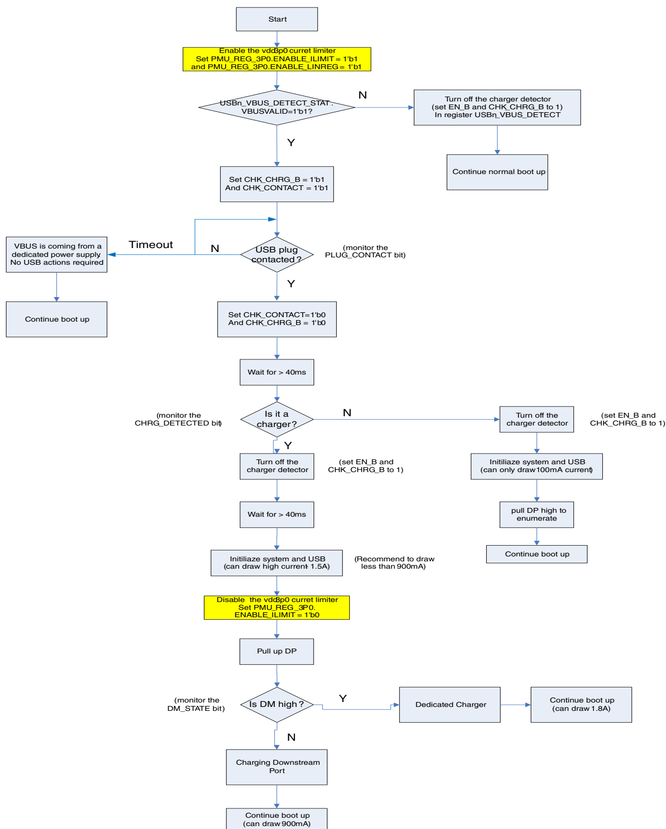
Figure 39-3. USBPHY Charger Detection Software Flow
