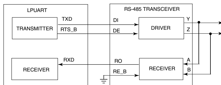
Figure 44-4. Transceiver driver enable using RTS_B
