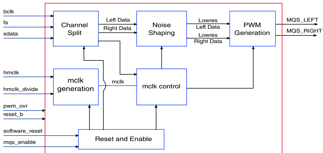
Figure 35-1. Block Diagram
