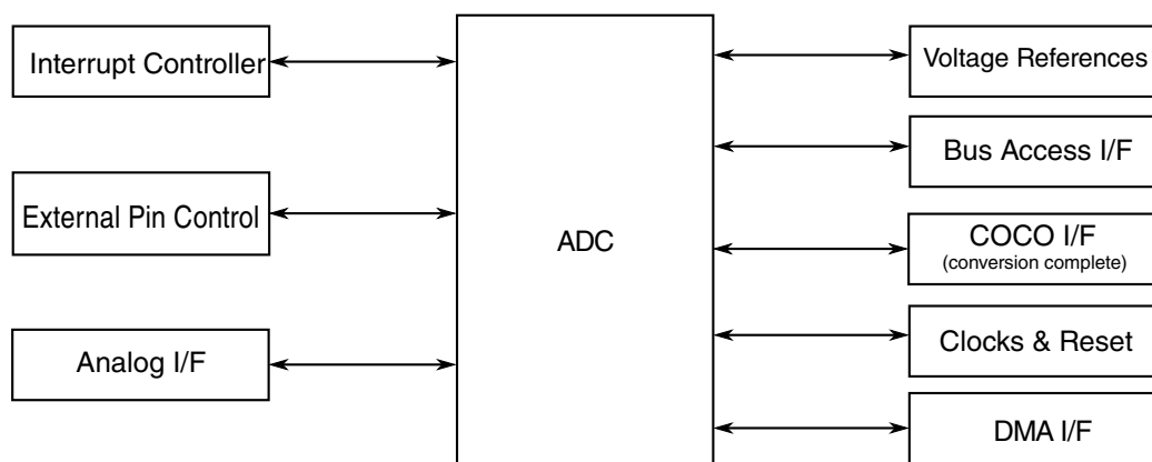
Figure 61-3. ADC module interface
