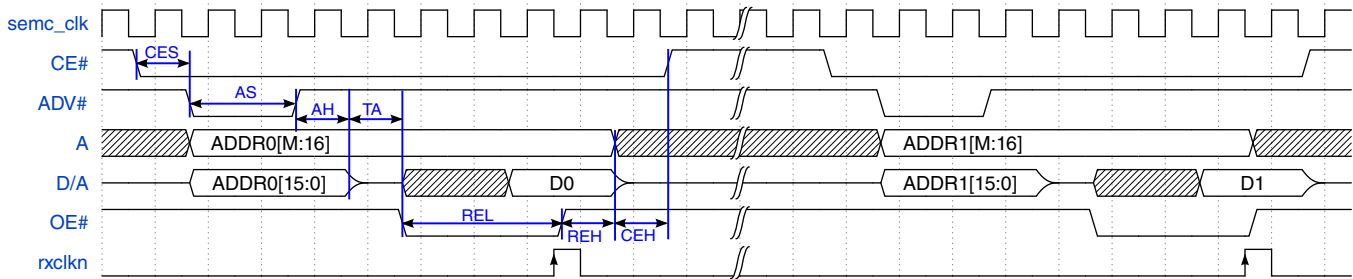
Figure 25-55. ASYNC SRAM Read in ADMUX Address Mode
