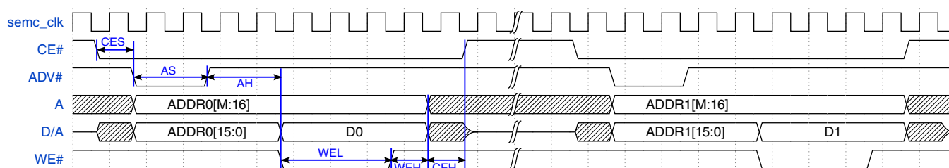
Figure 25-52. ASYNC NOR Flash Write in ADMUX Address Mode
