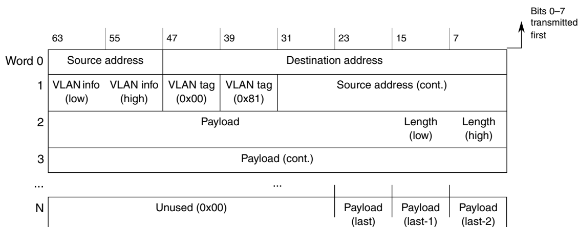
Figure 37-15. VLAN-tagged frame 64-bit mapping example
