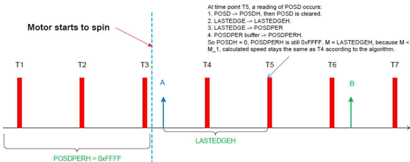
Figure 51-9. Speed measurement at time point T5
