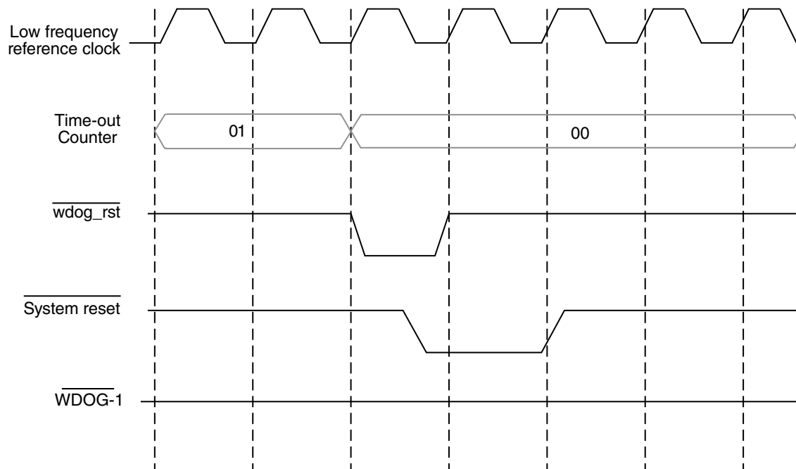
Figure 52-3. WDOG timeout condition/WDT bit is not set
