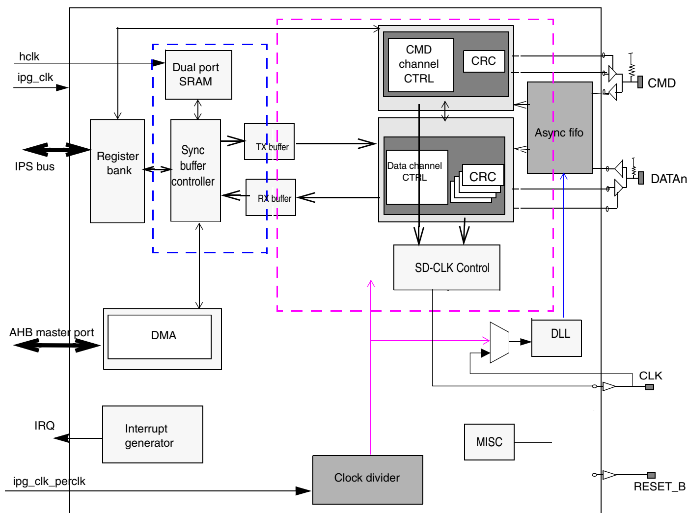
Figure 26-1. uSDHC block diagram
