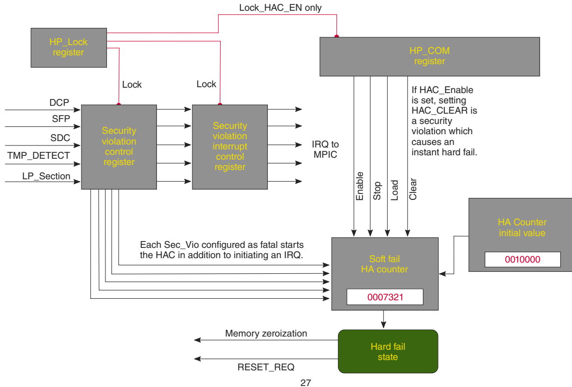
Figure 20-3. Relationship Between the Registers
