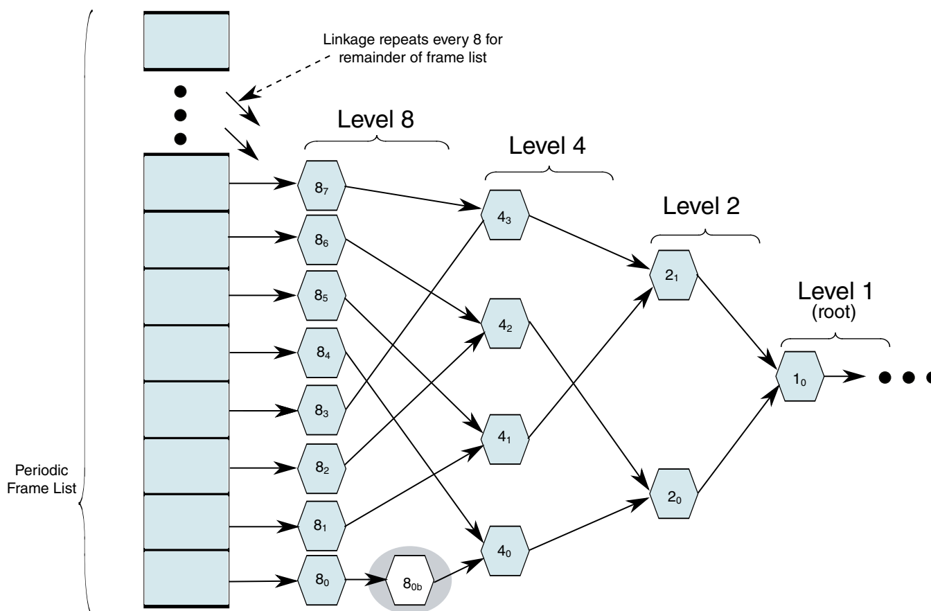
Figure 38-21. General Structure of EHCI Periodic Schedule Utilizing Interrupt Spreading
