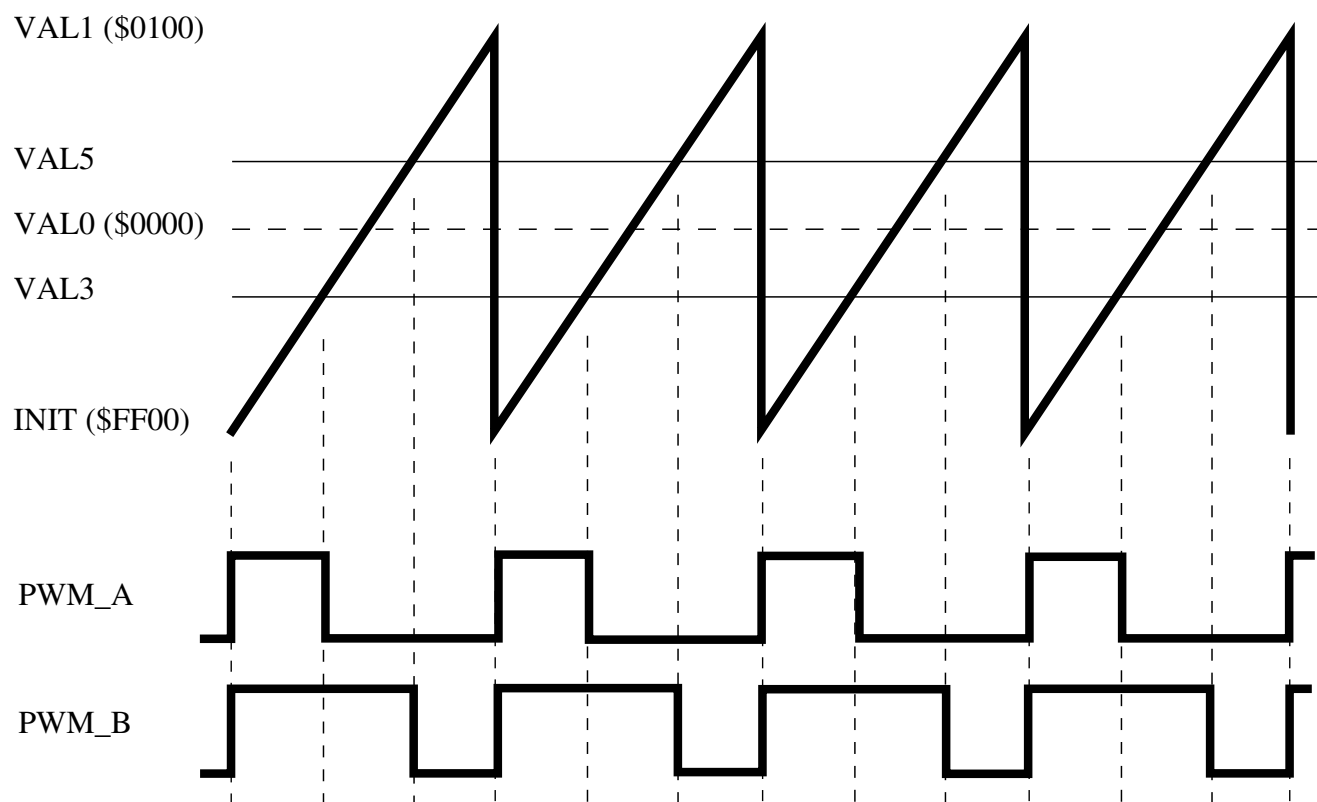
Figure 50-4. Edge Aligned Example (INIT=VAL2=VAL4)
