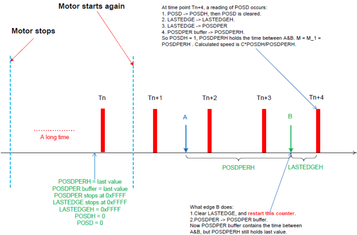
Figure 51-15. Speed measurement at time point Tn+4
