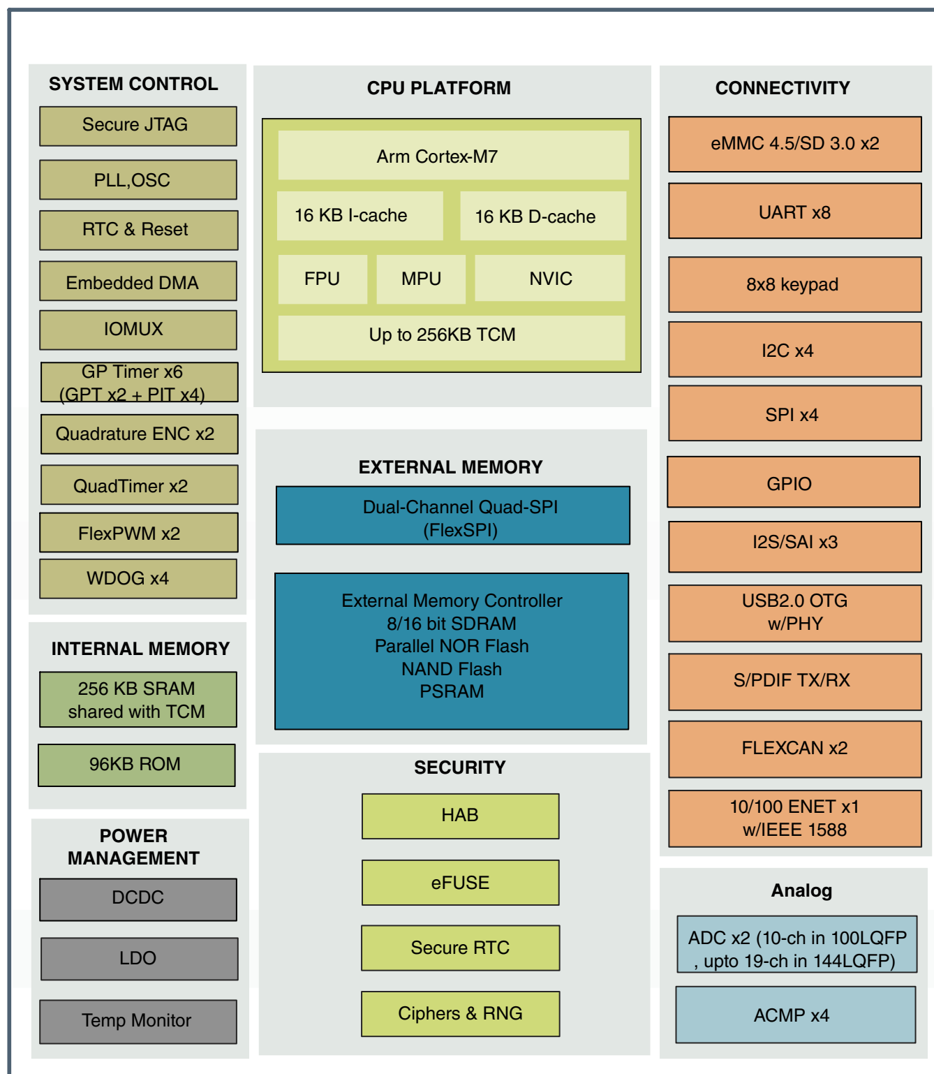
Figure 2-1. Simplified Block Diagram
