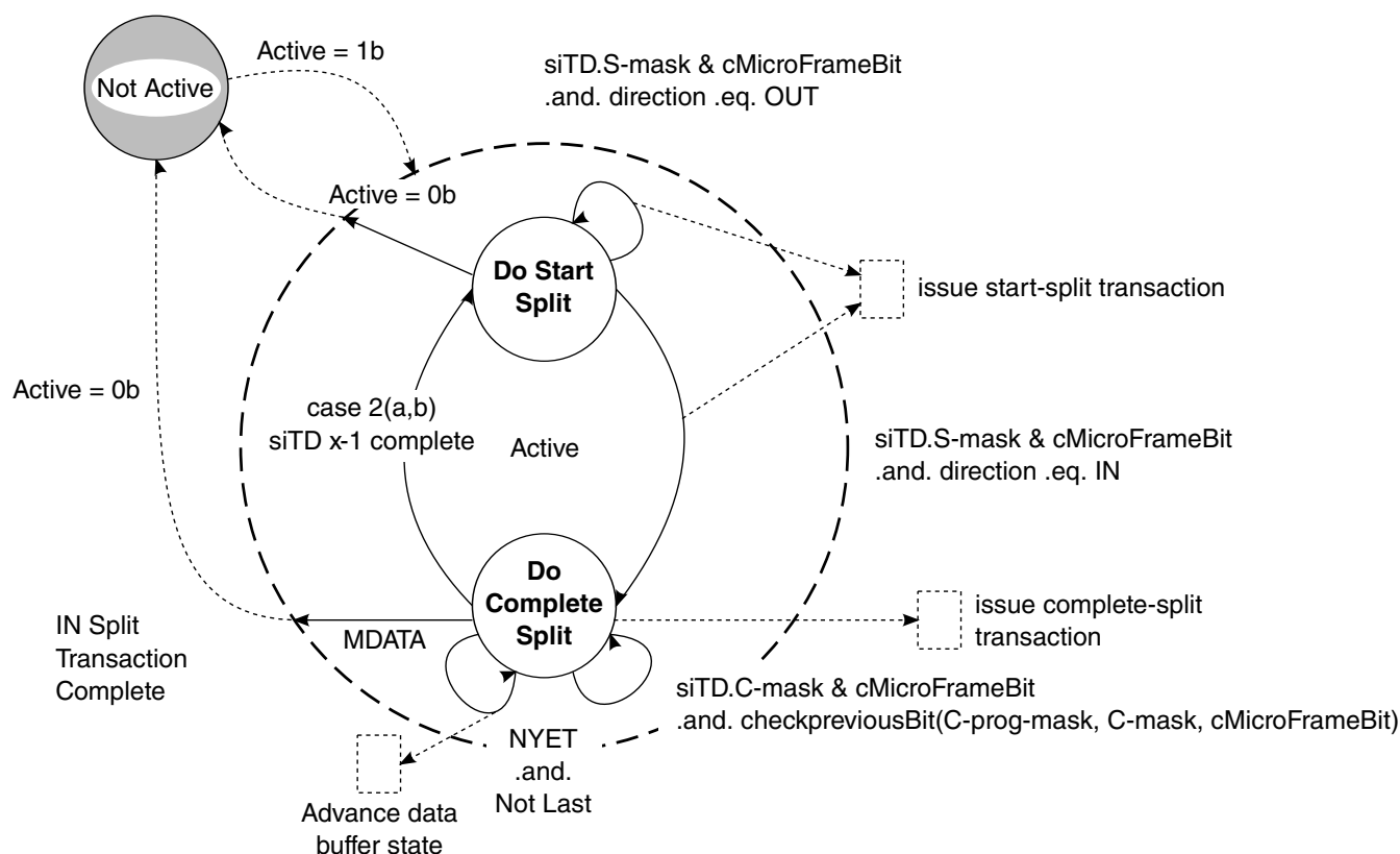
Figure 38-26. Split Transaction State Machine for Isochronous
