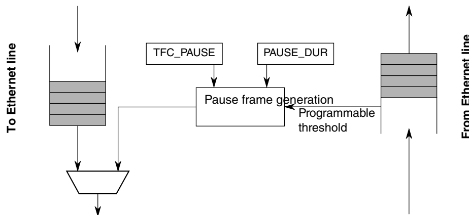
Figure 37-8. Pause frame generation overview
