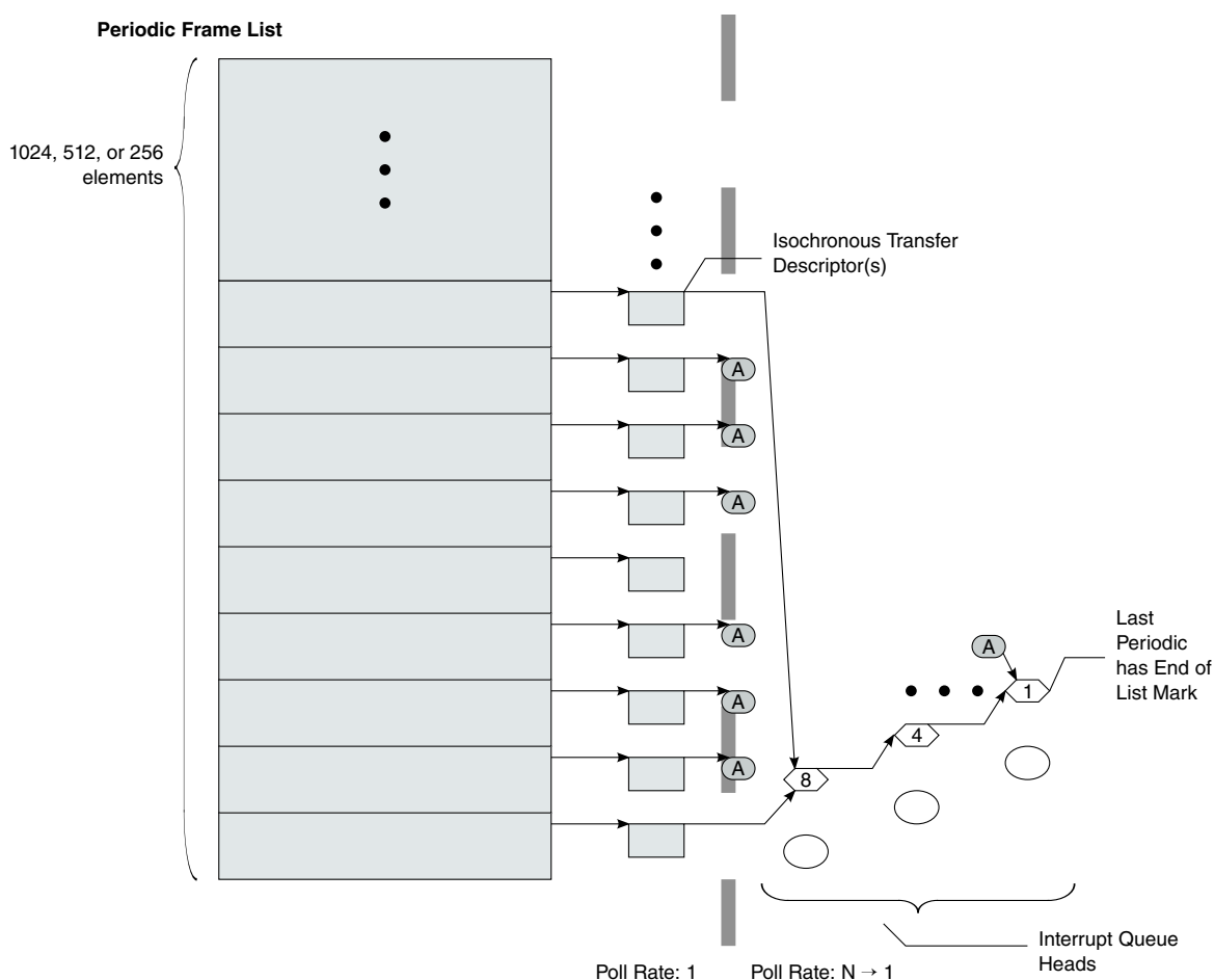
Figure 38-11. Example Periodic Schedule
