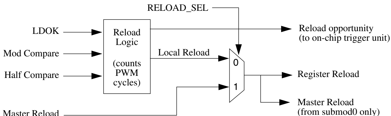
Figure 50-16. Register Reload Logic
