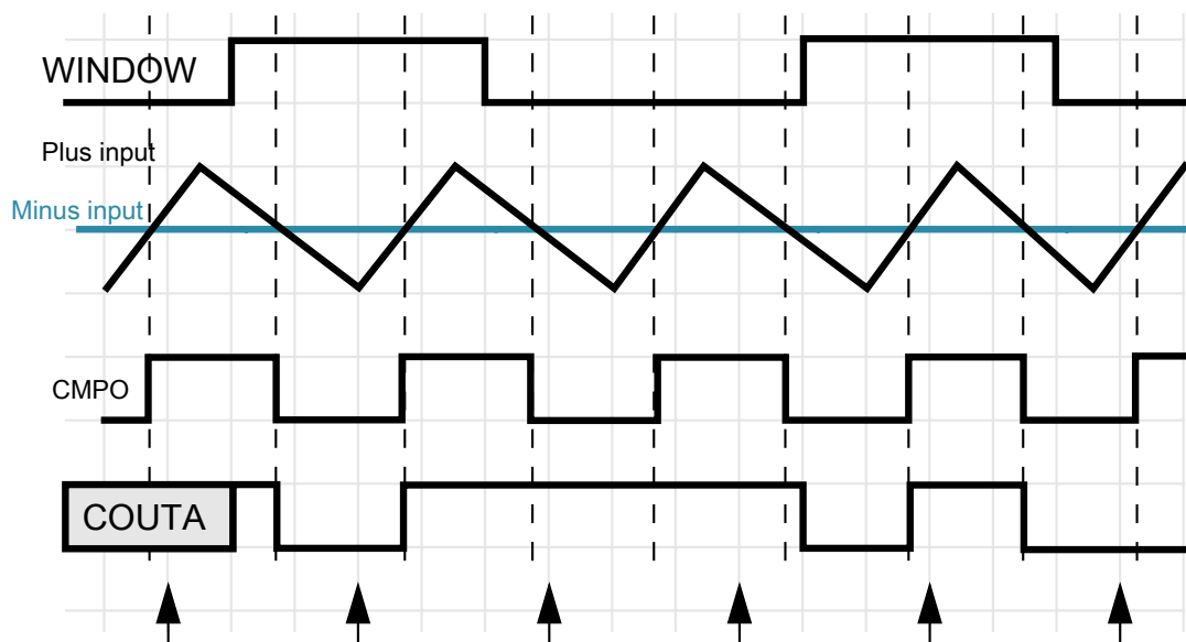
Figure 60-8. Windowed mode operation
