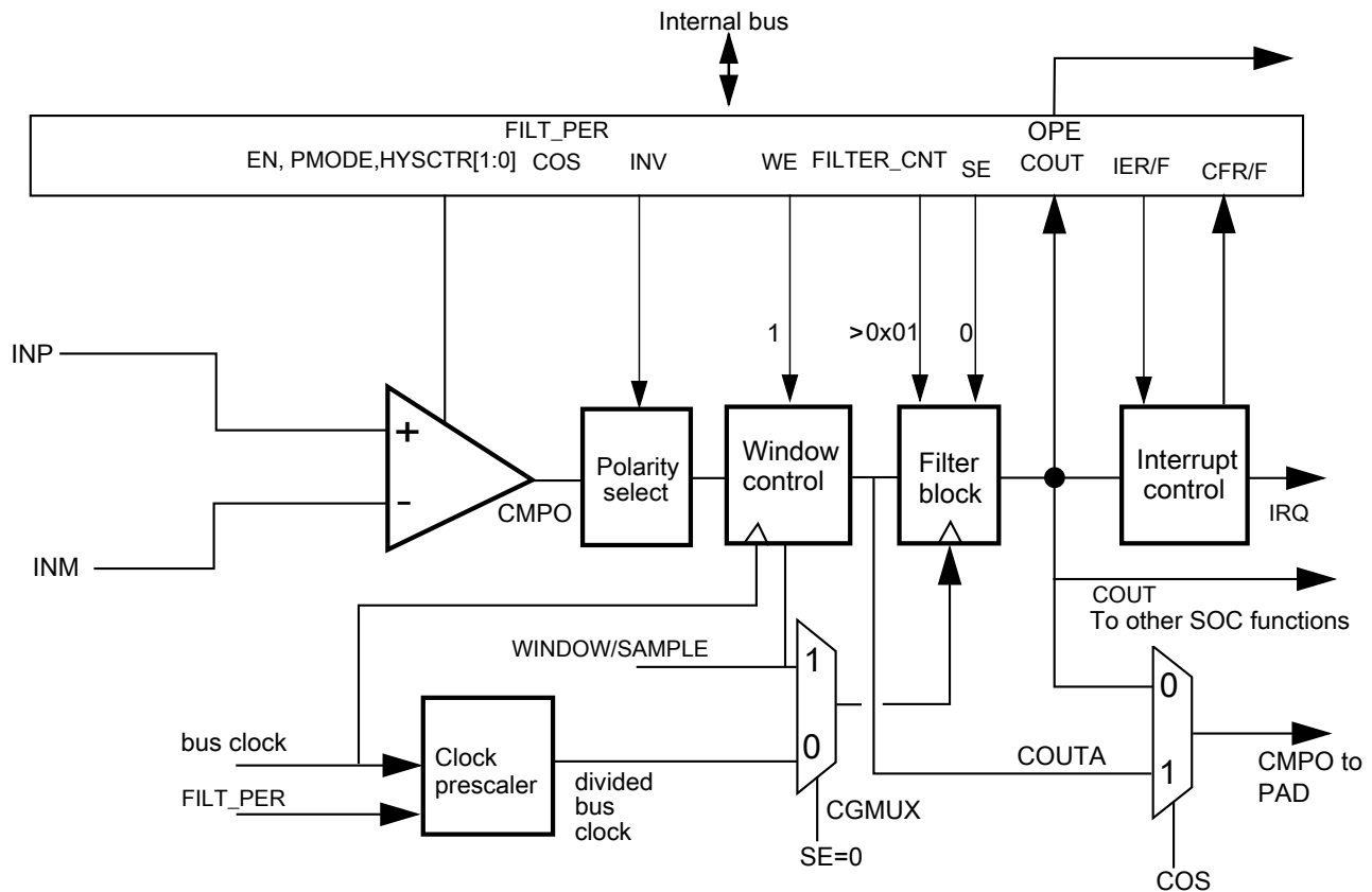
Figure 60-11. Windowed/Filtered mode
