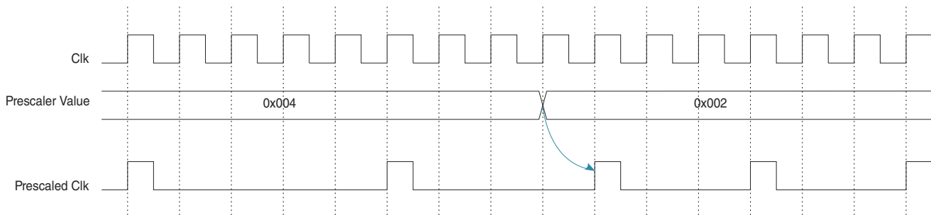
Figure 47-3. Prescaler Value Change Timing Diagram
