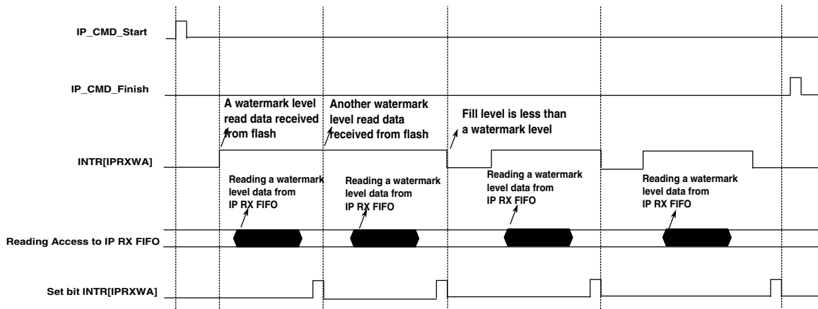
Figure 27-9. Reading IP RX FIFO by processor
