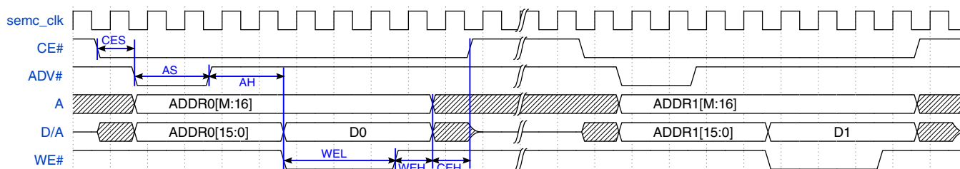
Figure 25-57. ASYNC SRAM Write in ADMUX Address Mode
