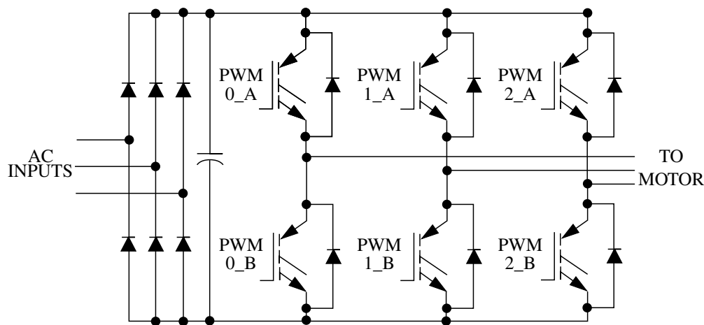
Figure 50-21. Typical 3 Phase AC Motor Drive
