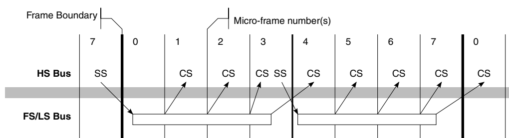
Figure 38-9. Frame Boundary Relationship between HS bus and FS/LS Bus
