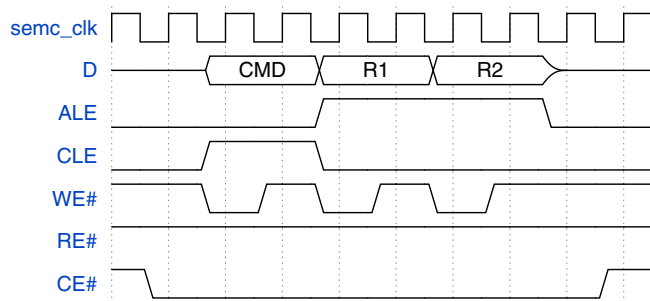
Figure 25-33. NAND Flash Access Address Type - Two Bytes Row Address
