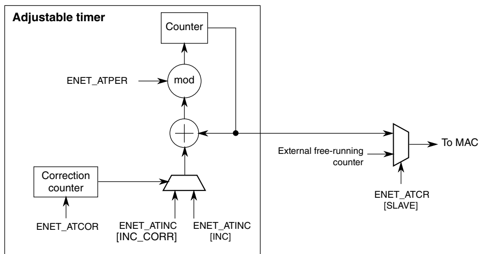
Figure 37-10. Adjustable timer implementation detail
