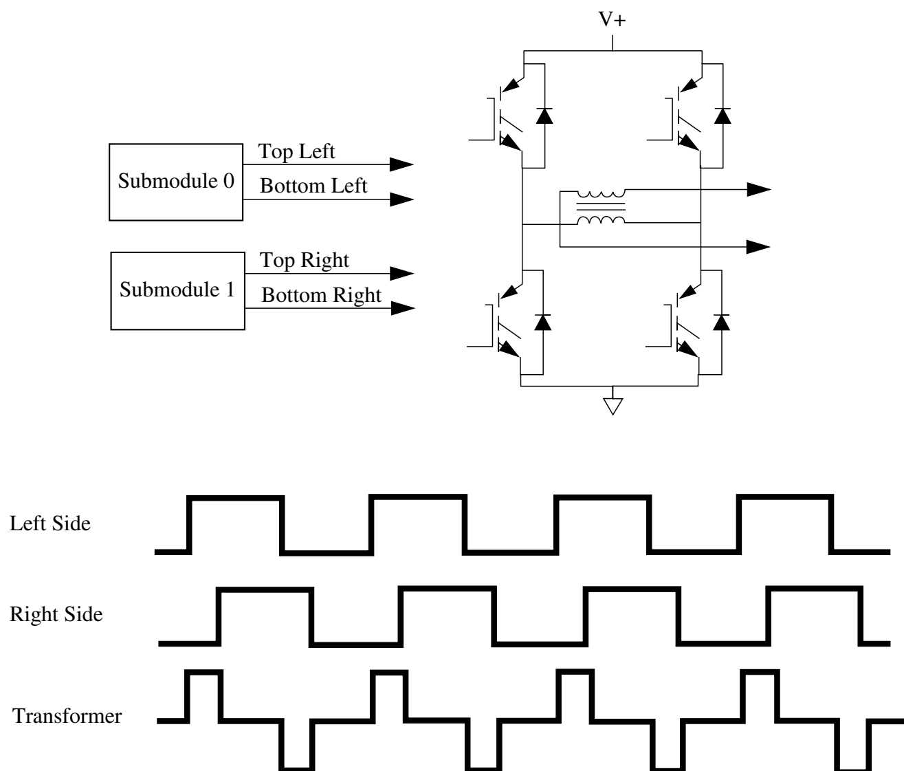
Figure 50-6. Phase Shifted PWMs Applied to a Transformer Primary
