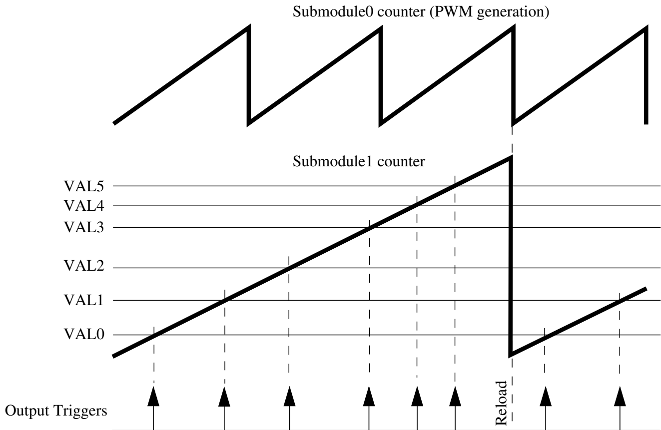
Figure 50-9. Multiple Output Triggers Over Several PWM Cycles
