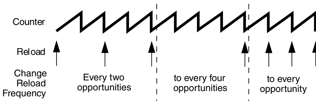
Figure 50-34. Full Cycle Reload Frequency Change
