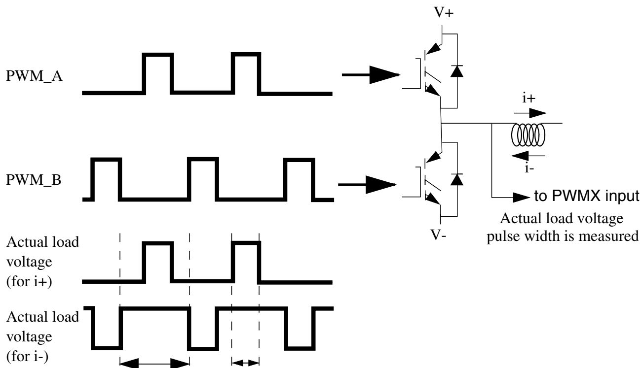
Figure 50-11. Output Pulse Width Measurement Possible with the E-Capture Circuit
