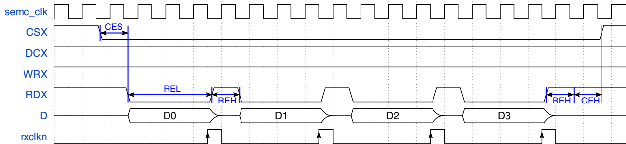
Figure 25-63. DBI Read Operation
