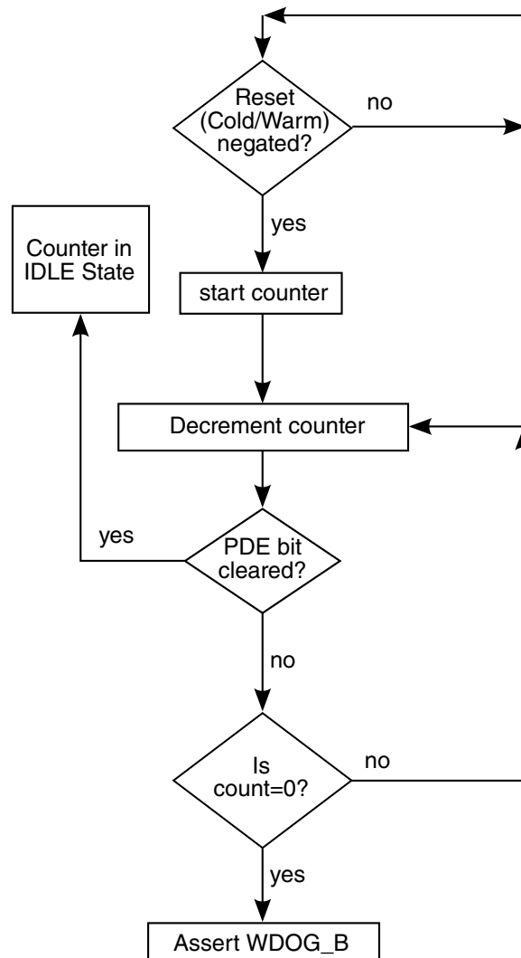
Figure 52-5. Power-Down Counter Flow Diagram
