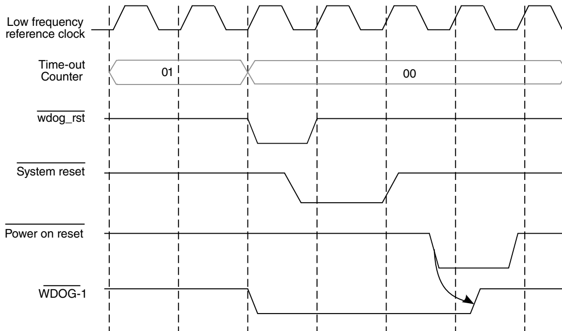
Figure 52-4. WDOG timeout condition/WDT bit is set
