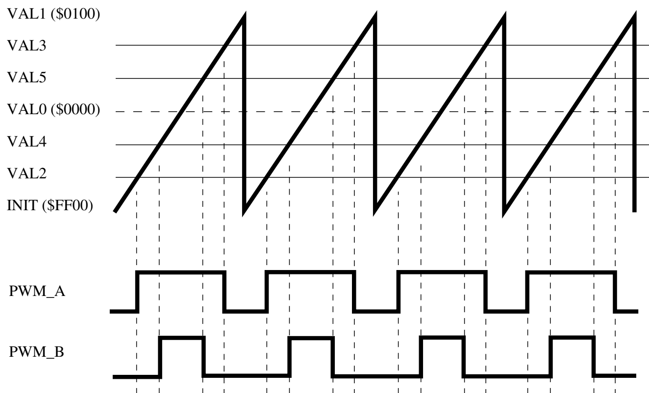
Figure 50-3. Center Aligned Example
