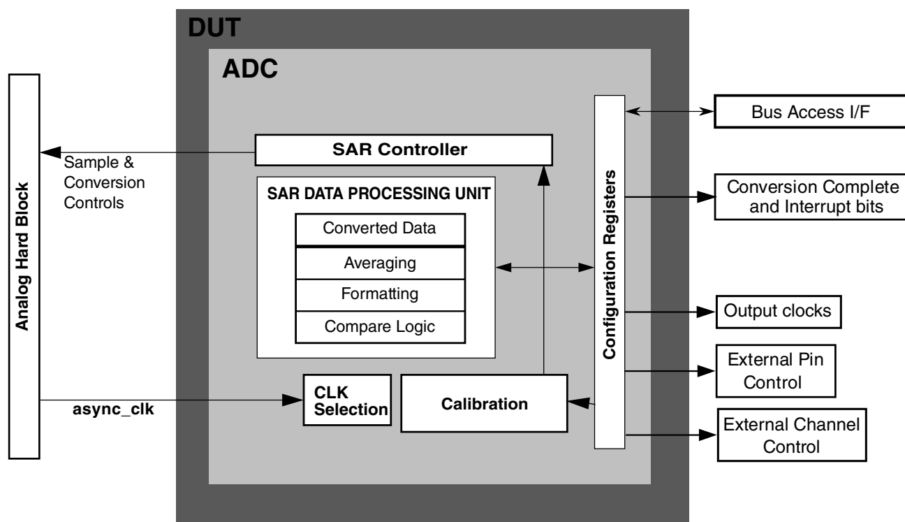
Figure 61-1. ADC I/F block diagram
