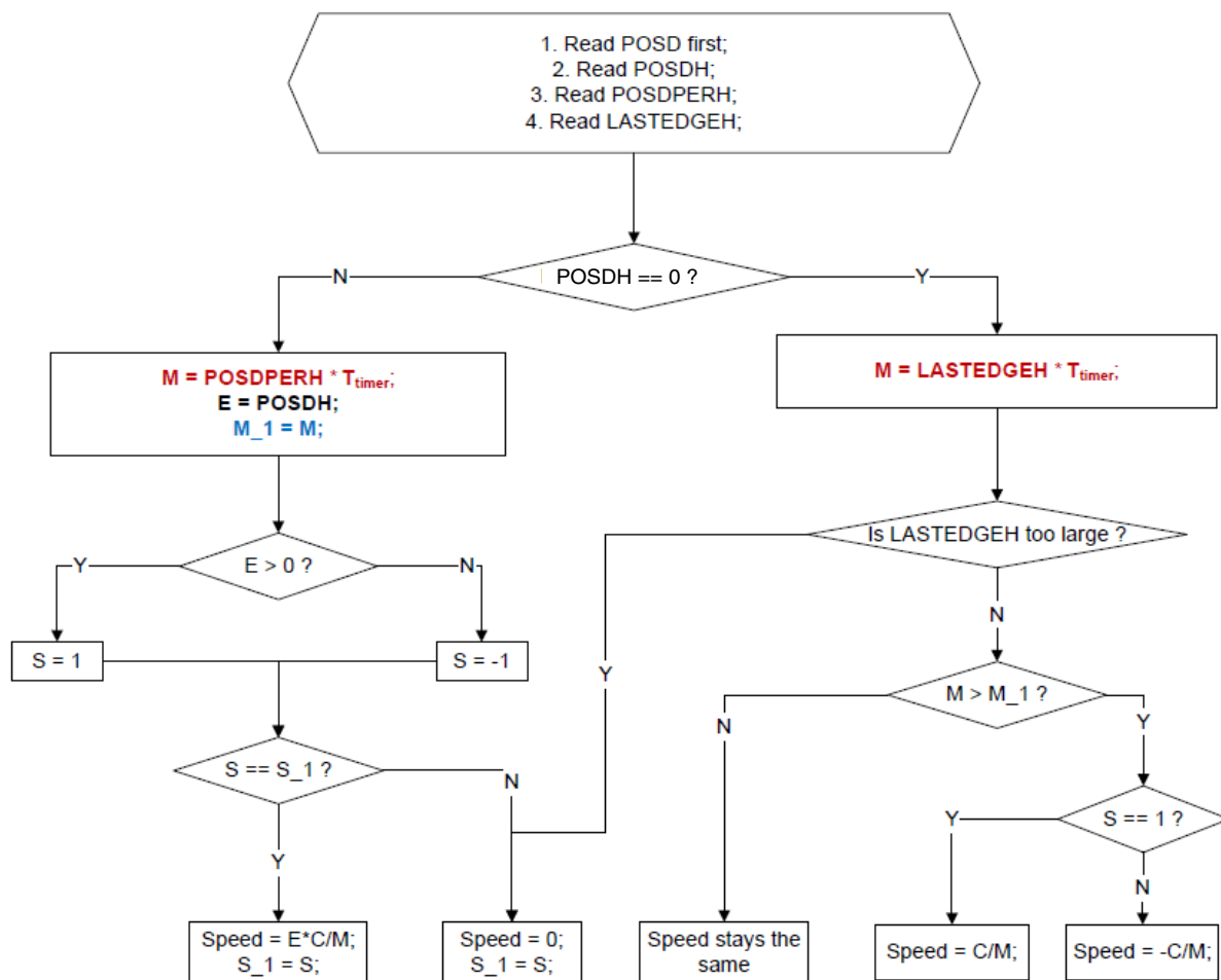
Figure 51-6. Flowchart of speed calculation with method
