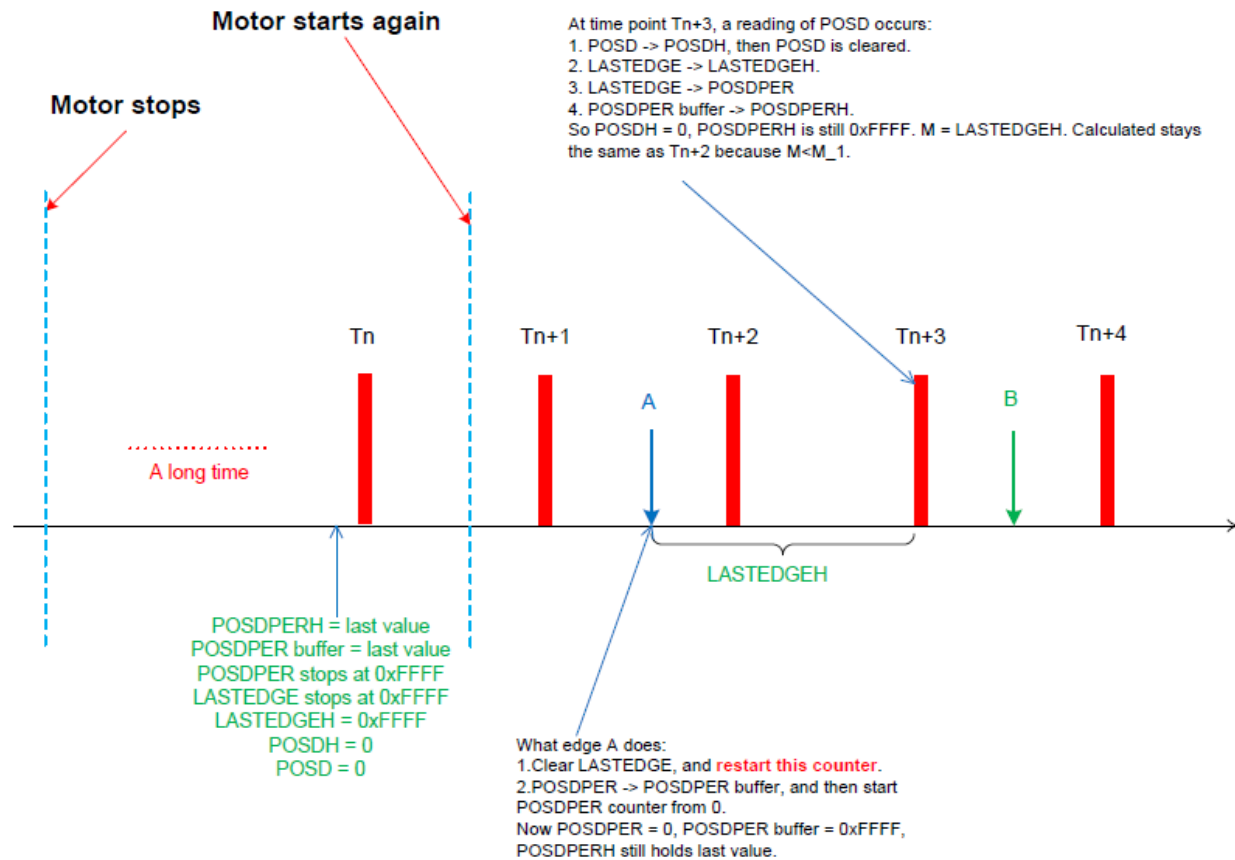
Figure 51-14. Speed measurement at time point T_{n+3}
