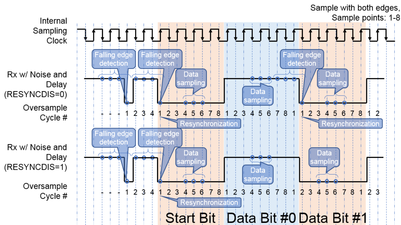
Figure 44-5. LPUART resynchronization
