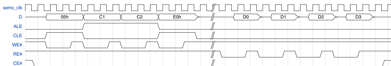
Figure 25-45. NAND Flash Access Command Type - Command + Address + Command + Read Phase
