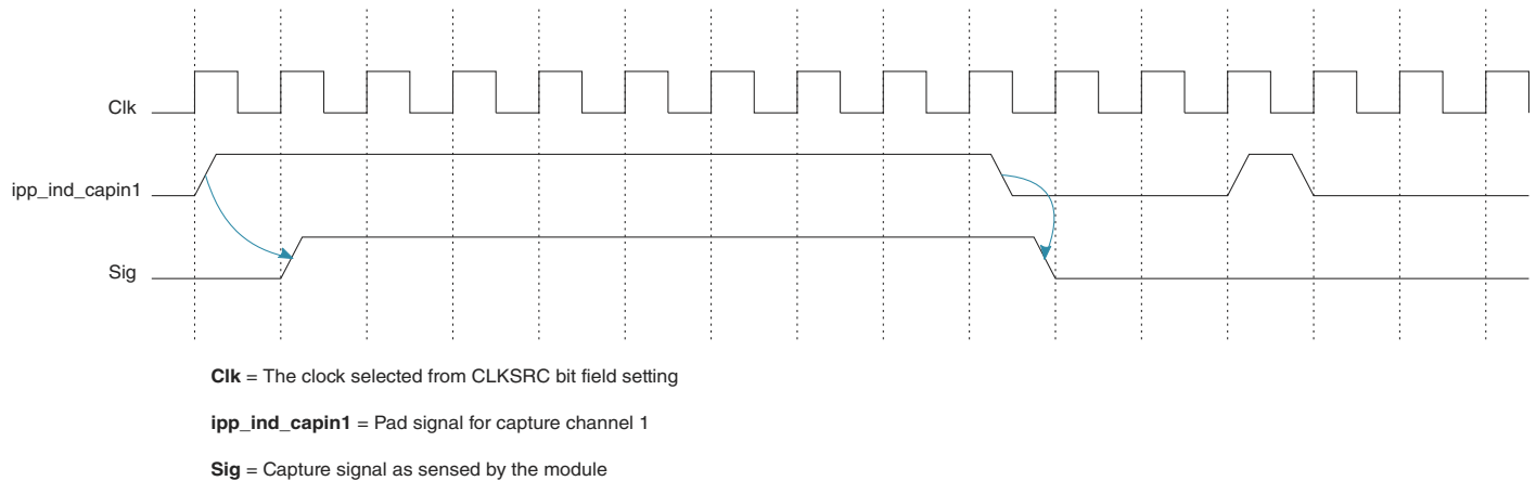
Figure 47-4. Input Capture Event Timing
