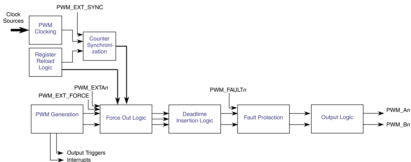
Figure 50-13. High-Level Output PWM Generation Block Diagram
