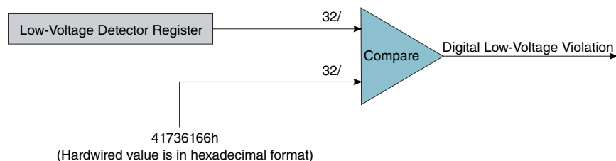
Figure 20-2. Digital low-voltage detector
