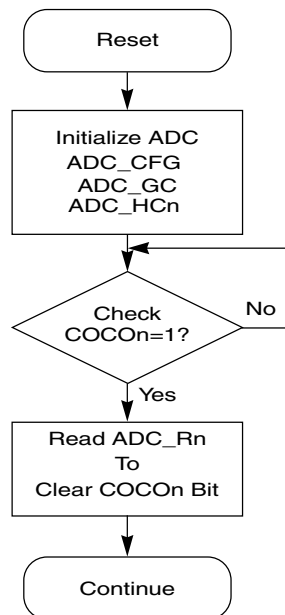
Figure 61-5. Initialization Flowchart for Example
