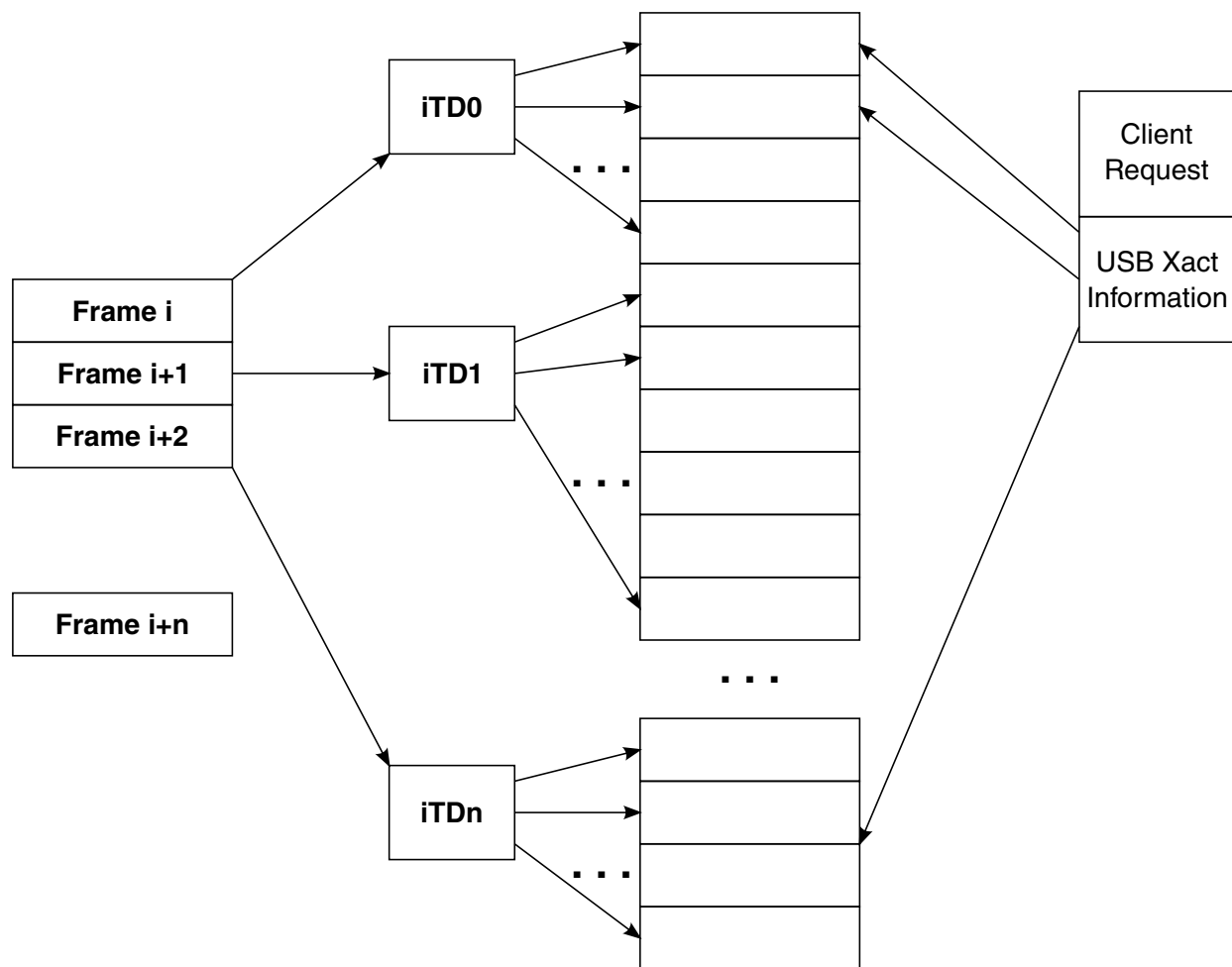
Figure 38-12. Example Association of iTDs to Client Request Buffer
