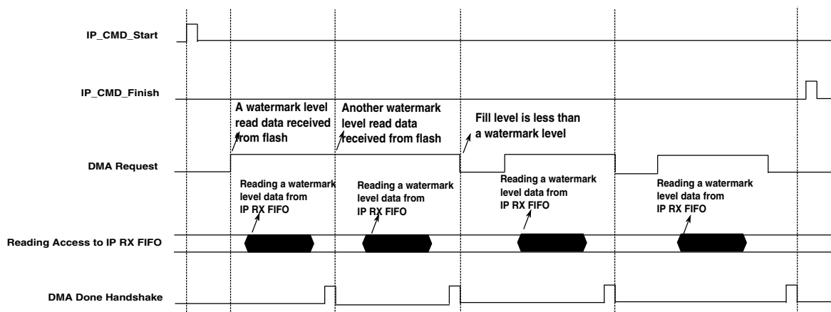
Figure 27-10. Reading from IP RX FIFO by DMA
