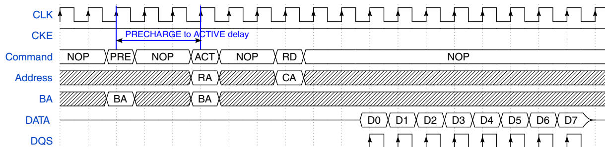
Figure 25-12. AXI Command - SDRAM READ
