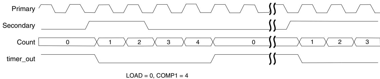
Figure 49-6. One-Shot Mode (CTRL[LENGTH]=1)
