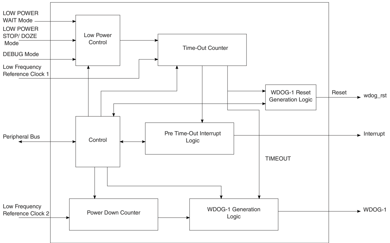
Figure 52-1. WDOG Diagram
