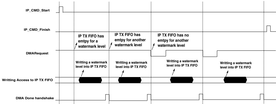
Figure 27-12. Filling from IP TX FIFO by DMA
