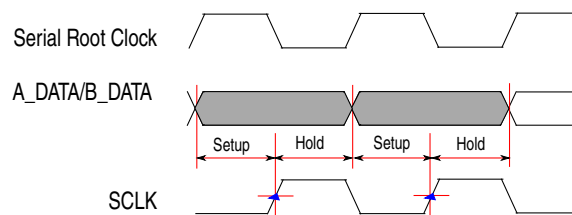
Figure 27-19. SDR instruction in SDR sequence
