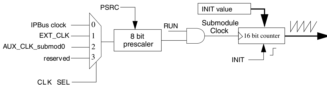
Figure 50-15. Clocking Block Diagram for PWM Submodule 1,2,3
