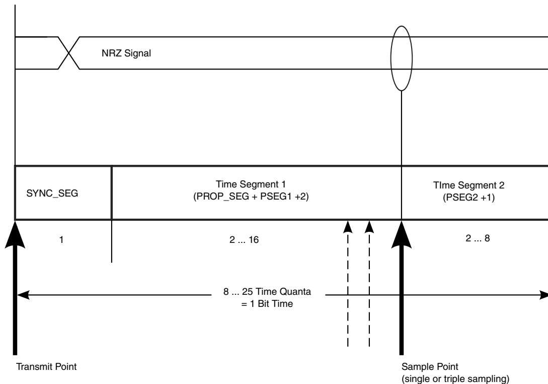
Figure 40-2. Segments within the Bit Time
