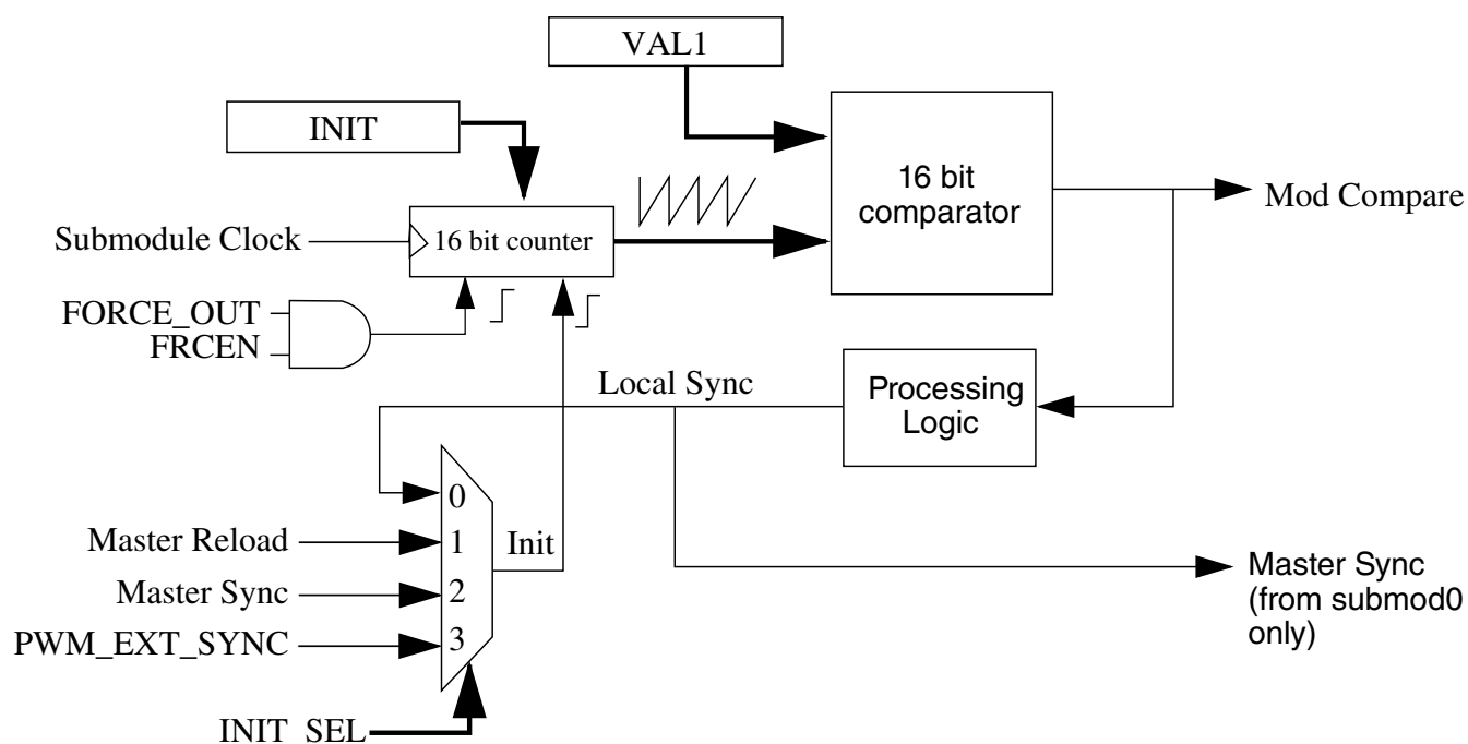
Figure 50-17. Submodule Timer Synchronization
