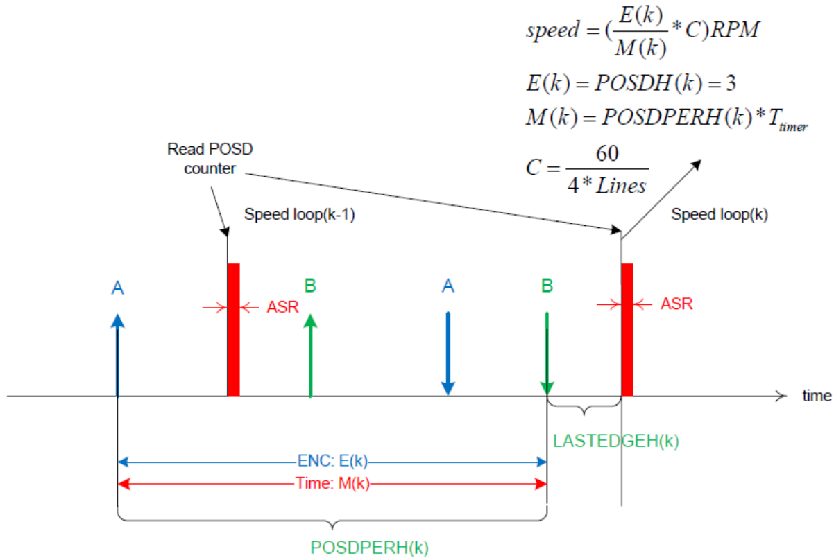
Figure 51-5. High speed measurement with method
