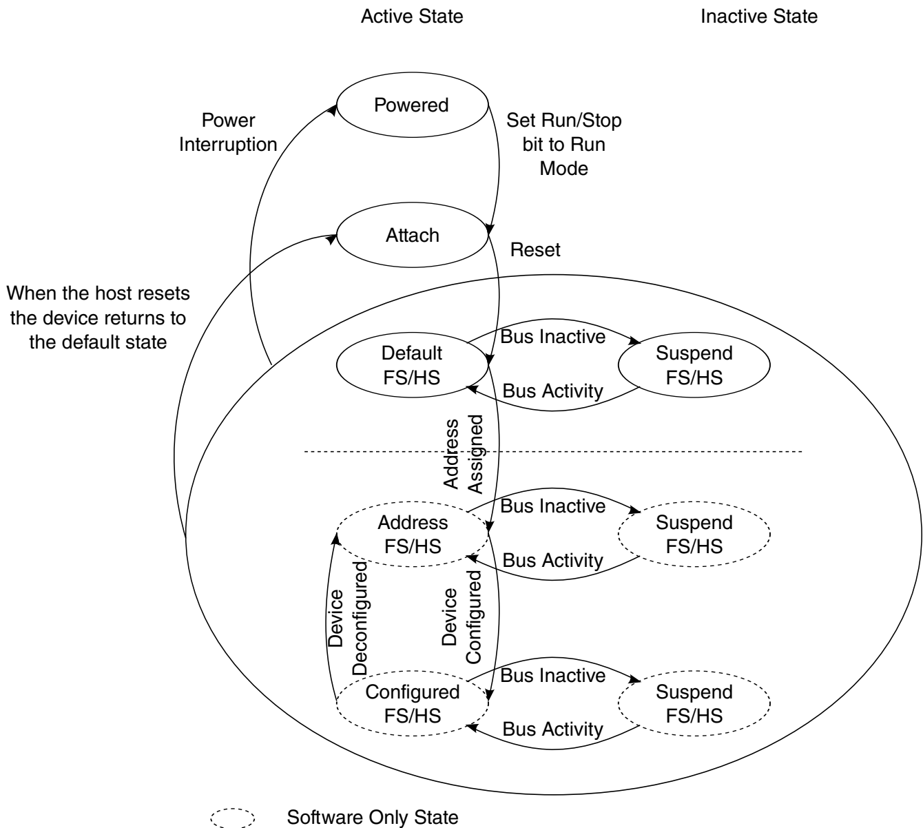
Figure 38-28. Device State Diagram
