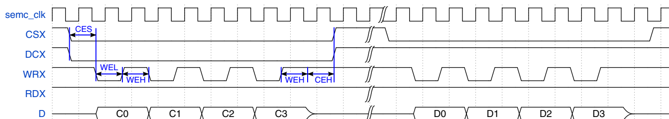
Figure 25-62. DBI Write Operation
