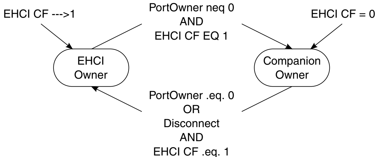
Figure 38-5. Port Owner Handoff State Machine
