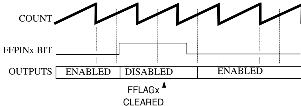
Figure 50-33. Manual Fault Clearing (FCTRL[FSAFE]=1)
