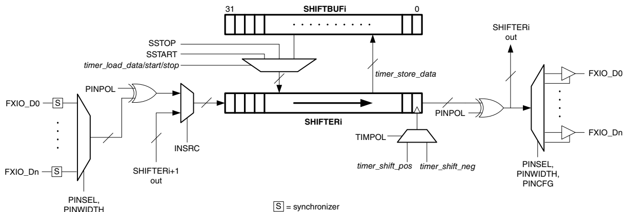
Figure 45-2. Shifter Microarchitecture
