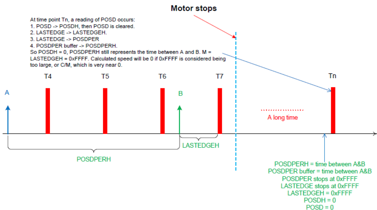
Figure 51-12. Speed measurement at time point Tn
