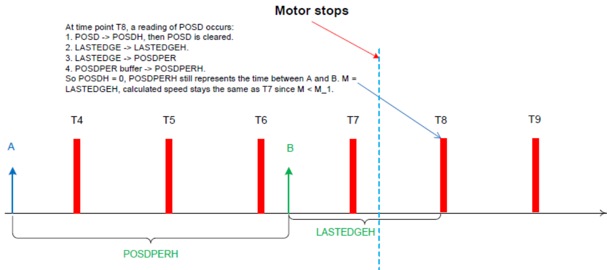
Figure 51-11. Speed measurement at time point T8
