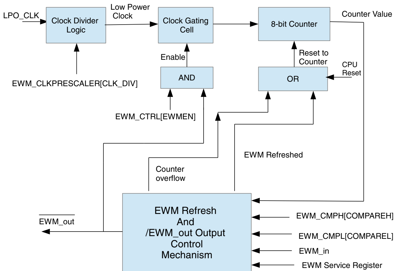
Figure 54-1. EWM Block Diagram
