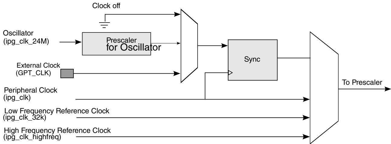
Figure 47-2. GPT Counter Clocks Diagram
