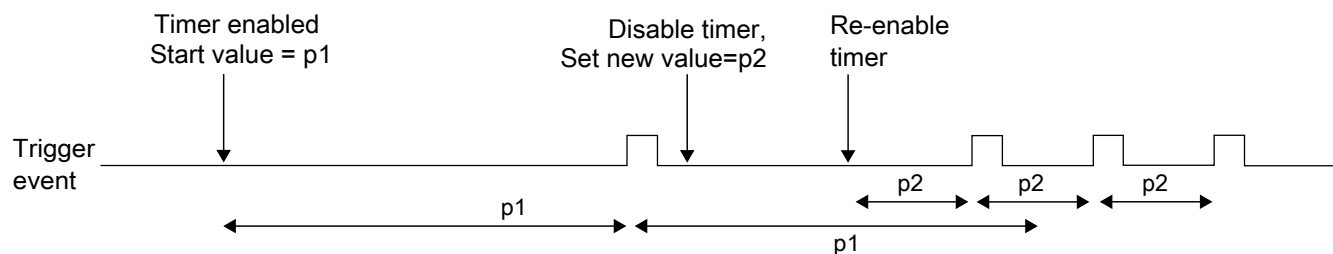
Figure 48-3. Modifying running timer period
