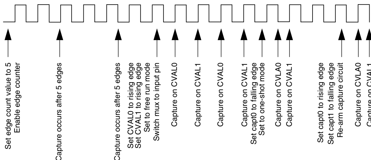
Figure 50-10. Capture Capabilities of the E-Capture Circuit
