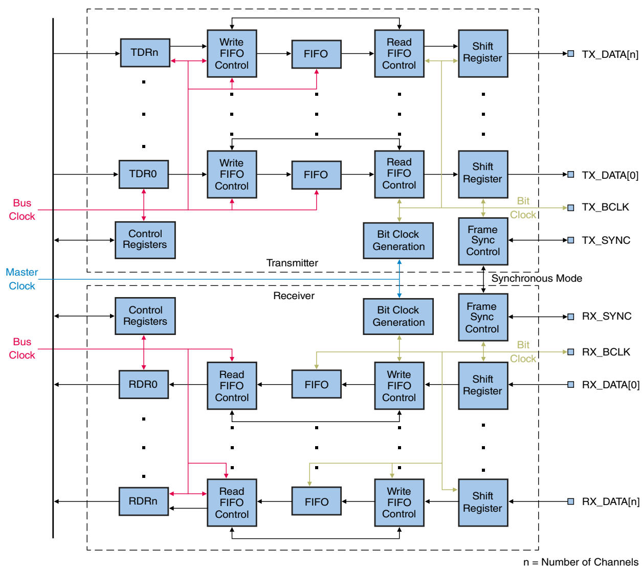
Figure 34-1. SAI block diagram
