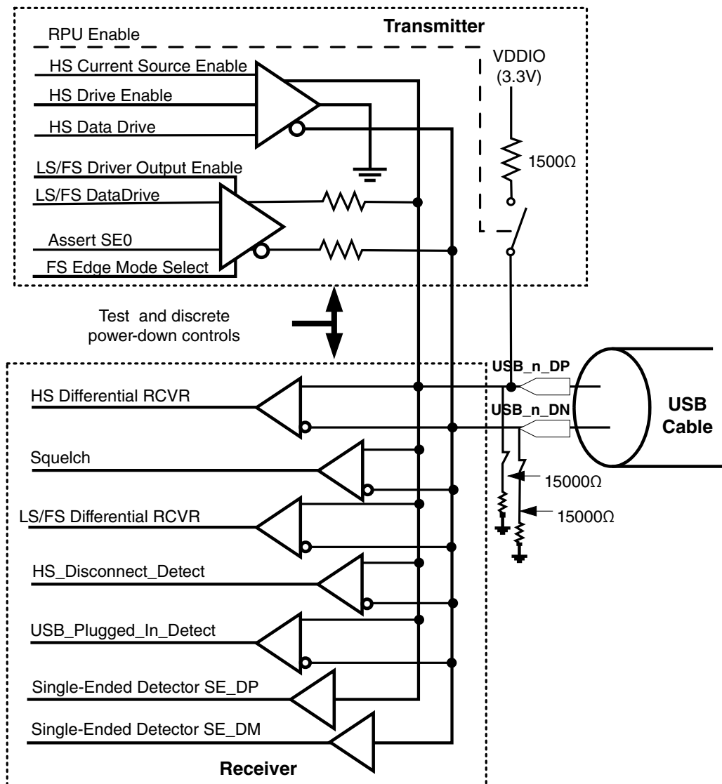
Figure 39-1. USB 2.0 PHY Analog Transceiver Block Diagram
