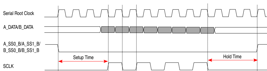
Figure 27-23. Chip selection output timing for DDR sequence
