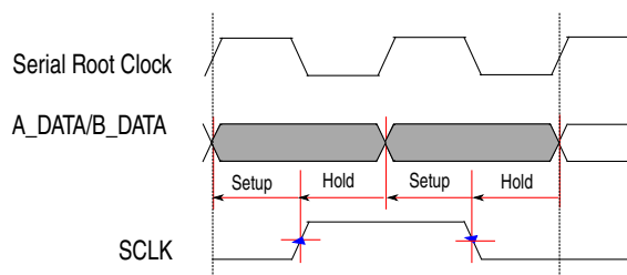
Figure 27-21. DDR instruction in DDR sequence
