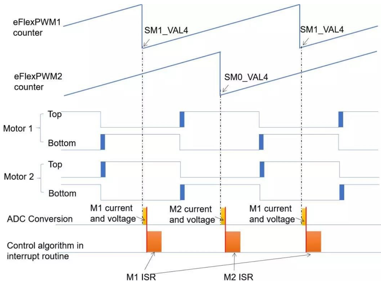
Figure 62-4. Synchronization between ADC and PWMs
