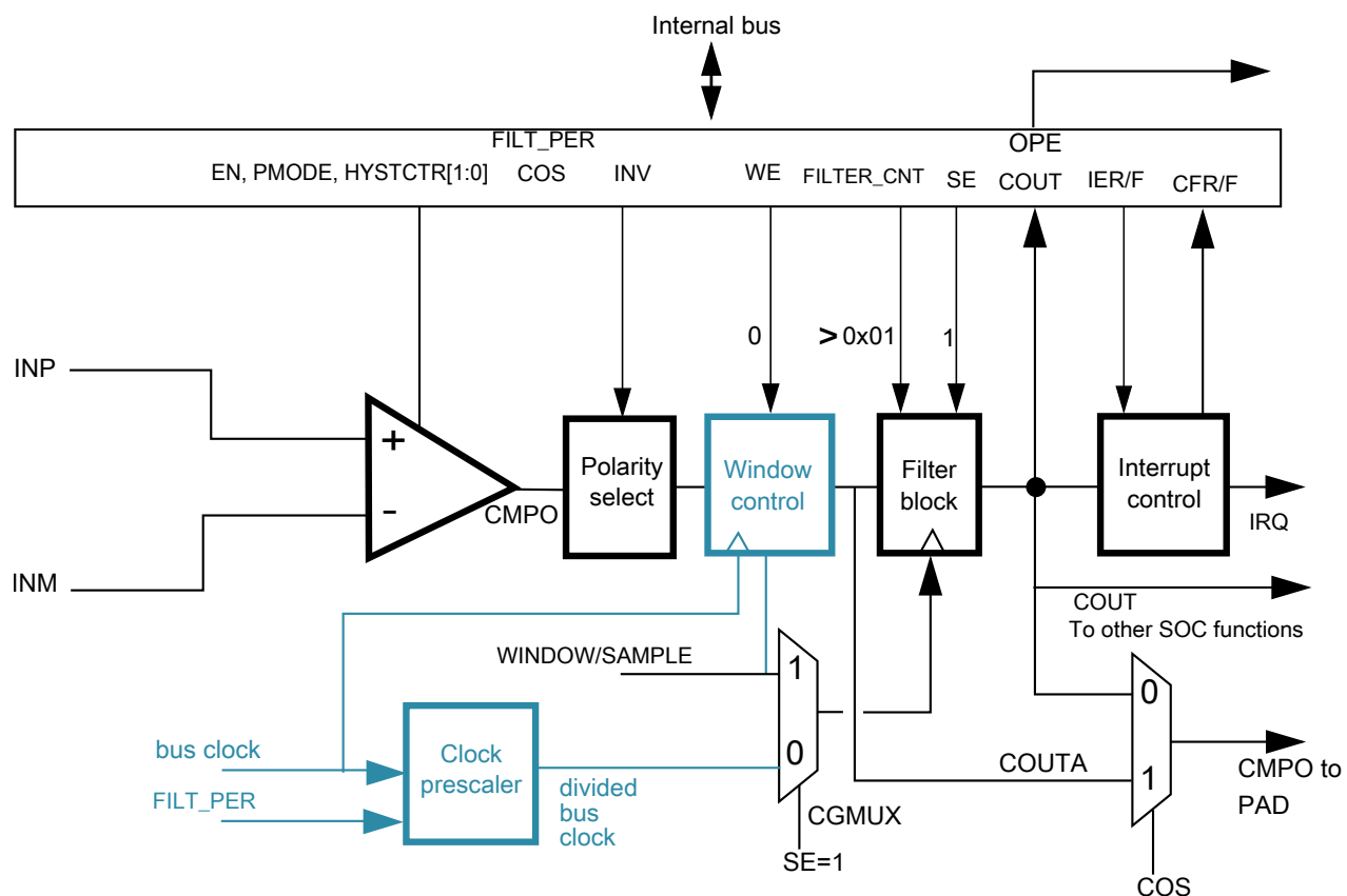
Figure 60-6. Sampled, Filtered (# 4A): sampling point externally driven
