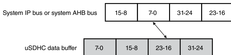
Figure 26-5. Data swap between system bus and uSDHC data buffer in half word big endian mode
