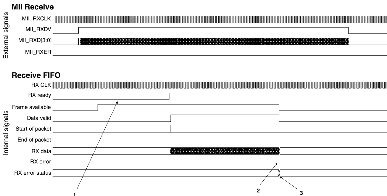
Figure 37-17. Receive FIFO overflow protection
