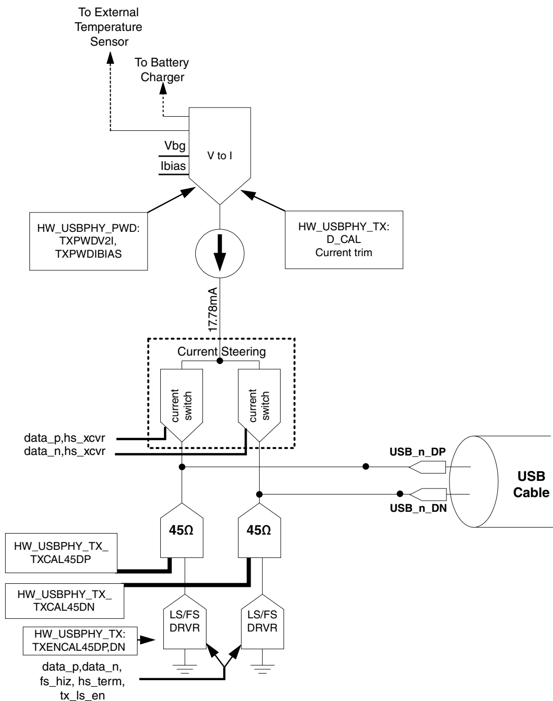
Figure 39-2. USB 2.0 PHY Transmitter Block Diagram
