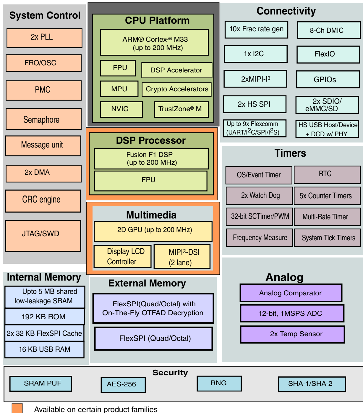
Figure 1. i.MX RT500 Block Diagram
