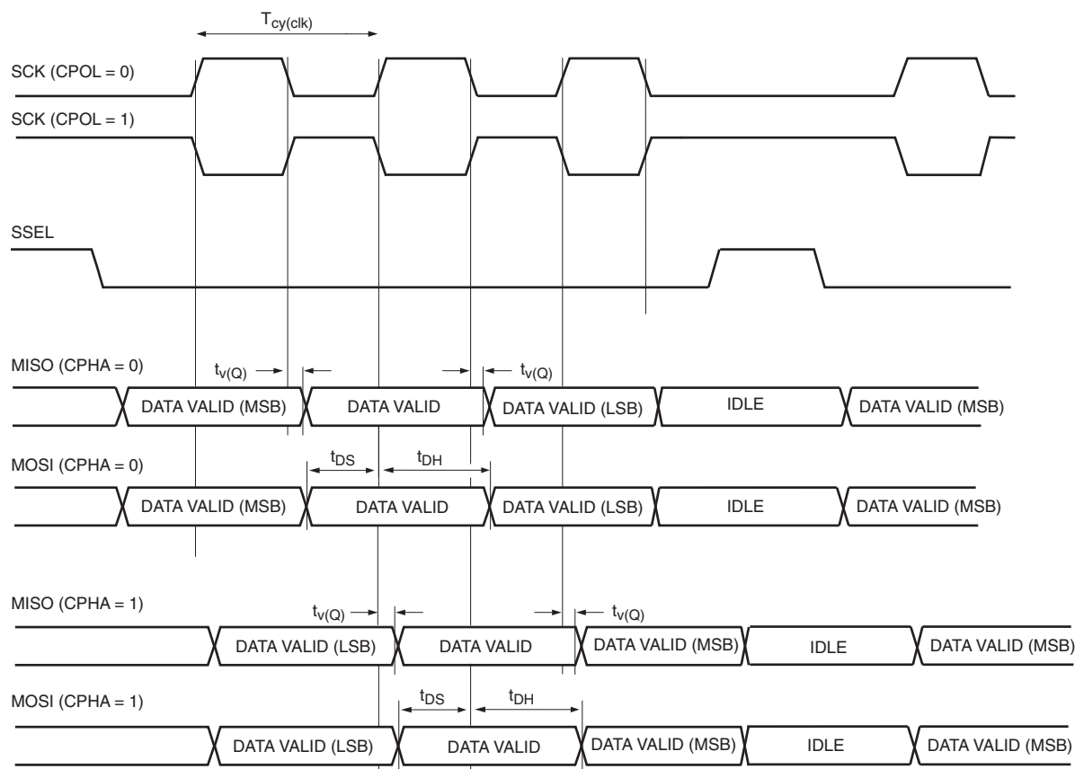
Figure 30. SPI slave timing
