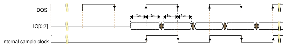
Figure 17. DDR mode (input timing, mode 3)
