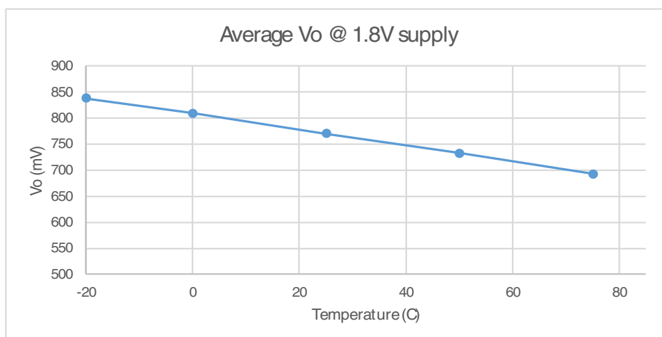
Fig 29. Average Vo @ 1.8V supply
