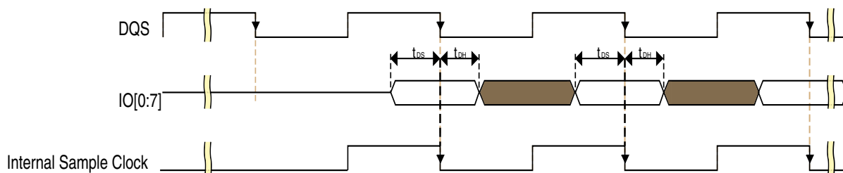
Figure 13. SDR mode (input timing, mode 3)
