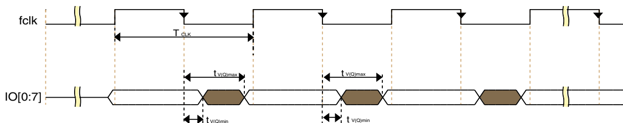
Figure 14. SDR mode (output timing, mode 0 and 1)
