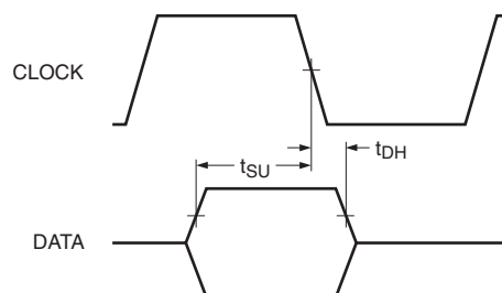
Figure 32. DMIC timing diagram
