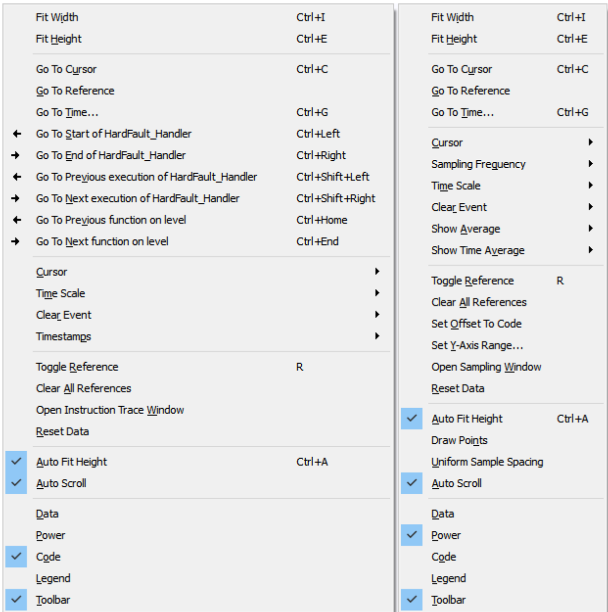
Context menus of the code pane (left) and power pane (right).
