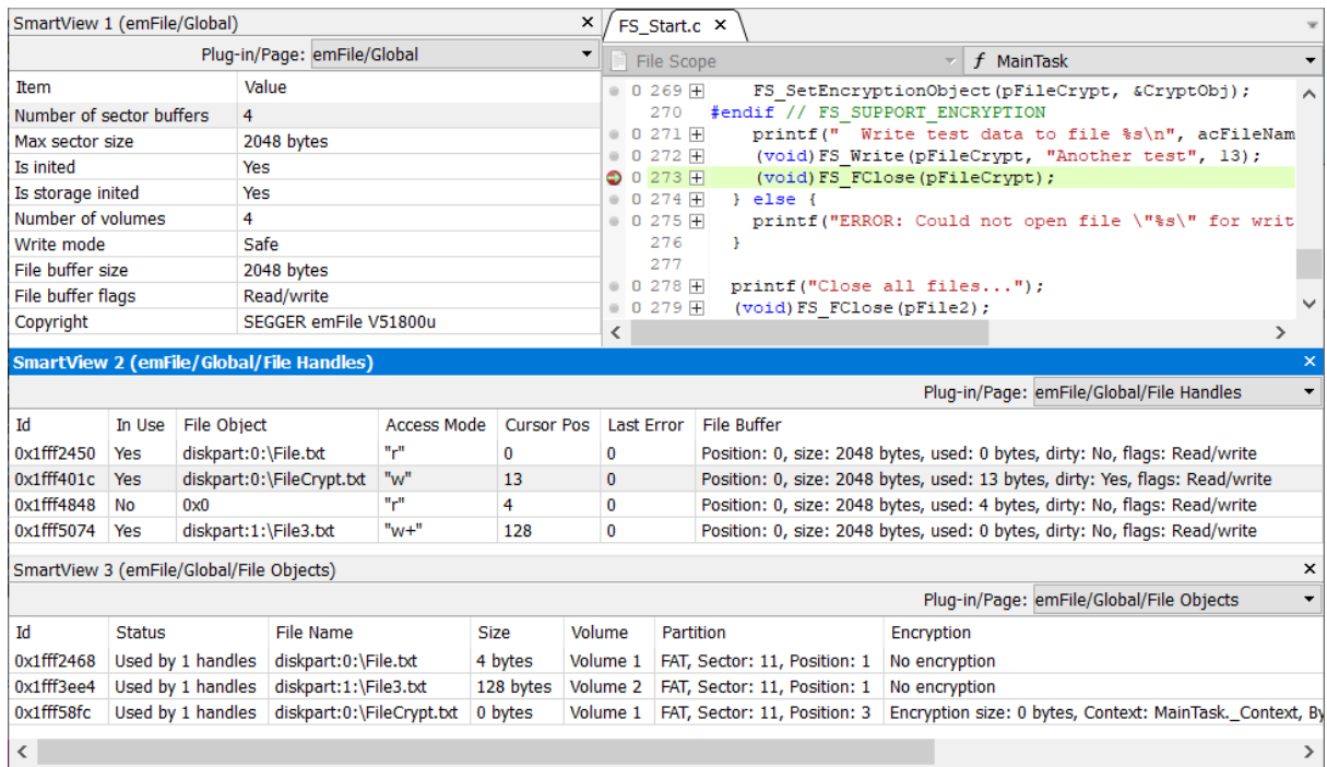
Three SmartView Windows displaying emFile information.
