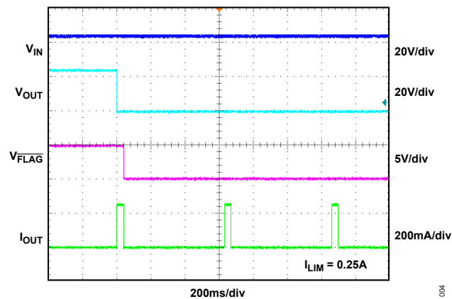
Figure 4. Autoretry Current-Limit Response
