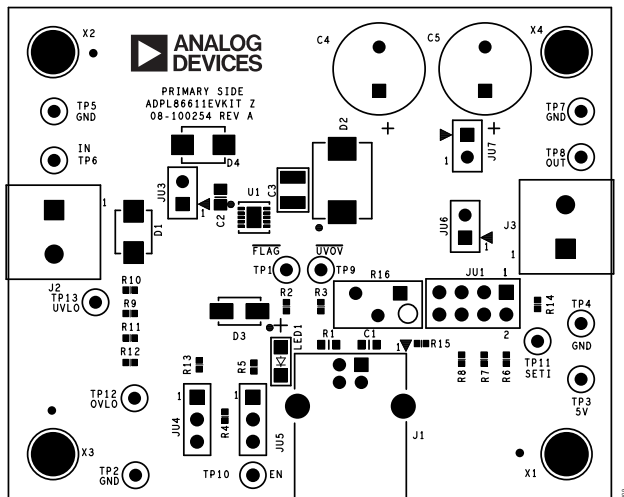
Figure 9. ADPL86611 EV Kit PCB Layout—Top Silkscreen
