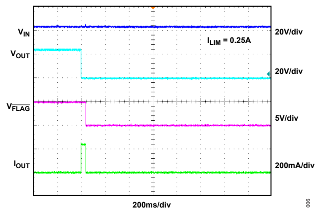
Figure 6. Latch-Off Current-Limit Response
