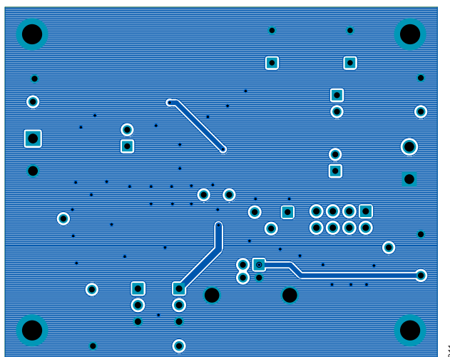
Figure 11. ADPL86611 EV Kit PCB Layout—Bottom Layer
