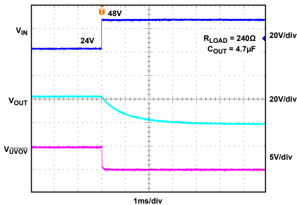
Figure 7. Overvoltage Fault Response
