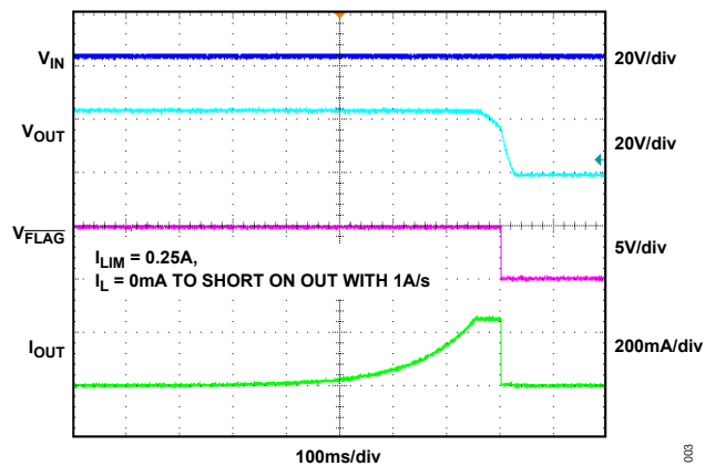
Figure 3. Current-Limit Response
