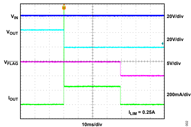
Figure 2. Output Short-Circuit Response
