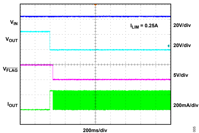
Figure 5. Continuous Current-Limit Response
