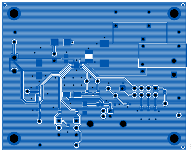
Figure 10. ADPL86611 EV Kit PCB Layout—Top Layer
