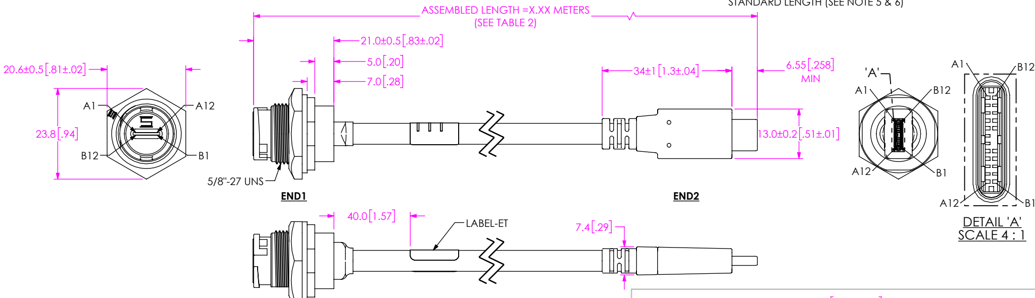
FIG 1 BPCU-C-X-X.XX-UC-P SHOWN
