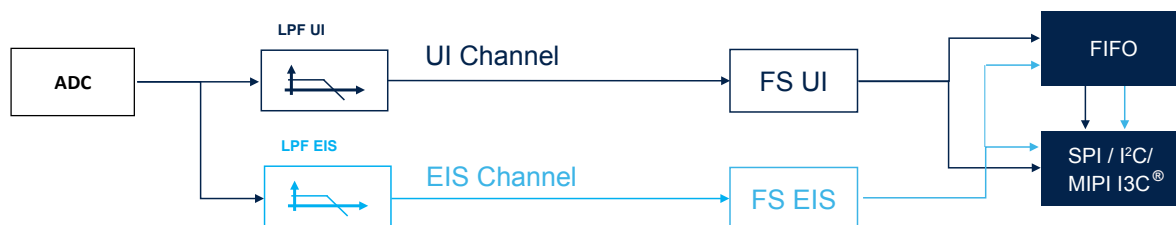
Figure 25. Gyroscope enhanced EIS and UI block diagram
