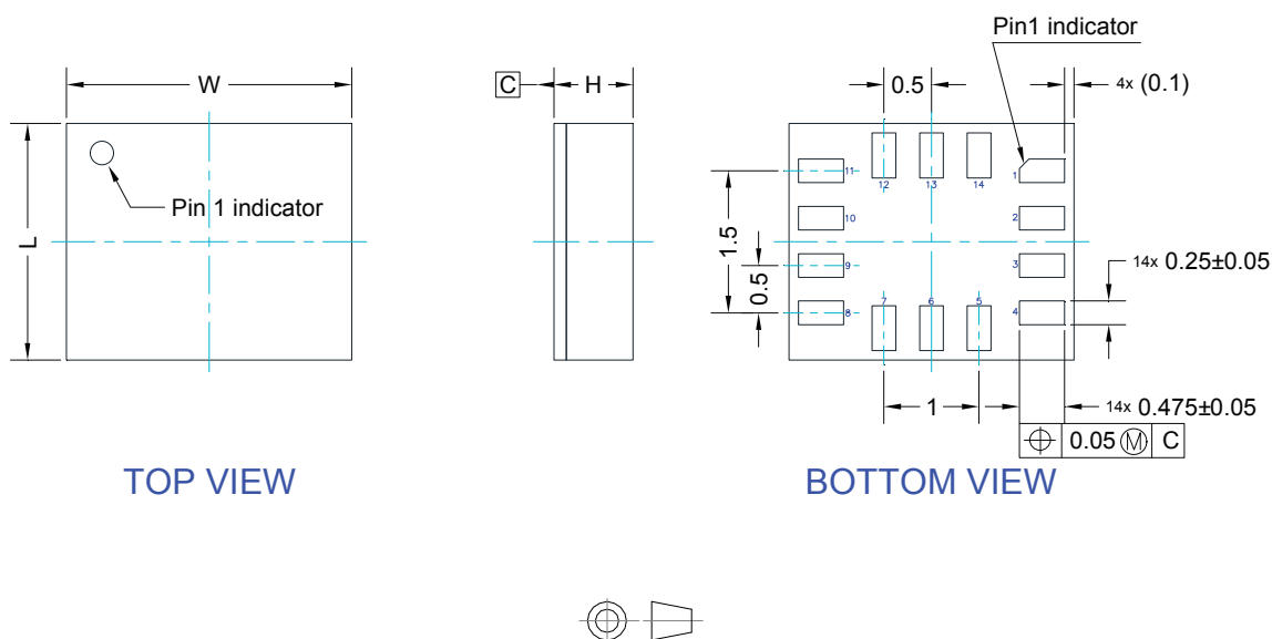
Figure 33. LGA-14L 2.5 x 3.0 x 0.86 mm package outline and mechanical data
