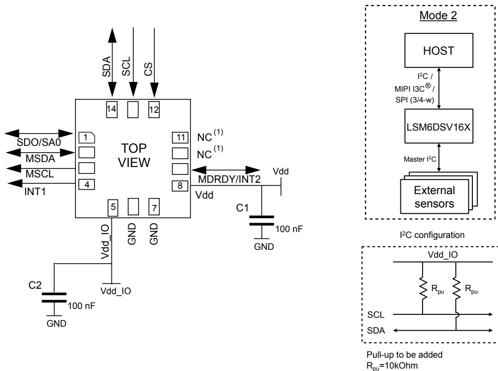
Figure 30. LSM6DSV16X electrical connections in mode 2
