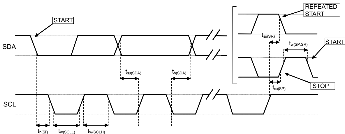
Figure 9. I 2 C slave timing diagram
