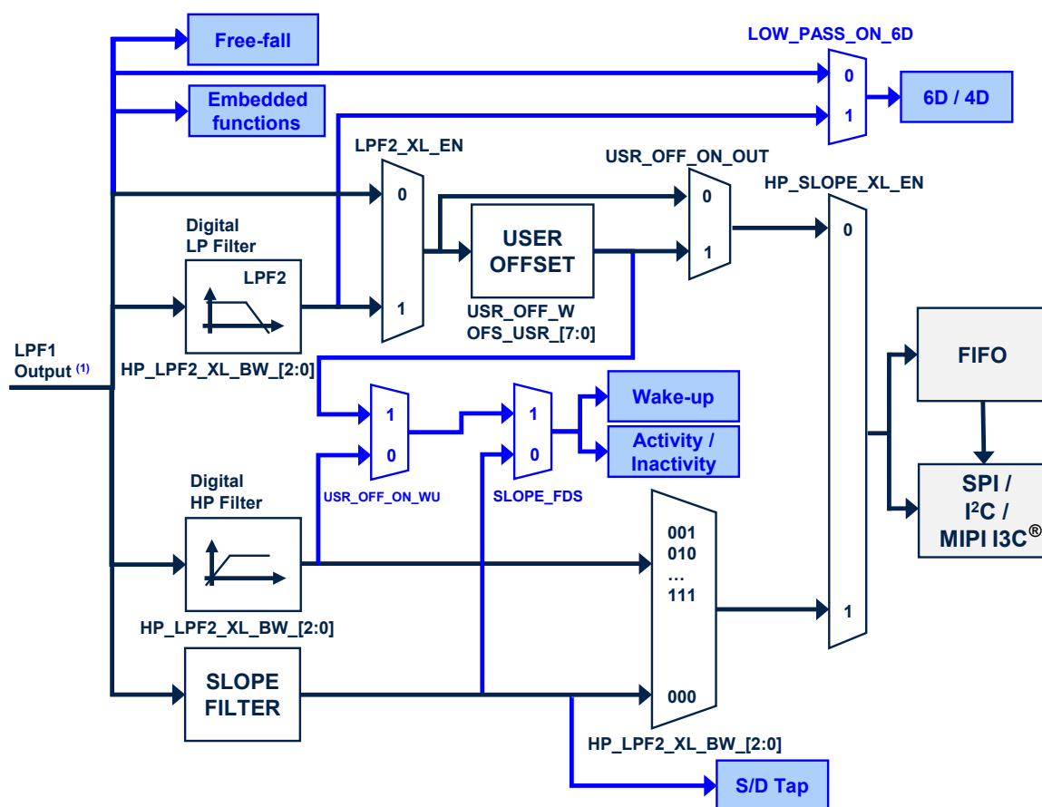
Figure 20. Accelerometer composite filter
