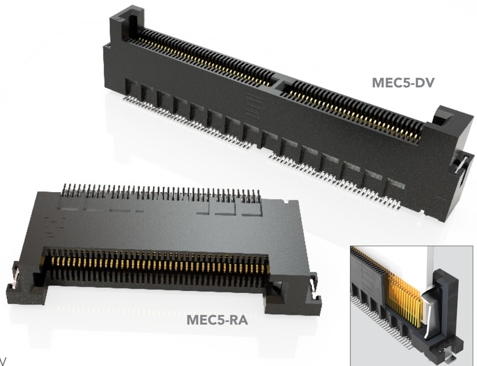
Side Justification Technology Forces Card and Body to Common Datum
