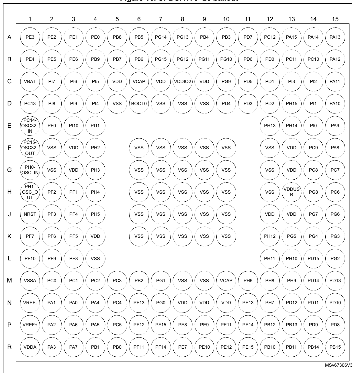
Figure 16. UFBGA176+25 ballout
