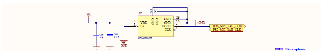
Figure 20. Microphone (MP34DT06JTR)
