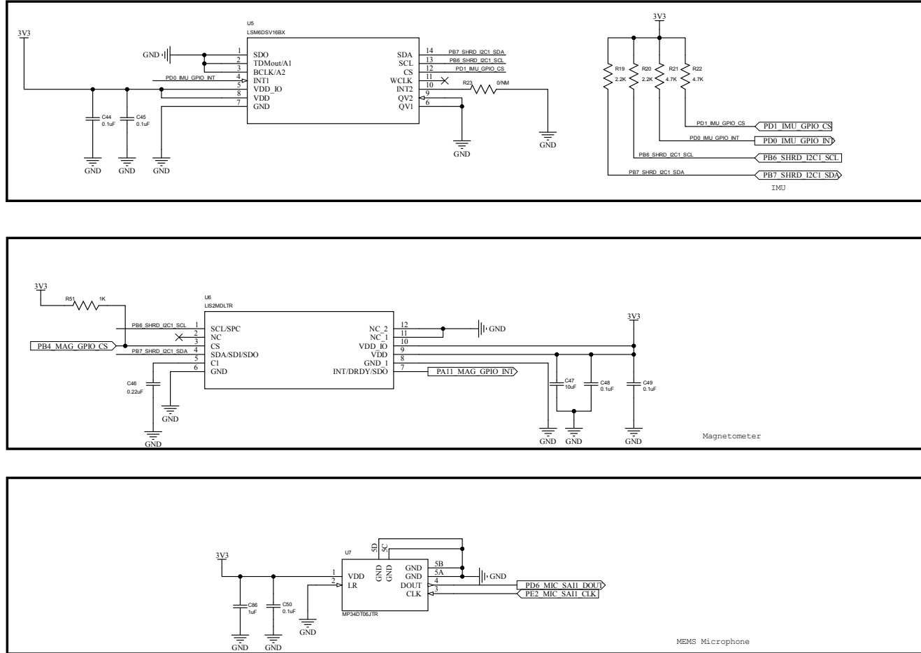
Figure 47. STEVAL-ROBKIT1-1 schematic (6 of 12)
