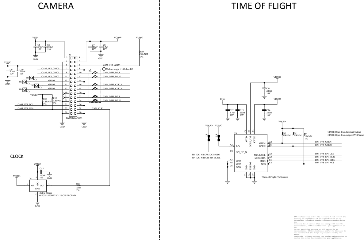
Figure 60. STEVAL-ROBKIT1-3 schematic (2 of 3)
