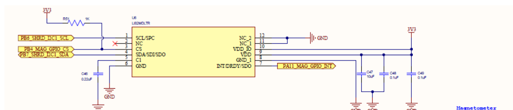
Figure 18. Magnetometer (LIS2MDL)
