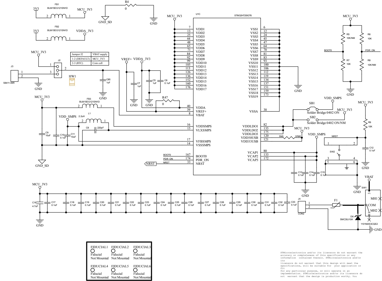
Figure 43. STEVAL-ROBKIT1-1 schematic (2 of 12)
