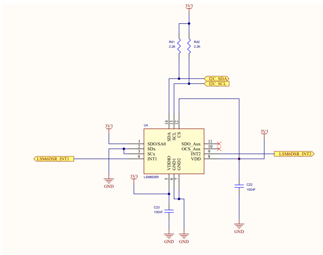
Figure 33. IMU (LSM6DSR)
