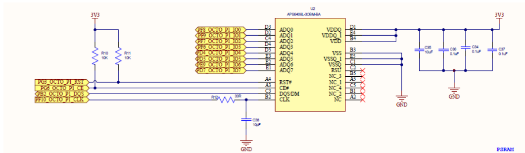
Figure 22. PSRAM memory
