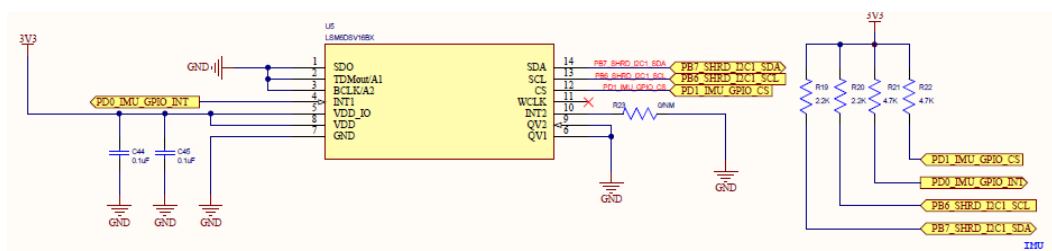
Figure 17. IMU (LSM6DSV16BX)
