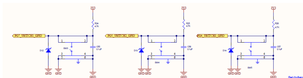
Figure 26. User Switches
