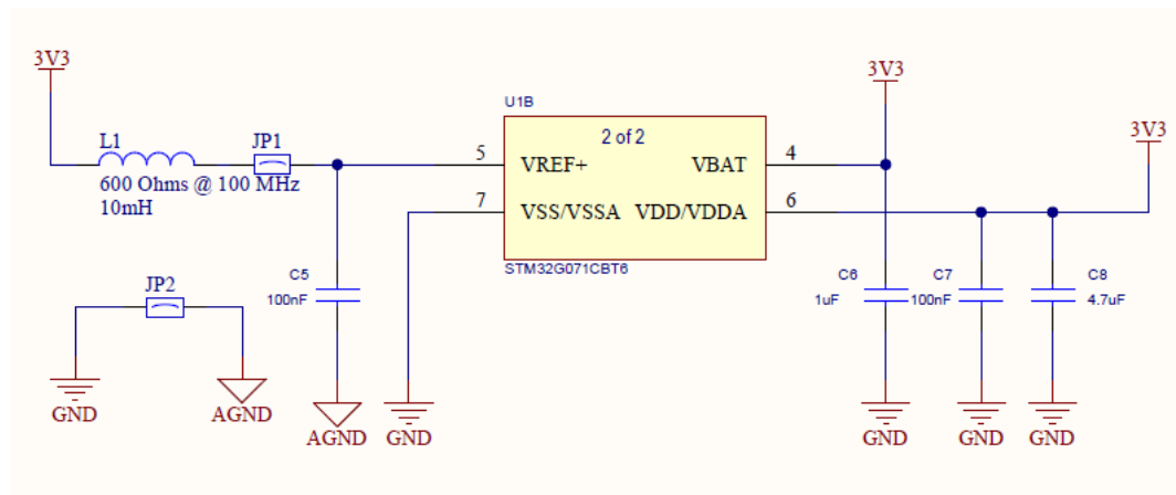
Figure 31. STM32G071CBT6 power section
