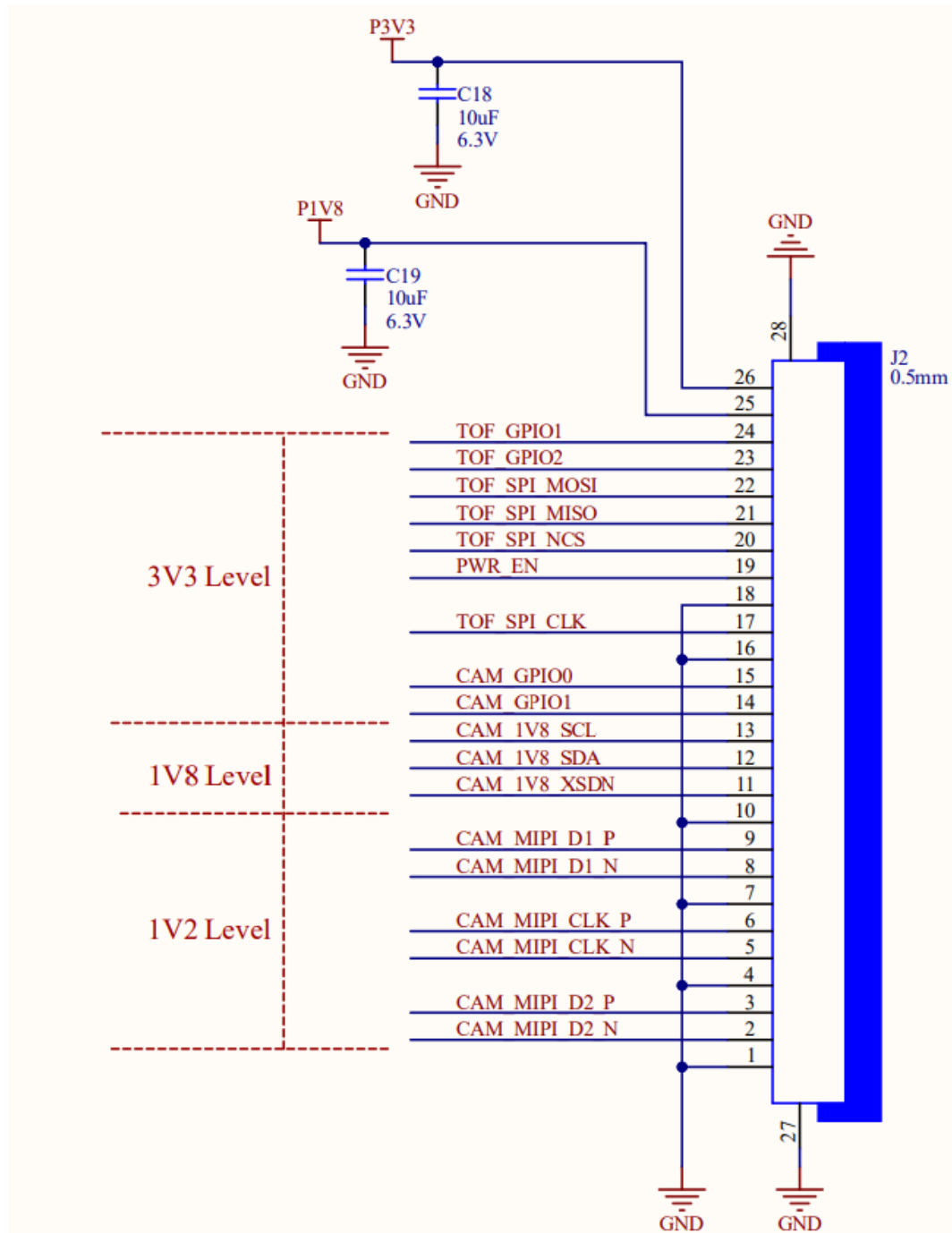
Figure 38. Camera module - mainboard interface
