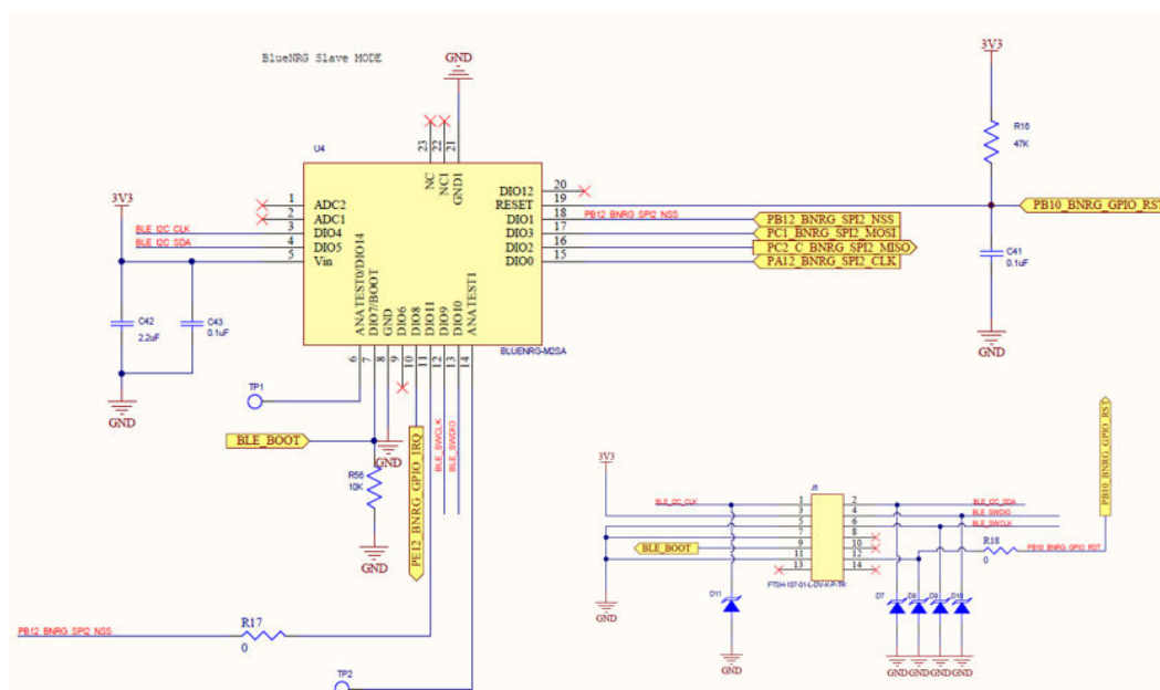
Figure 19. BlueNRG-M2SA
