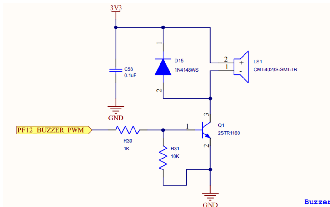
Figure 25. Buzzer
