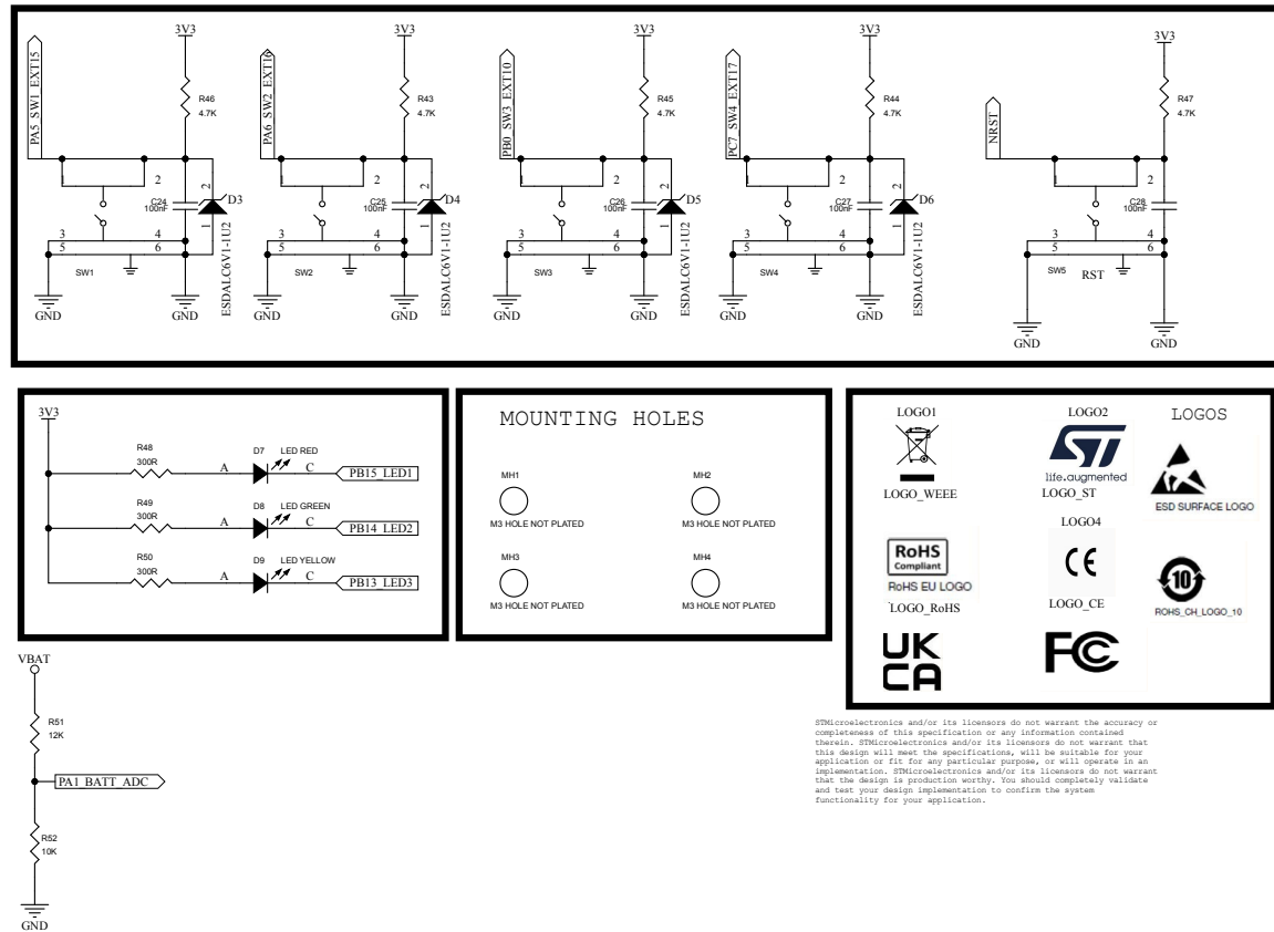
Figure 55. STEVAL-ROBKIT1-2 schematic (2 of 5)
