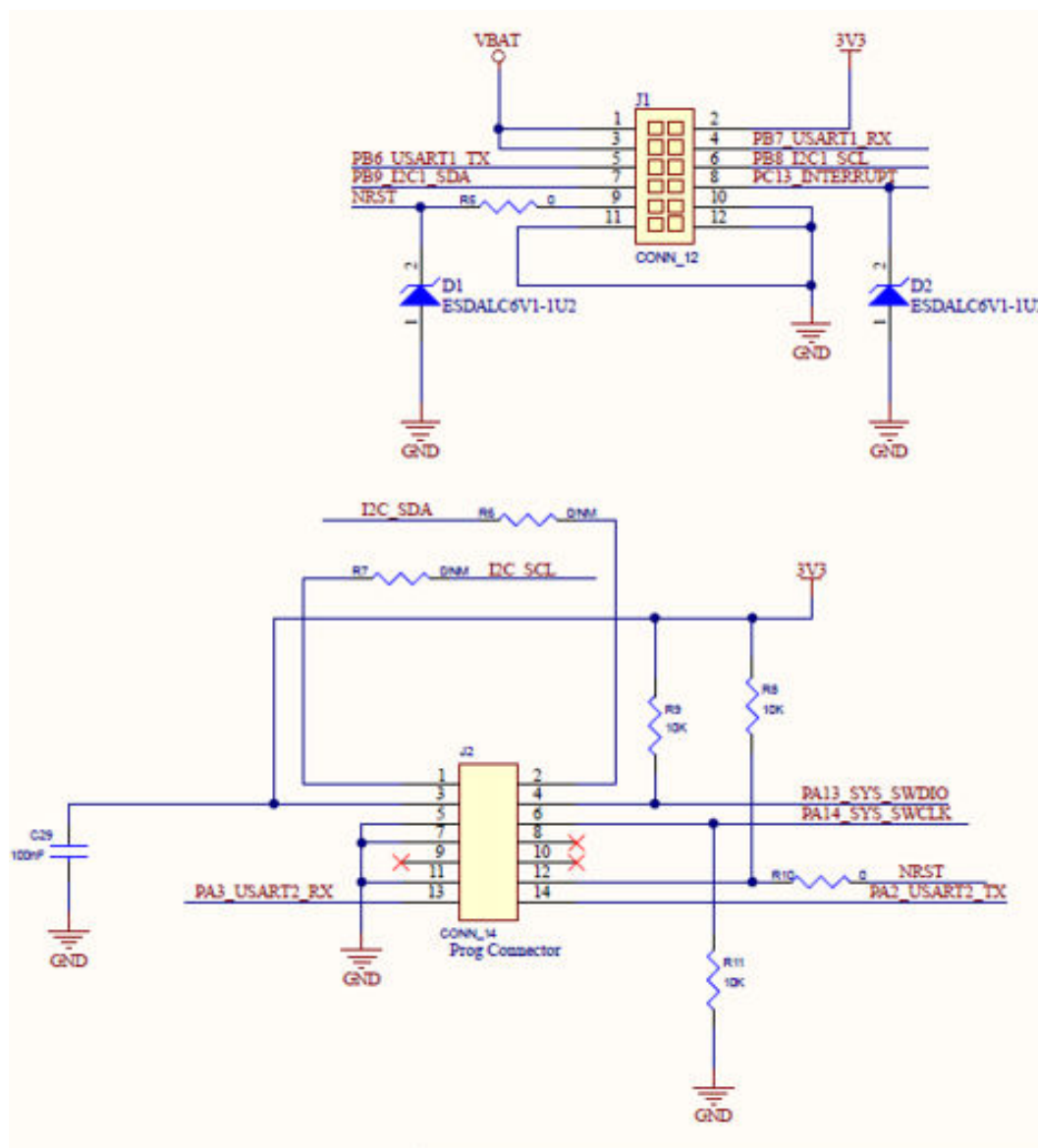
Figure 32. 12-pin box connector and 14-pin programming connector
