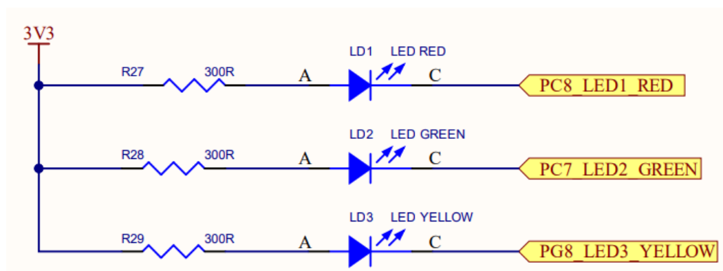
Figure 24. LED
