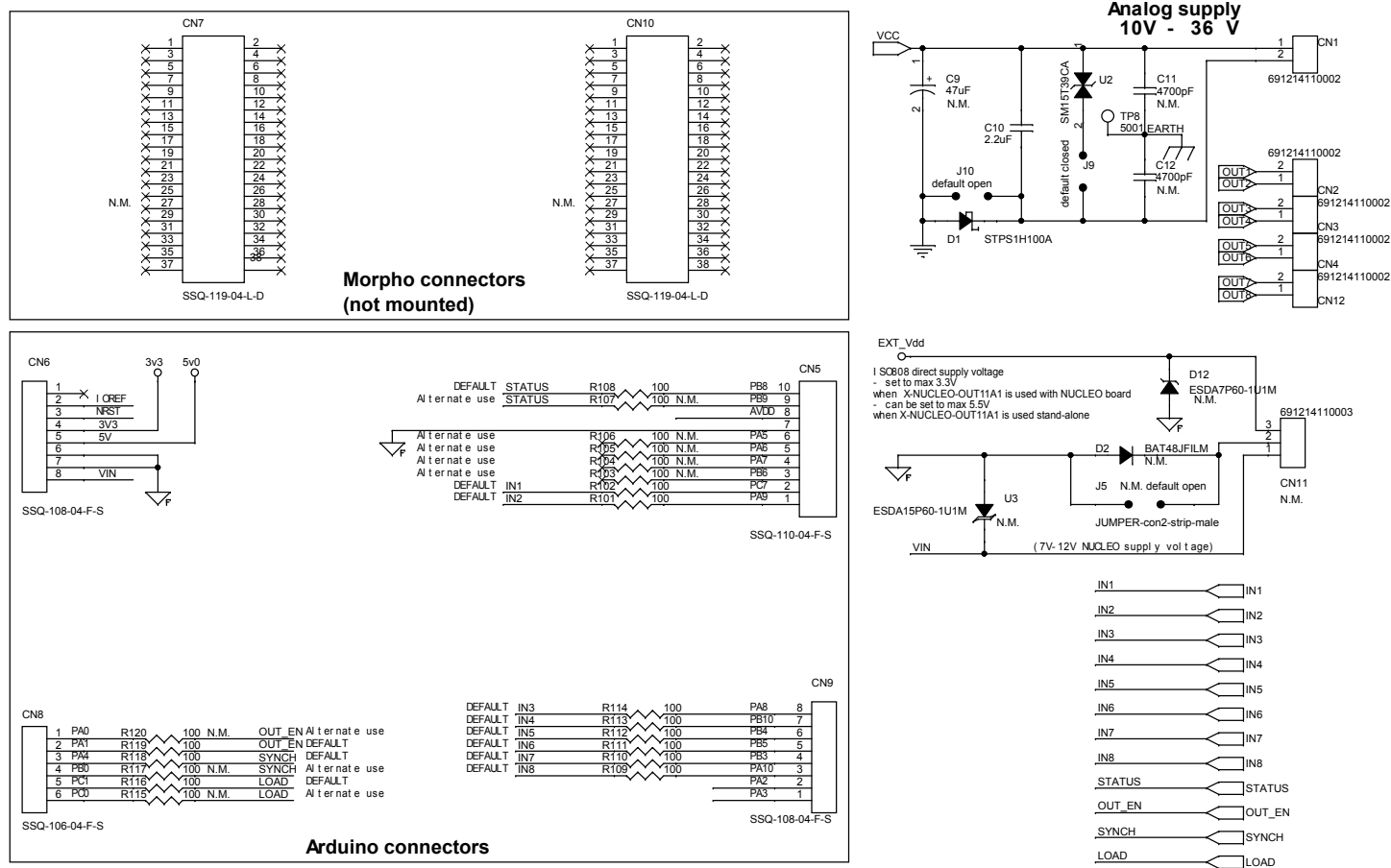
Figure 1. X-NUCLEO-OUT11A1 circuit schematic (1 of 2)
