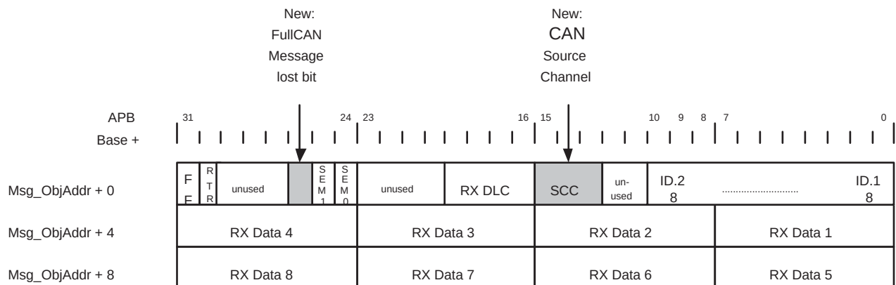
Fig 90. FullCAN message object layout
