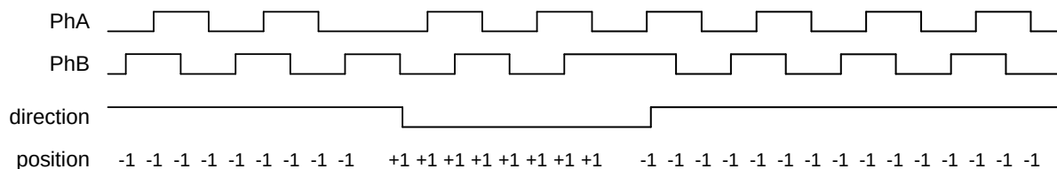
Fig 153. Quadrature Encoder Basic Operation
