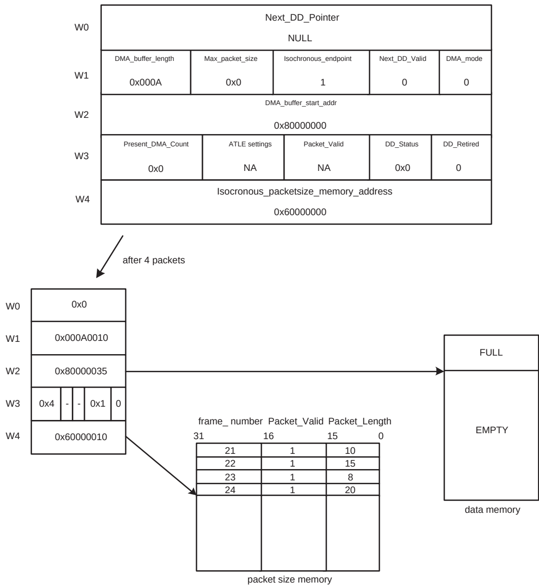
Fig 45. Isochronous OUT endpoint operation example
