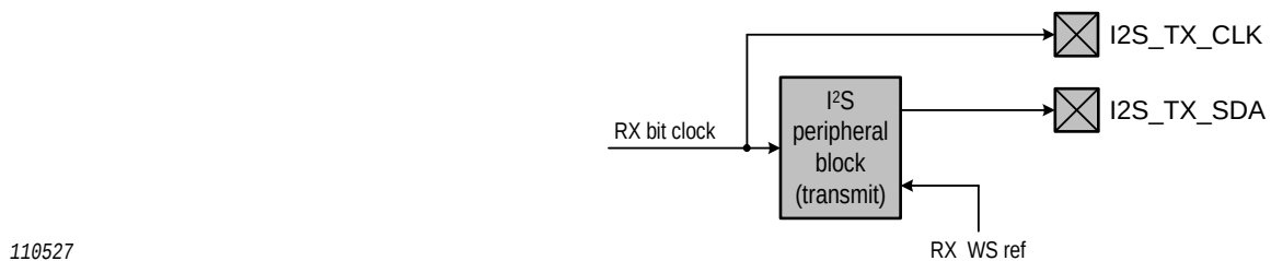
Fig 127. 4-wire transmitter master mode sharing the receiver bit clock and WS
