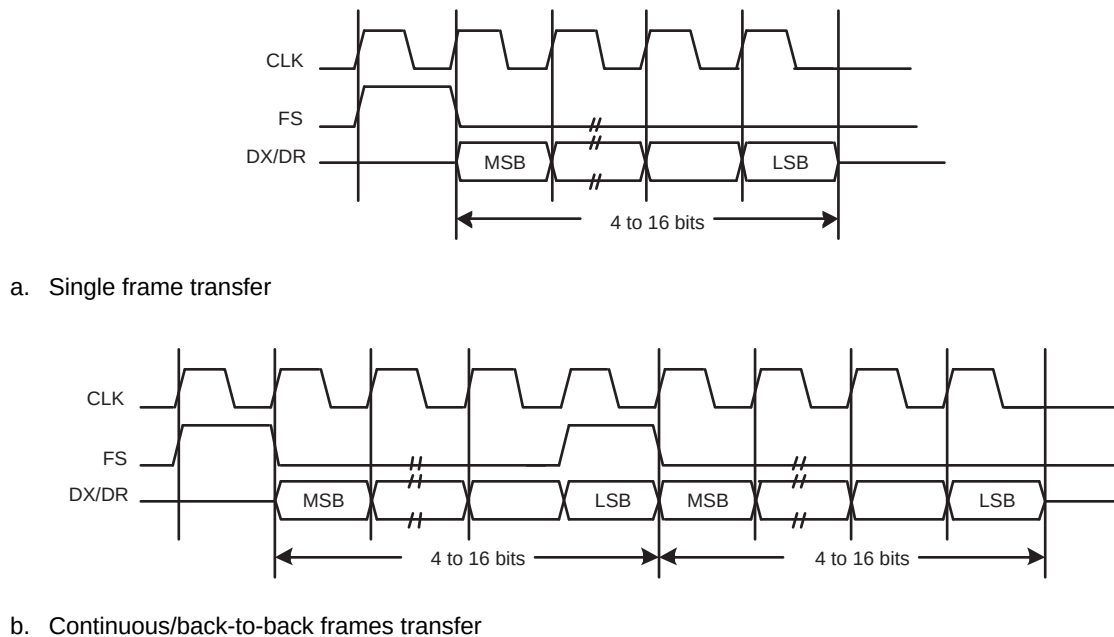
Fig 100. Texas Instruments Synchronous Serial Frame Format: a) Single and b) Continuous/back-to-back Two Frames Transfer
