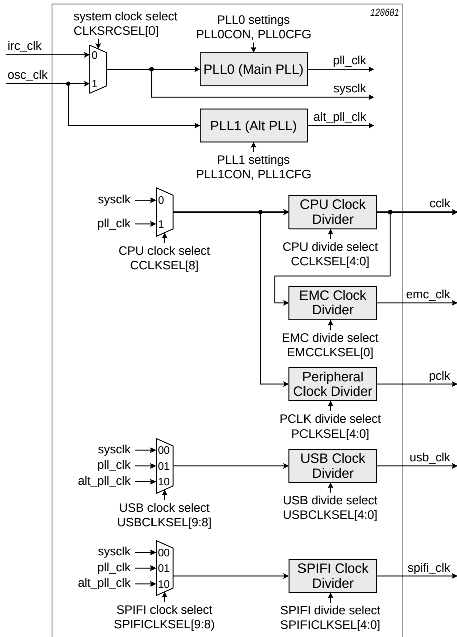
Fig 4. Clock generation
