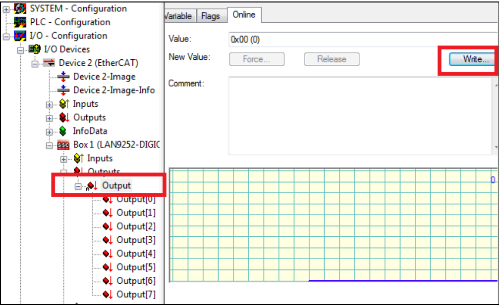
FIGURE 2-3: DIGIO OUTPUT .
