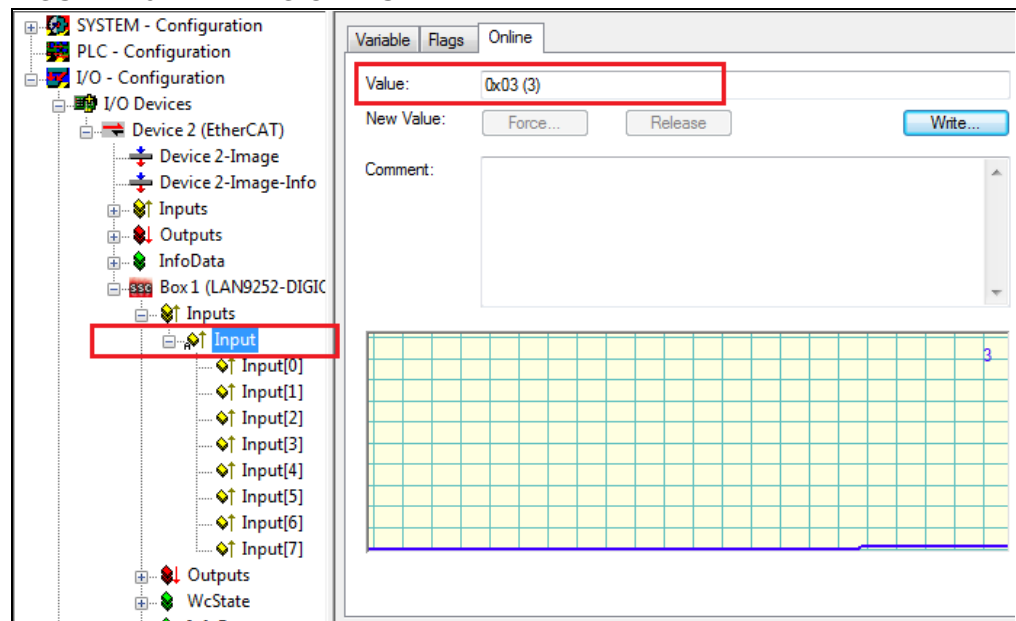
FIGURE 2-5: DIGIO INPUT .
