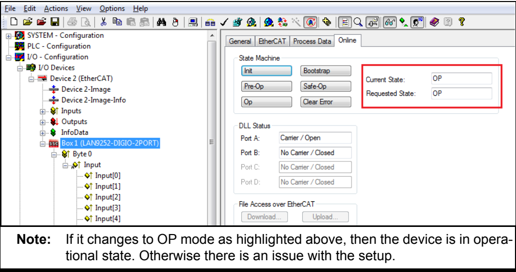
FIGURE 3-2: OP MODE
