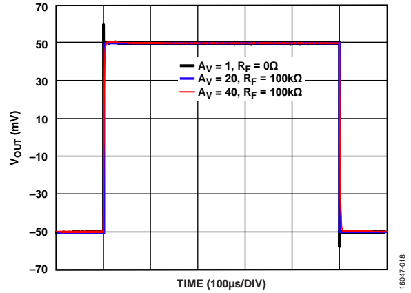
Figure 26. Small Signal Pulse Response at Various Gains, T_A = 25^\circ\text{C} , V_S = 110\text{ V} , V_{OUT} = 100\text{ mV p-p} , R_{LOAD} = 10\text{ k}\Omega , R_{ADJ} = 0\text{ }\Omega
