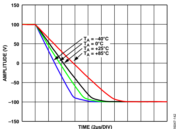
Figure 46. Large Signal Pulse Response at Various T_A with Two-Diode Forward Voltages, Falling Edge, A_V = 20 , V_S = \pm 110 V, V_{OUT} = 200 V p-p, R_F = 100 k \Omega , R_{LOAD} = 10 k \Omega , R_{ADJ} = 0 \Omega
