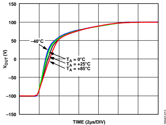
Figure 17. Large Signal Pulse Response at Various T_A , Rising Edge, A_V = 40 , V_S = \pm 110 V, V_{OUT} = 200 V p-p, R_F = 100 k \Omega , R_{LOAD} = 10 k \Omega , R_{ADJ} = 0 \Omega
