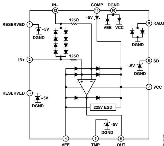
Figure 43. Simplified ESD Configuration
