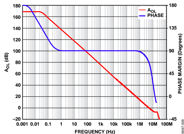
Figure 15. A_{OL} and Phase Margin vs. Frequency, T_A = 25^\circ\text{C} , V_S = \pm 110\text{ V} , R_{ADJ} = 0\ \Omega
