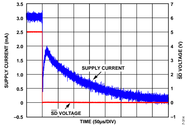
Figure 52. \overline{\text{SD}} Pin Response Time, Turning Off
