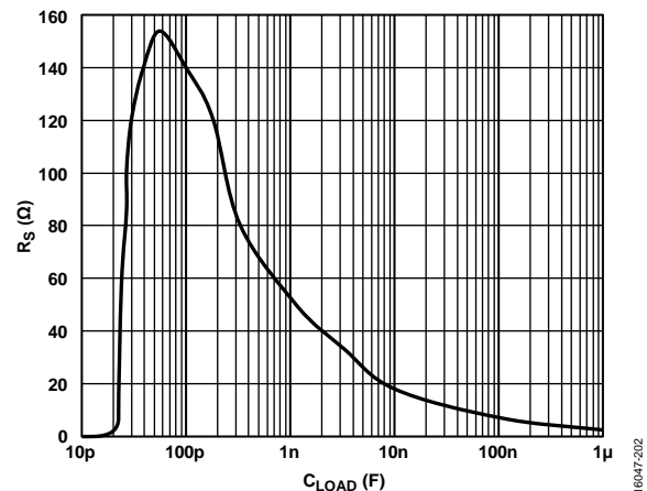
Figure 56. R_S vs. C_{LOAD} for Maximum 2 dB Peaking for Circuit from Figure 55, T_A = 25^\circ\text{C} , A_V = 1 , V_S = \pm 110\text{ V} , V_{OUT} = 100\text{ mV p-p} , R_F = 0\ \Omega , R_{ADJ} = 0\ \Omega
