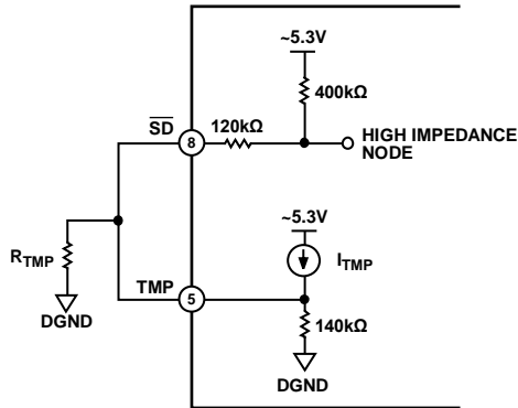
Figure 54. Tmp and \overline{SD} Pin Configuration for Short-Circuit Protection and Thermal Shutdown
