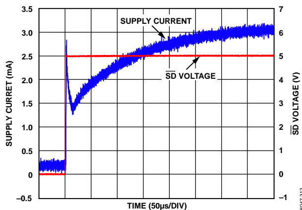
Figure 51. \overline{\text{SD}} Pin Response Time, Turning On
