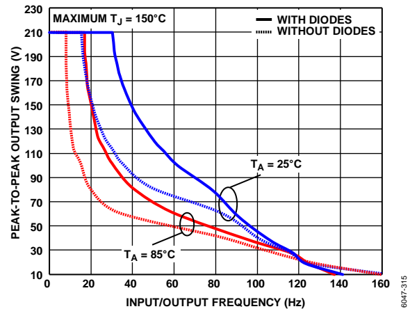
Figure 59. Dynamic SOA at T_A = 25^\circ\text{C} and T_A = 85^\circ\text{C} With and Without Input Clamping Diodes, A_V = 20 , V_S = \pm 110\text{ V} , R_F = 100\text{ k}\Omega , R_{LOAD} = 10\text{ k}\Omega , R_{ADJ} = 0\ \Omega
