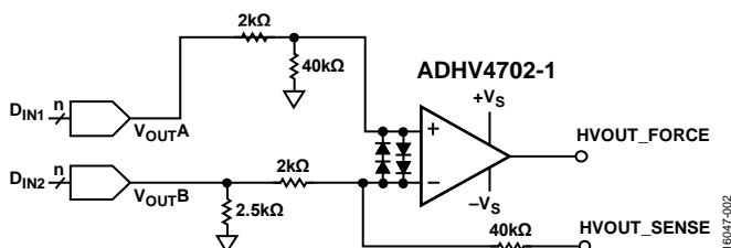
Figure 61. ADHV4702-1 Configured as a Voltage Subtractor Using DACs
