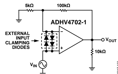
Figure 44. External Input Clamping Diodes Schematic
