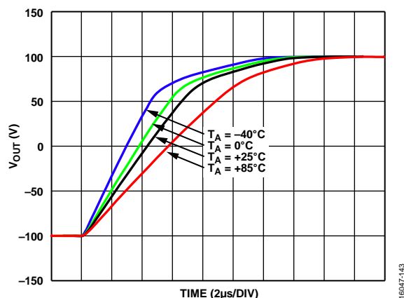
Figure 47. Large Signal Pulse Response at Various T_A with Two-Diode Forward Voltages, Rising Edge, A_V = 40 , V_S = \pm 110 V, V_{OUT} = 200 V p-p, R_F = 100 k \Omega , R_{LOAD} = 10 k \Omega , R_{ADJ} = 0 \Omega
