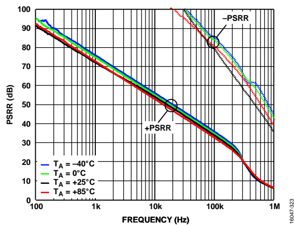
Figure 41. PSRR vs. Frequency at Various T_A , V_S = \pm 110\text{ V} , R_{\text{LOAD}} = 10\text{ k}\Omega , R_{\text{ADJ}} = 0\ \Omega
