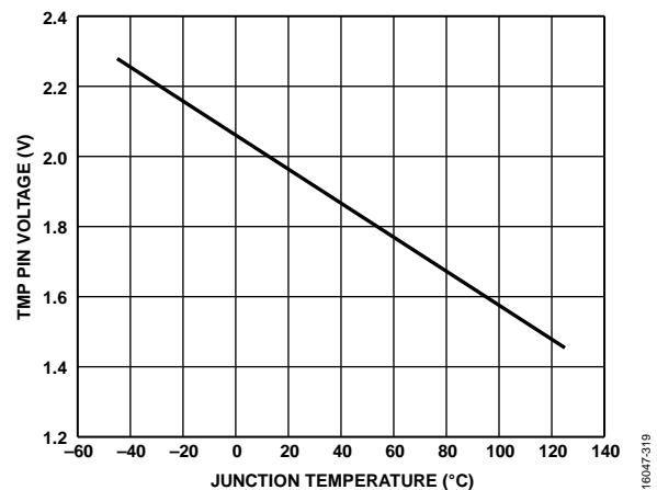
Figure 53. TMP Pin Voltage vs. Junction Temperature
