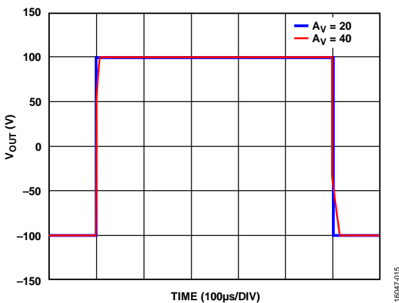
Figure 19. Large Signal Pulse Response at Various Gains, T_A = 25^\circ\text{C} , V_S = \pm 110 V, V_{OUT} = 200 V p-p, R_F = 100 k \Omega , R_{LOAD} = 10 k \Omega , R_{ADJ} = 0 \Omega
