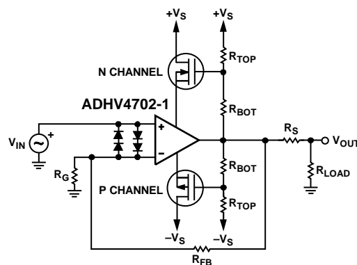
Figure 63. Voltage Extender Schematic
