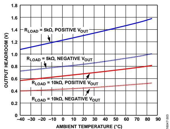
Figure 34. Output Headroom vs. Ambient Temperature at Various R_{LOAD} , V_S = \pm 110\text{ V} , R_{ADJ} = 0\ \Omega
