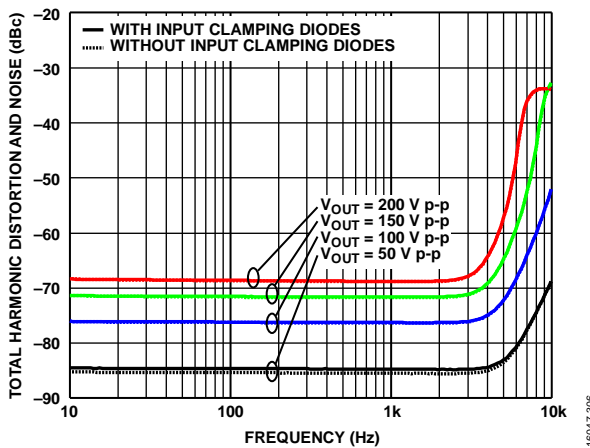
Figure 36. Total Harmonic Distortion and Noise vs. Frequency at Various Large Output Swings, T_A = 25^\circ\text{C} , A_V = 20 , V_S = \pm 110 \text{ V} , R_F = 100 \text{ k}\Omega , R_{LOAD} = 10 \text{ k}\Omega , R_{ADJ} = 0 \Omega
