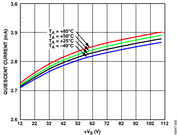
Figure 35. Quiescent Current vs. Positive Supply Voltage at Various T_A , R_{ADJ} = 0 \Omega
