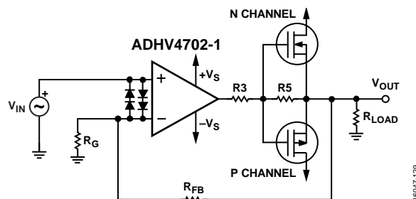
Figure 62. High Current Output Driver Schematic
