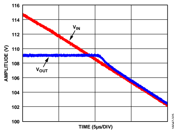
Figure 42. Output Overdrive Recovery, V_S = \pm 110\text{ V} , A_V = 40 , R_{\text{LOAD}} = 10\text{ k}\Omega , R_{\text{ADJ}} = 0\ \Omega
