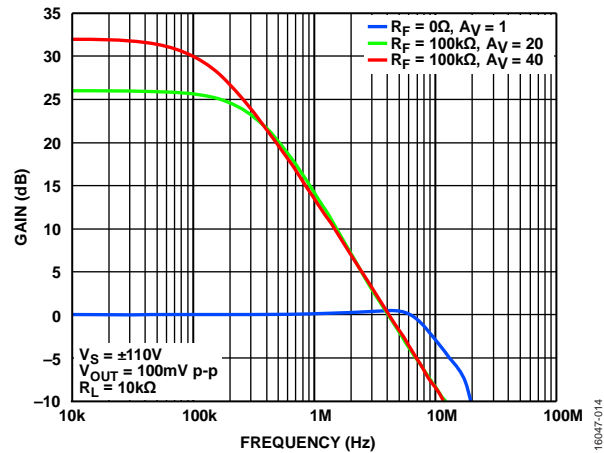
Figure 28. Small Signal Frequency Response at Various Gains, T_A = 25^\circ\text{C} , V_S = \pm 110\text{ V} , V_{OUT} = 100\text{ mV p-p} , R_L = 10\text{ k}\Omega , R_{ADJ} = 0\text{ }\Omega
