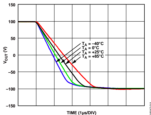
Figure 16. Large Signal Pulse Response at Various T_A , Falling Edge, A_V = 20 , V_S = \pm 110\text{ V} , V_{OUT} = 200\text{ V p-p} , R_F = 100\text{ k}\Omega , R_{LOAD} = 10\text{ k}\Omega , R_{ADJ} = 0\ \Omega
