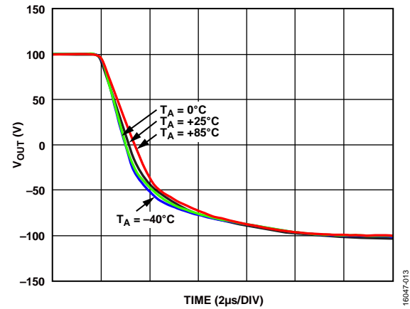
Figure 20. Large Signal Pulse Response at Various T_A , Falling Edge, A_V = 40 , V_S = \pm 110 V, V_{OUT} = 200 V p-p, R_F = 100 k \Omega , R_{LOAD} = 10 k \Omega , R_{ADJ} = 0 \Omega
