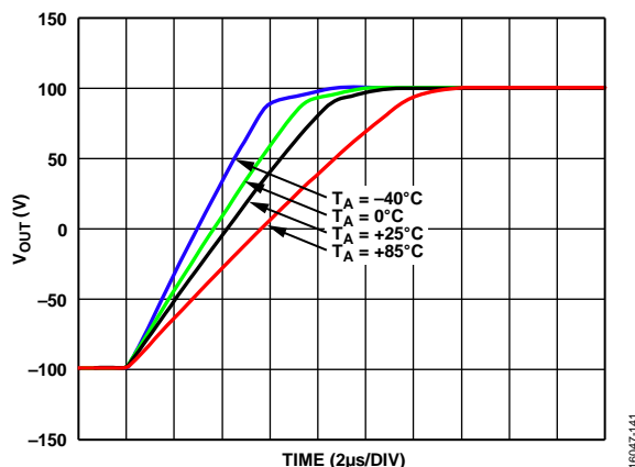
Figure 45. Large Signal Pulse Response at Various T_A with Two-Diode Forward Voltages, Rising Edge, A_V = 20 , V_S = \pm 110 V, V_{OUT} = 200 V p-p, R_F = 100 k \Omega , R_{LOAD} = 10 k \Omega , R_{ADJ} = 0 \Omega
