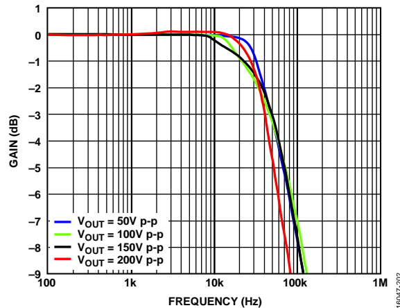
Figure 22. Large Signal Frequency Response at Various Output Swings with Input Clamping Diodes (See the Slew Boost Circuit and Protection Section), T_A = 25^\circ\text{C} , A_V = 40 , V_S = \pm 110 V, R_F = 100 k \Omega , R_{LOAD} = 10 k \Omega , R_{ADJ} = 0 \Omega
