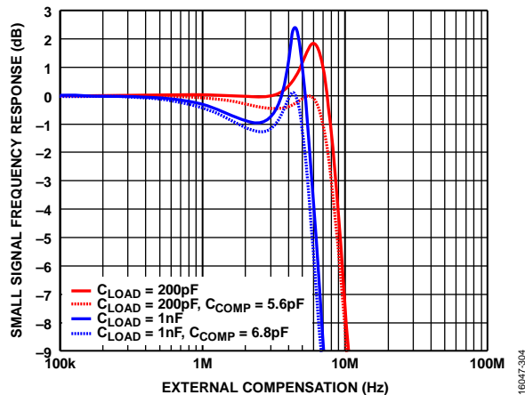
Figure 58. Small Signal Frequency Response vs. External Compensation, T_A = 25^\circ\text{C} , A_V = 1 , V_S = \pm 110\text{ V} , V_{OUT} = 100\text{ mV p-p} , R_F = 0\ \Omega , R_{ADJ} = 0\ \Omega
