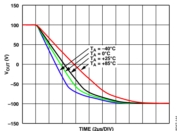
Figure 48. Large Signal Pulse Response at Various T_A with Two-Diode Forward Voltages, Falling Edge, A_V = 40 , V_S = \pm 110 V, V_{OUT} = 200 V p-p, R_F = 100 k \Omega , R_{LOAD} = 10 k \Omega , R_{ADJ} = 0 \Omega
