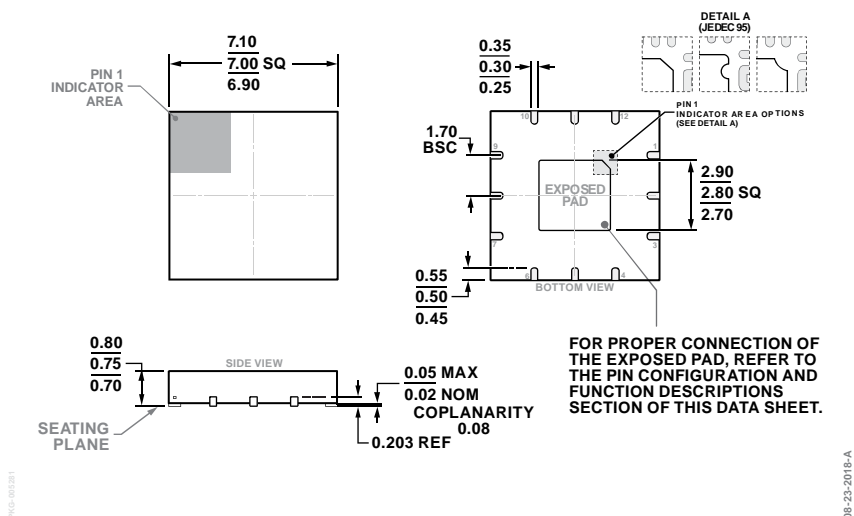
Figure 64. 12-Lead Lead Frame Chip Scale Package [LFCSP] 7 mm x 7 mm Body and 0.75 mm Package Height (CP-12-8)
