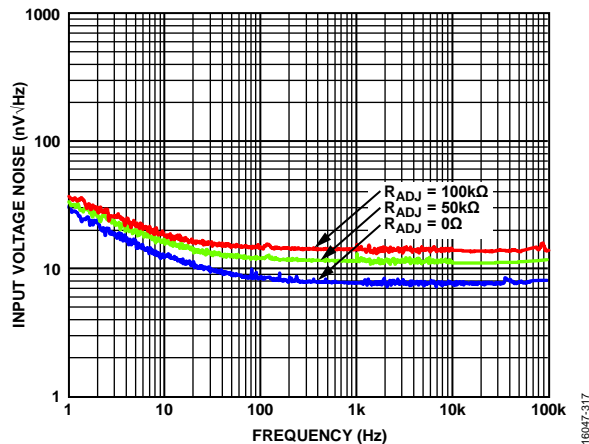
Figure 50. Input Voltage Noise at Various R_{ADJ} , T_A = 25^\circ\text{C} , V_S = \pm 110
