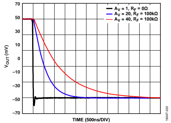
Figure 27. Small Signal Pulse Response at Various Gains, Falling Edge, T_A = 25^\circ\text{C} , V_S = \pm 110\text{ V} , V_{OUT} = 100\text{ mV p-p} , R_{LOAD} = 10\text{ k}\Omega , R_{ADJ} = 0\text{ }\Omega
