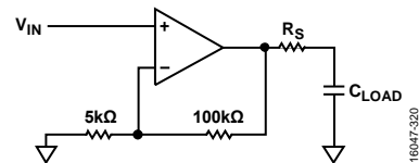
Figure 55. Circuit for C_{LOAD} Drive
