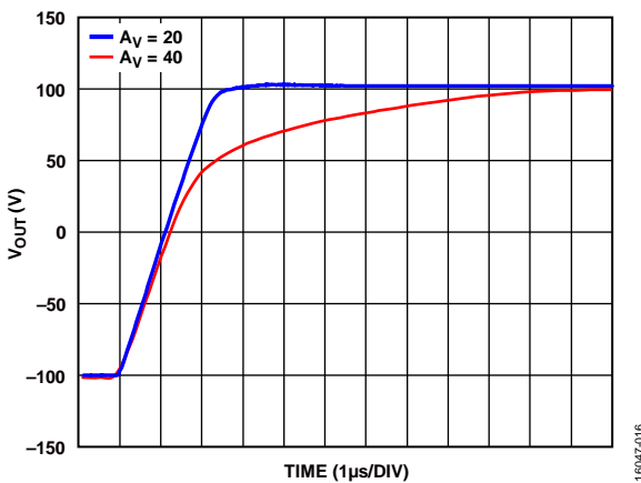
Figure 18. Large Signal Pulse Response at Various Gains, Rising Edge, T_A = 25^\circ\text{C} , V_S = \pm 110 V, V_{OUT} = 200 V p-p, R_F = 100 k \Omega , R_{LOAD} = 10 k \Omega , R_{ADJ} = 0 \Omega
