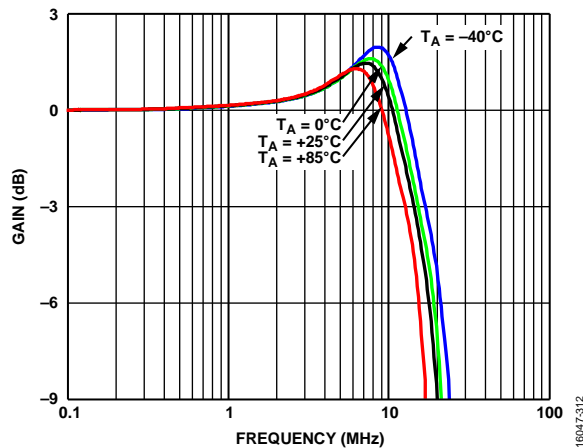
Figure 25. Small Signal Frequency Response at Various T_A , A_V = 1 , V_S = \pm 110\text{ V} , V_{OUT} = 100\text{ mV p-p} , R_L = 10\text{ k}\Omega , R_{ADJ} = 0\text{ }\Omega
