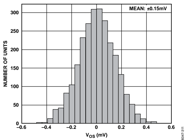
Figure 11. Input Offset Voltage Distribution, T_A = 25^\circ\text{C} , V_S = \pm 110\text{ V} , V_{CM} = 0\text{ V} , R_{ADJ} = 0\ \Omega
