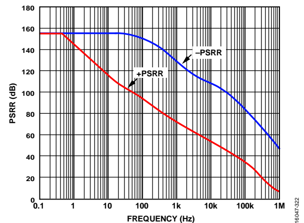
Figure 40. PSRR vs. Frequency, T_A = 25^\circ\text{C} , V_S = \pm 110 \text{ V} , R_{LOAD} = 10 \text{ k}\Omega , R_{ADJ} = 0 \Omega
