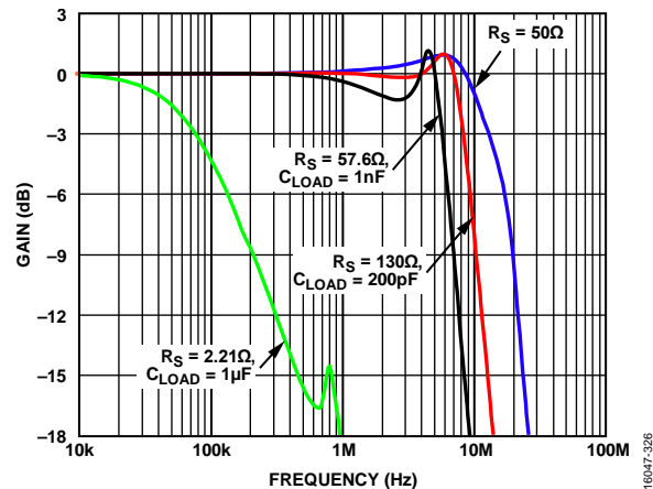
Figure 57. Small Signal Response for Various C_{LOAD} and R_S Values, T_A = 25^\circ\text{C} , A_V = 1 , V_S = \pm 110\text{ V} , V_{OUT} = 100\text{ mV p-p} , R_F = 0\ \Omega , R_{ADJ} = 0\ \Omega
