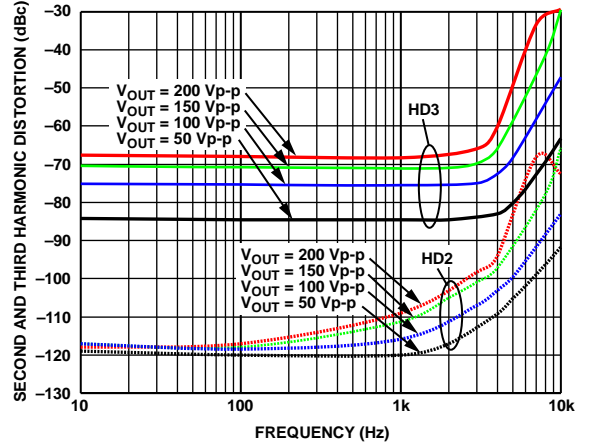
Figure 39. Second Harmonic Distortion (HD2) and Third Harmonic Distortion (HD3) vs. Frequency at Various Output Swings, T_A = 25^\circ\text{C} , A_V = 40 , V_S = \pm 110 \text{ V} , R_F = 100 \text{ k}\Omega , R_{LOAD} = 10 \text{ k}\Omega , R_{ADJ} = 0 \Omega
