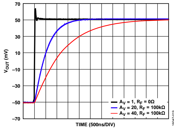
Figure 24. Small Signal Pulse Response at Various Gains, Rising Edge, T_A = 25^\circ\text{C} , V_S = \pm 110\text{ V} , V_{OUT} = 100\text{ mV p-p} , R_{LOAD} = 10\text{ k}\Omega , R_{ADJ} = 0\text{ }\Omega
