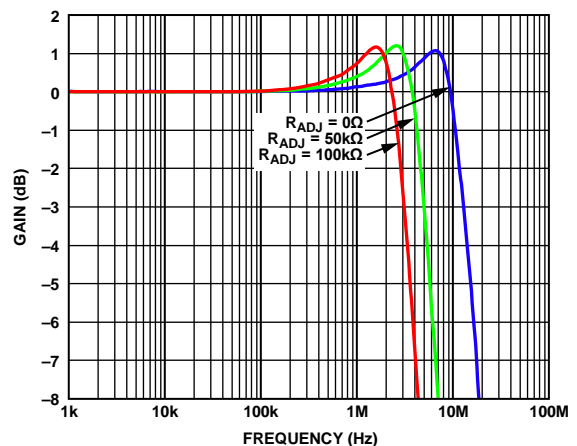
Figure 49. Small Signal Frequency Response at Various R_{ADJ} , T_A = 25^\circ\text{C} , A_V = 1 , V_S = \pm 110 V, V_{OUT} = 100 mV p-p, R_F = 0 \Omega , R_{LOAD} = 10 k \Omega
