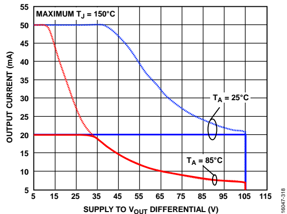
Figure 60. DC SOA at T_A = 25^\circ\text{C} and T_A = 85^\circ\text{C} , A_V = 20 , V_S = \pm 110\text{ V} , R_F = 100\text{ k}\Omega , R_{ADJ} = 0\ \Omega
