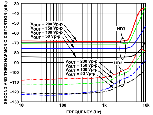
Figure 38. Second Harmonic Distortion (HD2) and Third Harmonic Distortion (HD3) vs. Frequency at Various Output Swings, T_A = 25^\circ\text{C} , A_V = 20 , V_S = \pm 110 \text{ V} , R_F = 100 \text{ k}\Omega , R_{LOAD} = 10 \text{ k}\Omega , R_{ADJ} = 0 \Omega
