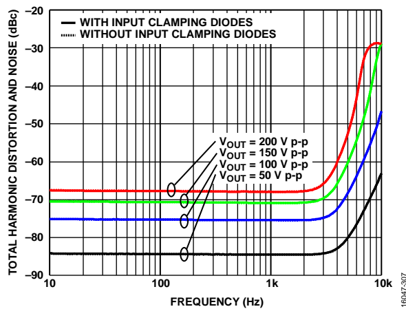
Figure 37. Total Harmonic Distortion and Noise vs. Frequency at Various Large Output Swings, T_A = 25^\circ\text{C} , A_V = 40 , V_S = \pm 110 \text{ V} , R_F = 100 \text{ k}\Omega , R_{LOAD} = 10 \text{ k}\Omega , R_{ADJ} = 0 \Omega
