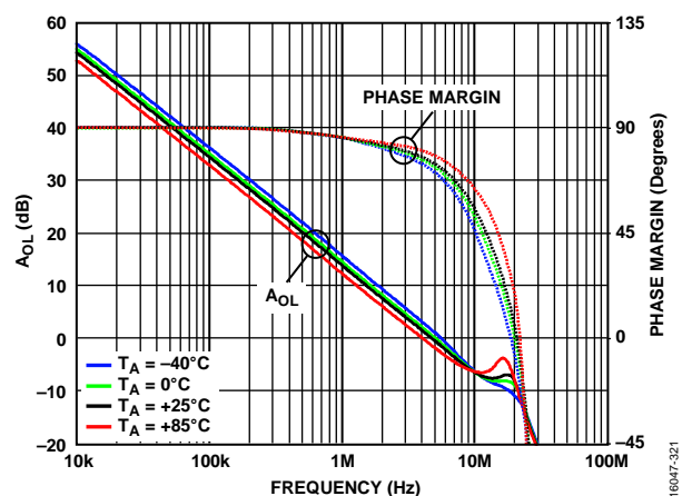
Figure 14. A_{OL} and Phase Margin vs. Frequency at Various T_A , V_S = \pm 110\text{ V} , R_{ADJ} = 0\ \Omega
