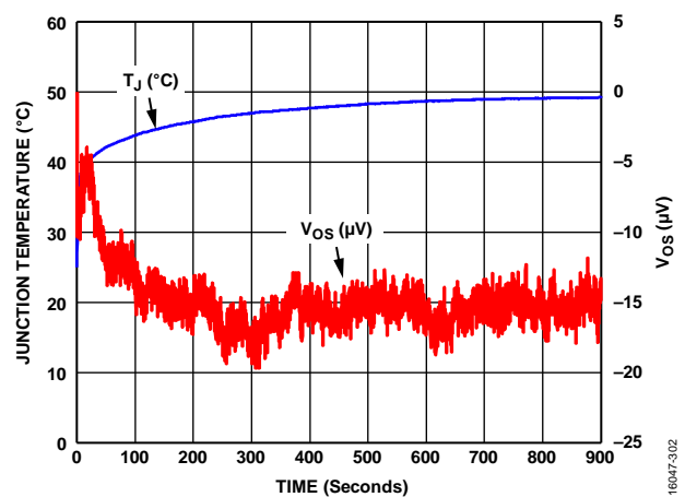
Figure 33. Offset Voltage Warmup Drift and T_J , V_S = \pm 110 , R_{ADJ} = 0\ \Omega
