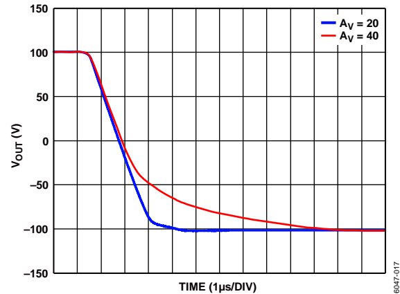
Figure 21. Large Signal Pulse Response at Various Gains, Falling Edge, T_A = 25^\circ\text{C} , V_S = \pm 110 V, V_{OUT} = 200 V p-p, R_F = 100 k \Omega , R_{LOAD} = 10 k \Omega , R_{ADJ} = 0 \Omega
