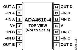
Figure 6. ADA4610-4 Pin Configuration, 14-Lead SOIC_N (R Suffix)
