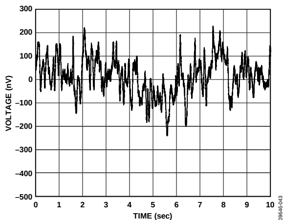
Figure 47. Voltage Noise, 0.1 Hz to 10 Hz
