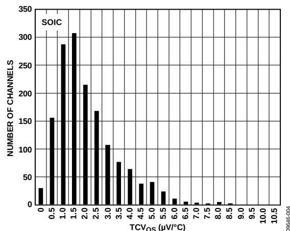
Figure 8. Input Offset Voltage Drift ( TCV_{OS} ) Distribution, V_{SY} = \pm 5\text{ V}
