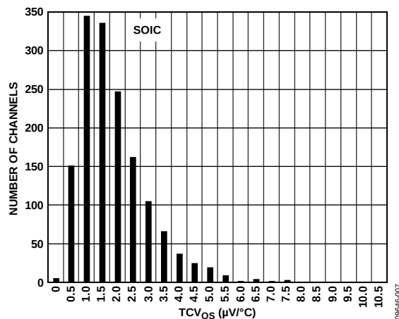
Figure 11. TCV_{OS} Distribution, V_{SY} = \pm 15\text{ V}
