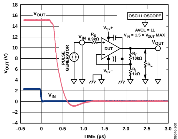
Figure 49. Positive Overload Recovery
