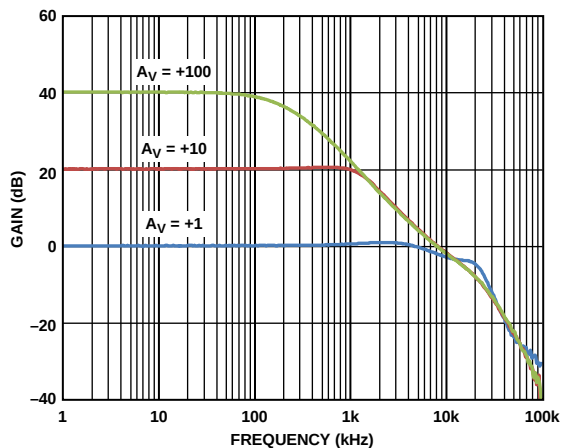
Figure 25. Closed-Loop Gain vs. Frequency, V_{SV} = \pm 5\text{ V}
