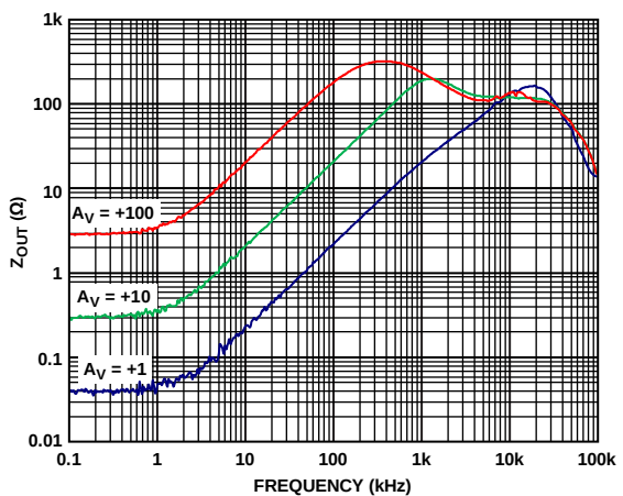
Figure 26. Closed-Loop Output Impedance ( Z_{OUT} ) vs. Frequency, V_{SV} = \pm 5\text{ V}
