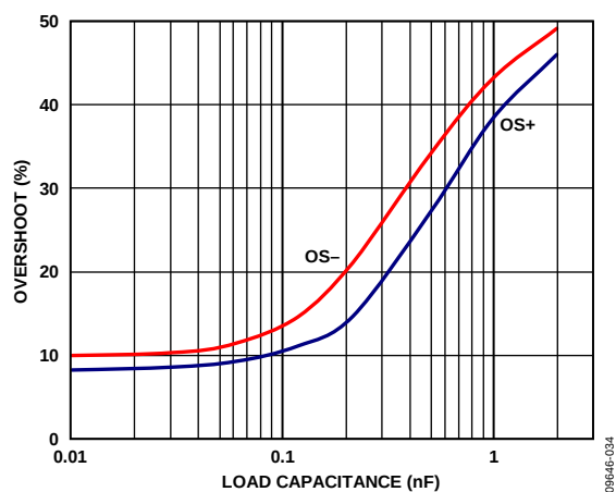
Figure 38. Overshoot vs. Load Capacitance, V_{SY} = \pm 5\text{ V} , A_V = +1 , R_L = 2\text{ k}\Omega , V_{IN} = 100\text{ mV p-p}
