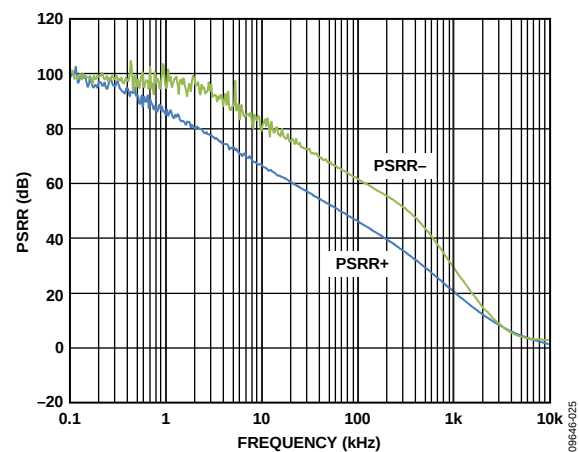
Figure 30. PSRR vs. Frequency, V_{SV} = \pm 15\text{ V}
