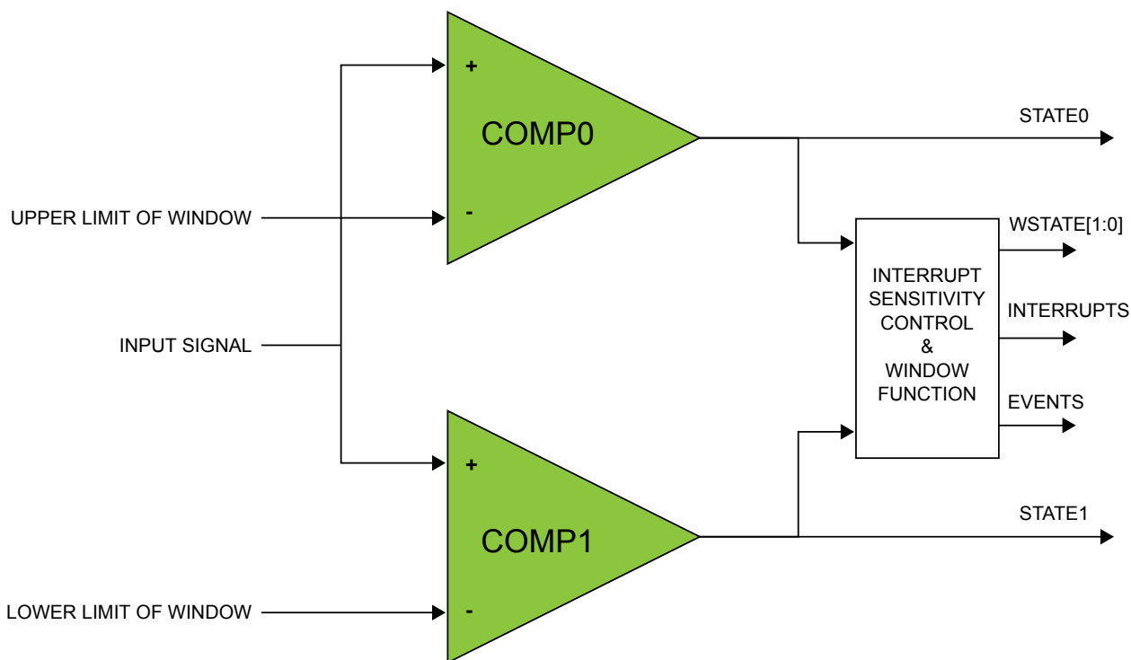
Figure 42-4. Comparators in Window Mode
