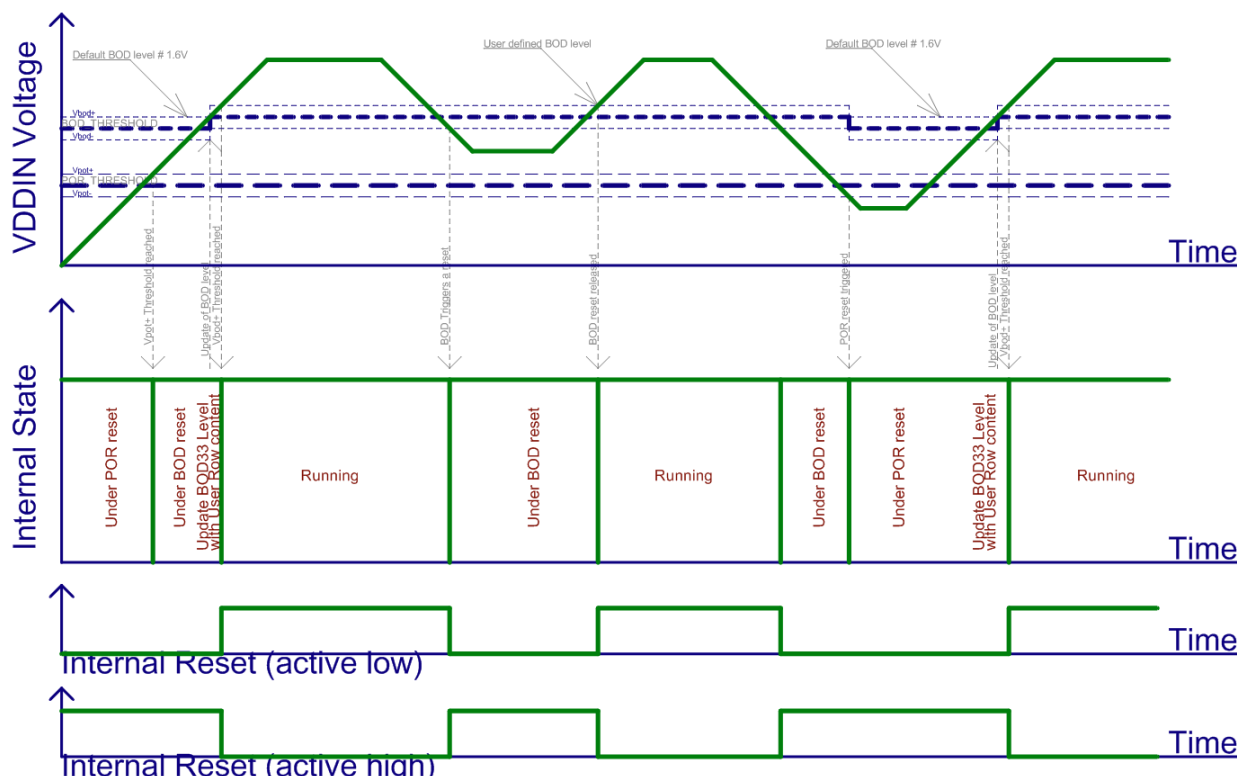
Figure 45-1. BOD Reset Behavior at Startup and Default Levels
