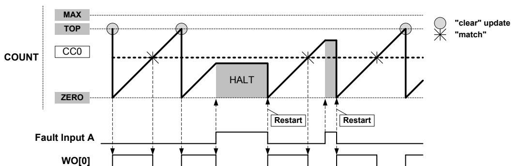
Figure 36-28. Waveform Generation with Halt and Restart Actions
