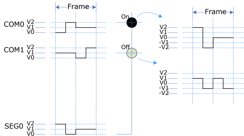
Figure 43-7. 1/2 bias, 1/2 Duty Standard Waveform
