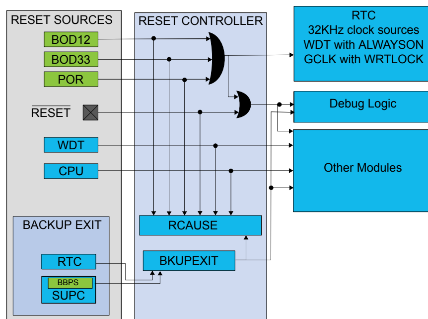
Figure 19-1. Reset System
