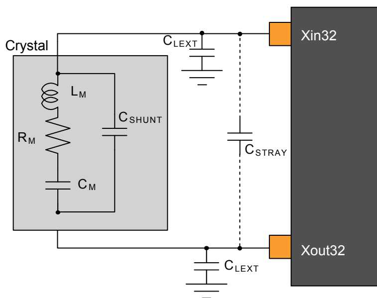
Figure 45-3. Oscillator Connection
