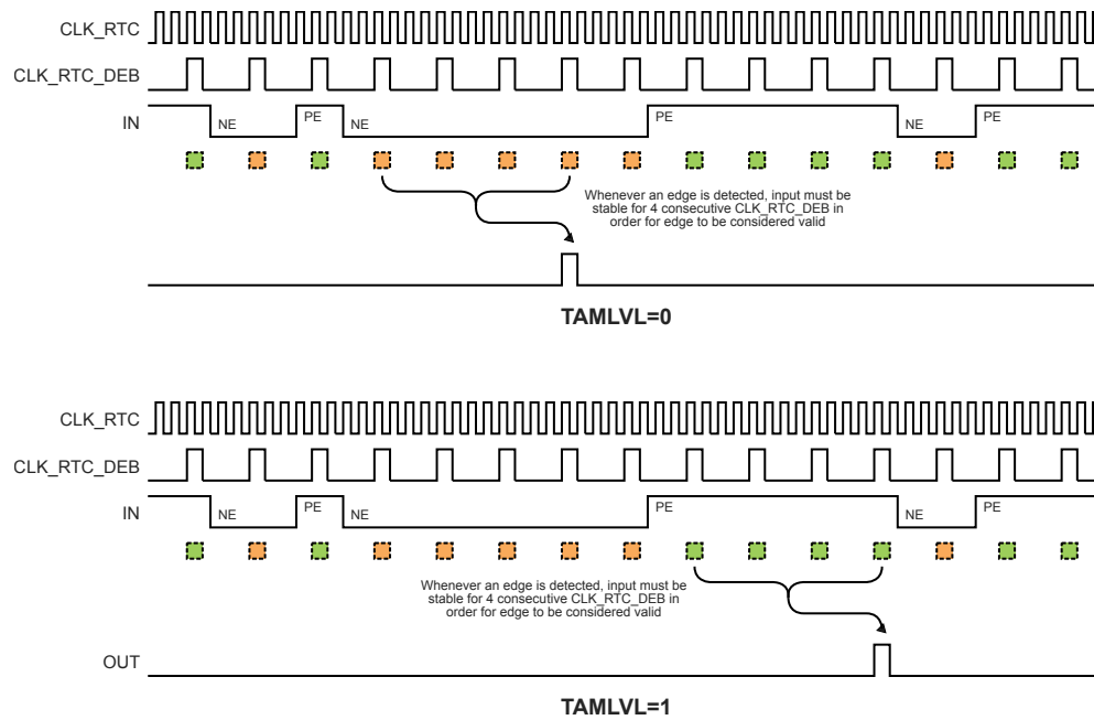
Figure 25-8. Edge Detection with Asynchronous Stability Debouncing
