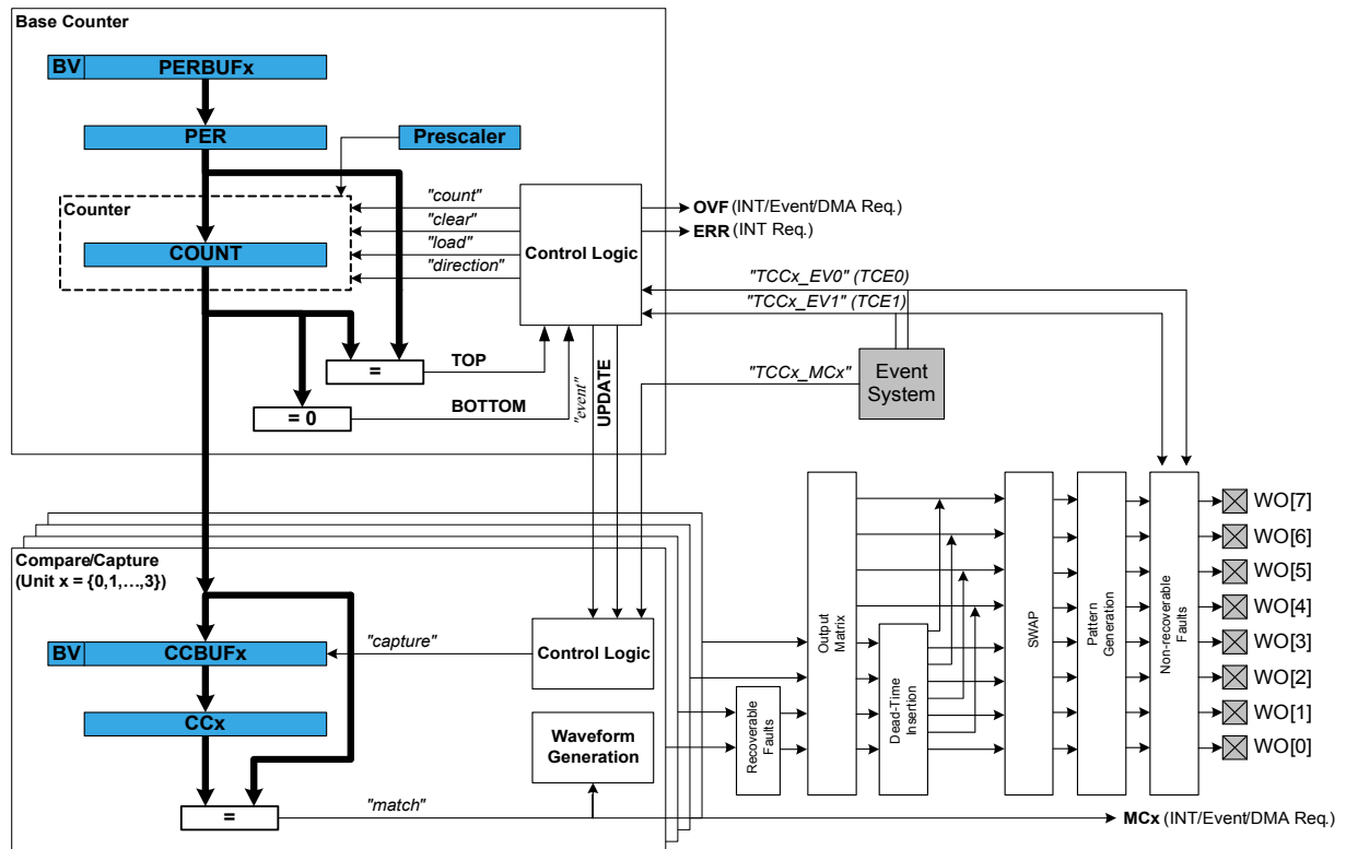
Figure 36-1. Timer/Counter for Control Applications - Block Diagram
