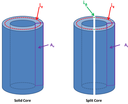
Figure 4: Solid core versus split core configurations.
