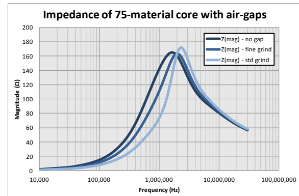
Figure 6: Calculated impedance for three different air gaps.
