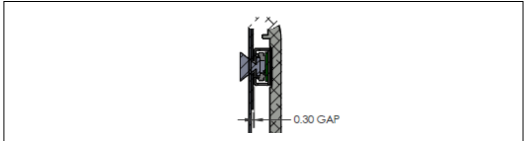
Figure 7-13. Stereo Depth Module Air Gap
