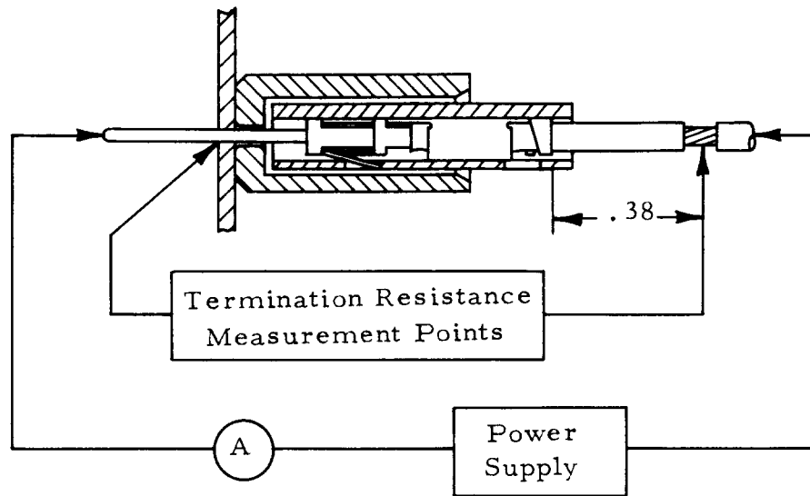
Receptacle Mated To Header
