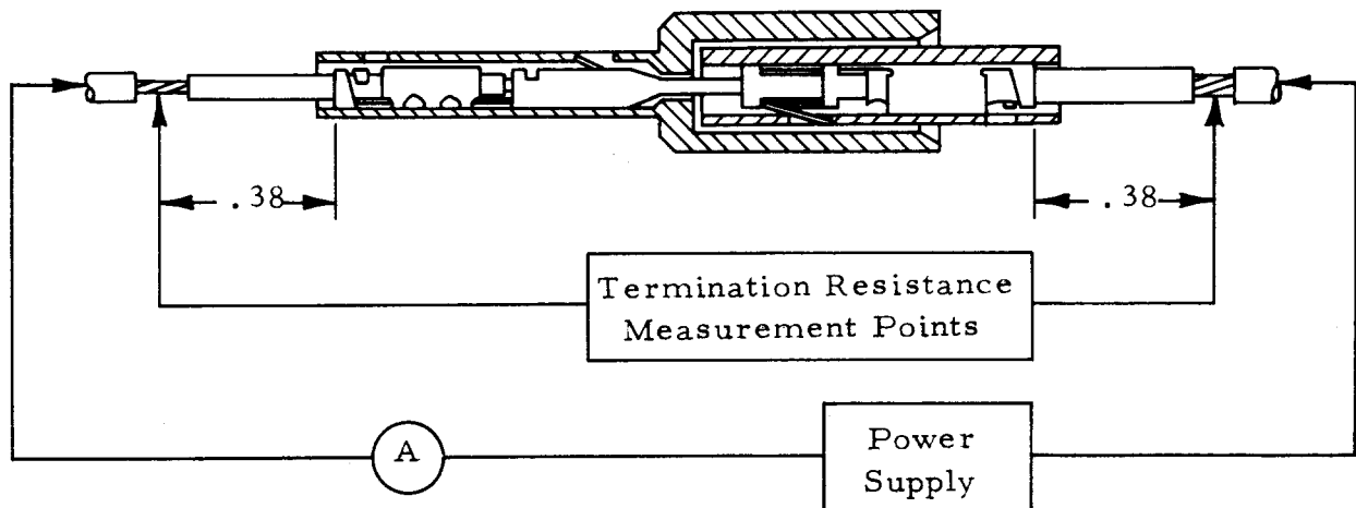
Receptacle Mated To Pin Contact
