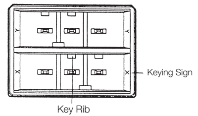
XY-Type
