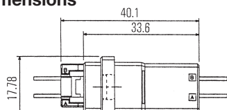
Panel/Free-Hanging Type
