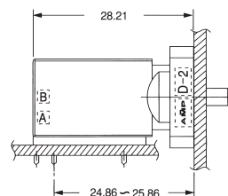
Drawer Type
