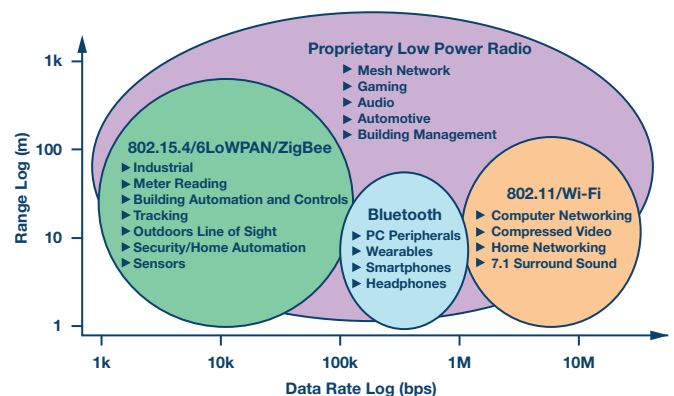
Figure 1. Short-range wireless connections.
