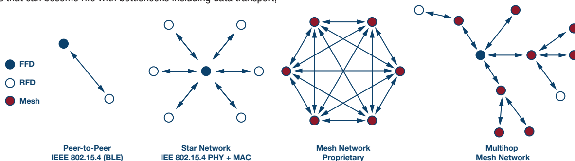
Figure 4. Network models: peer-to-peer, star, mesh, and multihop topology
