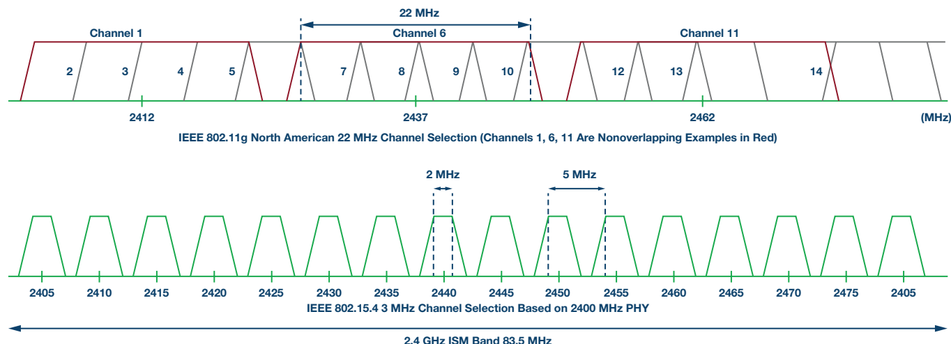
Figure 3. Worldwide IEEE 802.15.4 PHY, Channel 11 through Channel 26 and IEEE 802.11g, Channel 1 through Channel 14.
