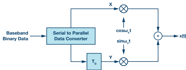
Figure 6. Offset QPSK modulator architecture.
