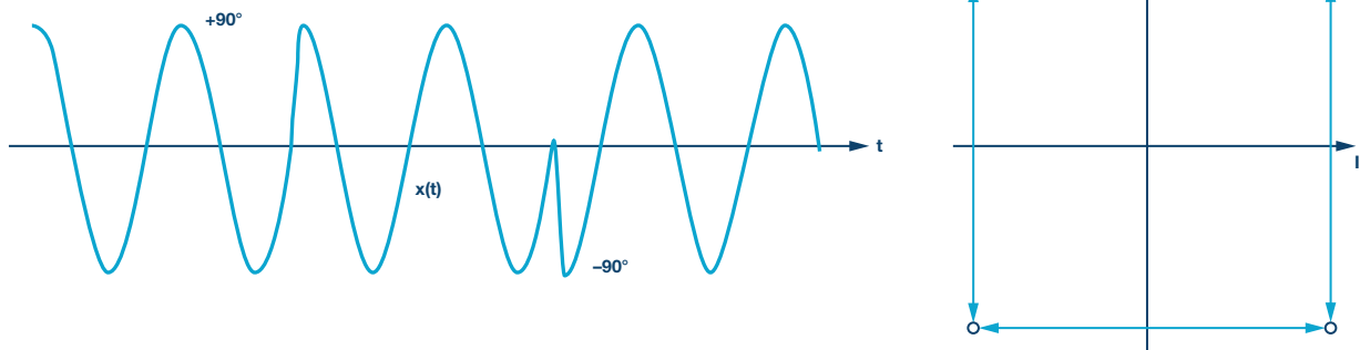
Figure 7. Phase transition \pm 90^\circ (left) with I/Q O-QPSK options (right).
