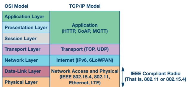
Figure 2. OSI and TCP/IP models.
