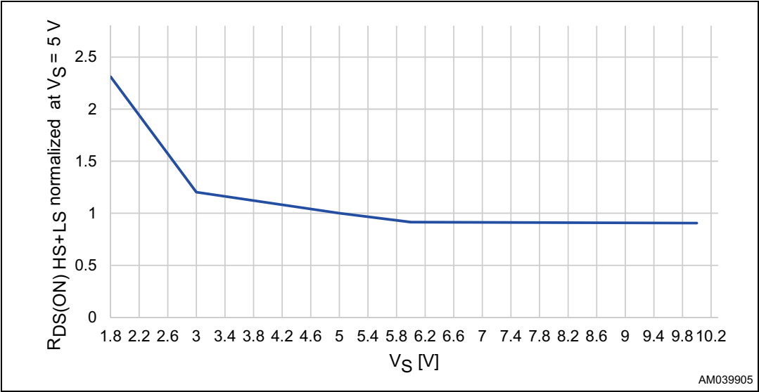
Figure 12. Power stage resistance versus supply voltage (normalized at V_S = 5\text{ V} )
