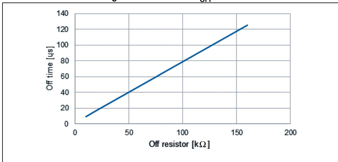
Figure 7. OFF time vs. R_{\text{OFF}} value
